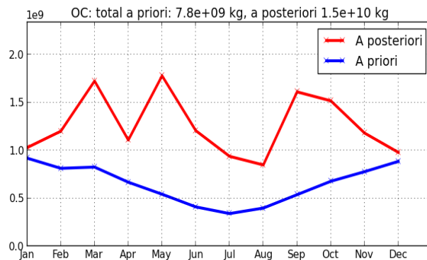
Figure 11. Monthly emissions of OC in Asia, total 2008, unit = \text{Mt PM month}^{-1} .
