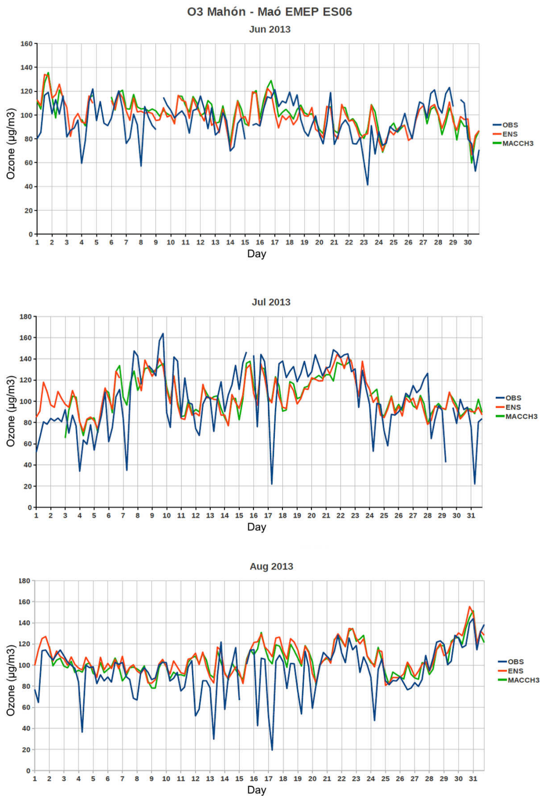
Figure 11. As Fig. 10 but for Mahón ( 39.867^{\circ} N, 4.32^{\circ} W).
