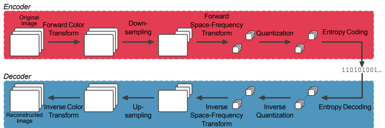
Figure 1: Schematic of a typical encoding and decoding process in lossy image compression, such as JPEG (ITU 1992). The input image is first converted from the original color space (e.g., RGB) to a representation reducing correlation between color bands (e.g., YCbCr (ITU 1995)). Each color component, possibly after some down-sampling, is split into independent coding units (e.g., blocks of 8 \times 8 pixels). Space-frequency transformation permits not only spatial decorrelation but identifies information to be selectively discarded through quantization. The transformed and quantized coefficients are further compressed by an entropy coding stage using lossless approaches. This results in a bitstream arranged according to a predetermined syntax, that can be decoded performing all previous operations in reverse order, to obtain an approximation of the original image.
