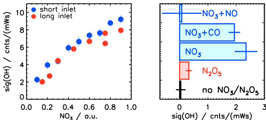
Figure 9. OH signals, if air containing \text{NO}_3 produced from thermal decomposition of frozen \text{N}_2\text{O}_5 is sampled for two designs of the OH fluorescence cell. Left panel: Variation of \text{NO}_3 concentration by changing the air flow through the \text{N}_2\text{O}_5 source. Right panel: No OH signal (cell with the short inlet) is seen without flow from the \text{N}_2\text{O}_5 source, only a small signal is observed if \text{N}_2\text{O}_5 is not actively heated downstream of the source (small efficiency of \text{N}_2\text{O}_5 dissociation), the large signal observed, if \text{N}_2\text{O}_5 is sampled through an heated inlet (high efficiency of \text{N}_2\text{O}_5 dissociation). The signal remains, if CO is added to scavenge OH, but disappears, if NO is added to scavenge \text{NO}_3 .
