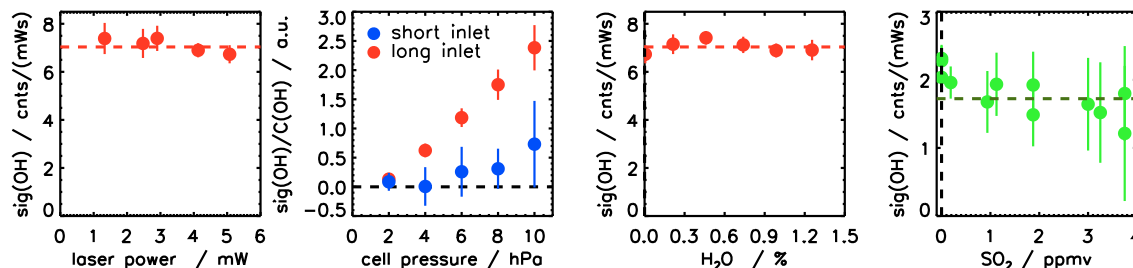
Figure 6. OH signals from limonene or \alpha -pinene ozonolysis depending on various parameters: laser power (1 ppmv \alpha -pinene, 110 ppbv \text{O}_3 , cell with short inlet), cell pressure (45 ppbv limonene, 350 ppbv \text{O}_3 , 1000 ppmv propane), water vapor (1 ppmv \alpha -pinene, 110 ppbv \text{O}_3 , cell with short inlet), \text{SO}_2 (40 ppbv limonene, 550 ppbv \text{O}_3 , 400 ppmv propane, cell with long inlet). No propane was added for testing the laser power and water vapor dependencies. In these two cases, the concentration of \alpha -pinene was chosen to be high enough, such that the OH signal was dominated by internally produced OH in the detection cell.
