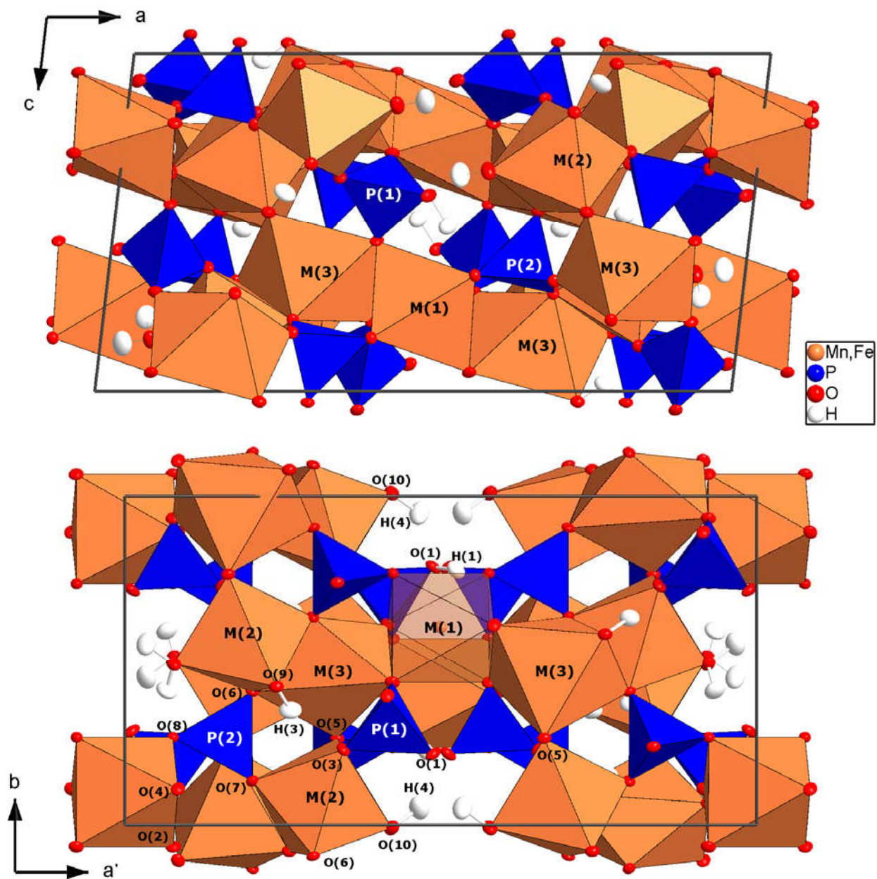
Figure 1. Two views of the crystal structure of hureaulite based on the neutron structure refinement (at 293 K) of this study. Displacement ellipsoid probability factor: 50%.
