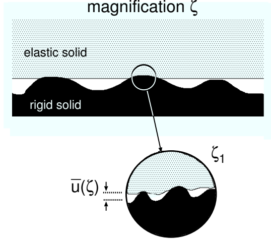
FIG. 4: An asperity contact region observed at the magnification \zeta . It appears that complete contact occurs in the asperity contact region, but upon increasing the magnification to the highest resolution (magnification \zeta_1 ) it is observed that the solids are separated by the (average) distance \bar{u}(\zeta) .
