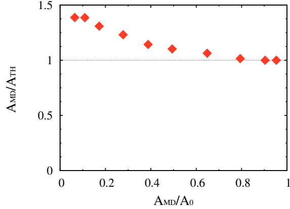
FIG. 9: Projected contact area comparison between molecular dynamics simulations A_{MD} and continuum mechanics theory of Persson A_{TH} . At small squeezing pressure, A_{MD} is about (30 – 38)% bigger than the A_{TH} . However, the difference decreases with increasing pressure.
