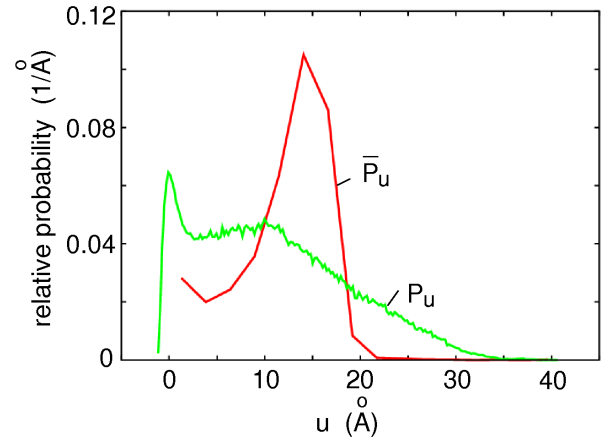
FIG. 21: The probability distributions P_u and \bar{P}_u are defined in the text. For the surface shown in Fig. 3 and for the squeezing pressure 1.3 GPa. The distribution \bar{P}_u has a delta function at u = 0 with the weight A(\zeta_1)/A_0 \approx 0.047 .
