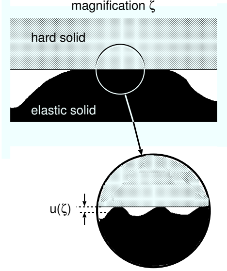
FIG. 17: An asperity contact region observed at the magnification \zeta . It appears that complete contact occurs in the asperity contact region, but upon increasing the magnification it is observed that the solids are separated by the average distance \bar{u}(\zeta) .
