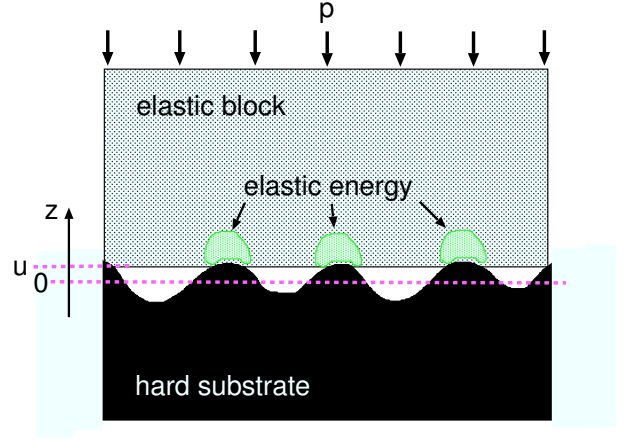
FIG. 2: An elastic block squeezed against a rigid rough substrate. The separation between the average plane of the substrate and the average plane of the lower surface of the block is denoted by u . Elastic energy is stored in the block in the vicinity of the asperity contact regions.
