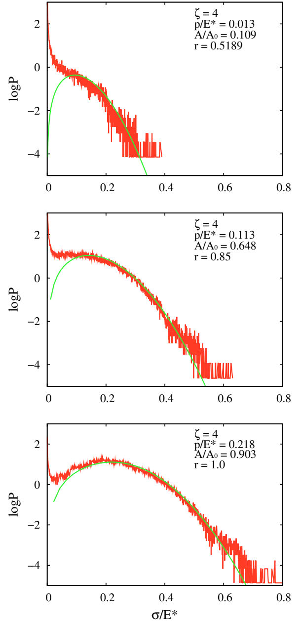
FIG. 7: The pressure distribution for \zeta = 4 for three different nominal pressure. The analytical theory has been used to fit the numerical pressure distribution as good as possible. Note r = \tilde{G}/G (see Ref.[13]).
