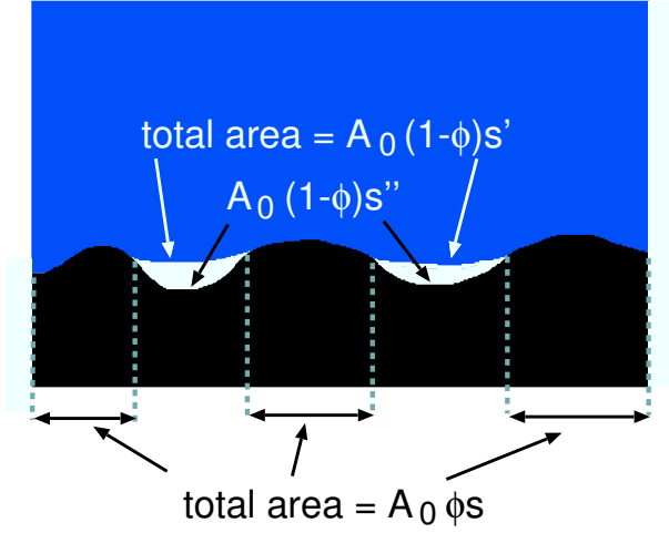
FIG. 5: The interface between liquid and solid. \phi < 1 is the ratio between the projected liquid-solid contact area and the nominal (or apparent) contact area A_0 . Because the solid surface is curved, the actual liquid-solid contact area will be A_0\phi s where s > 1 . Similarly, since in general the liquid-vapor interface is curved (in spite of the fact that the total curvature 1/R_1 + 1/R_2 may vanish) and tilted (relative to the average surface plane) the total liquid-vapor interface area is A_0(1-\phi)s' , with s' > 1 . Similarly, the solid-vapor interface area equals A_0(1-\phi)s'' with s'' > 1 .
