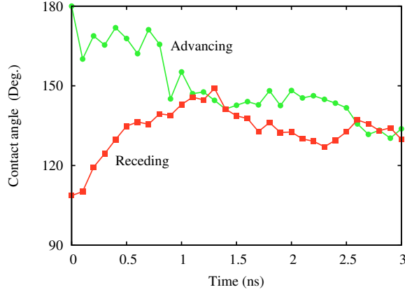
FIG. 19: The advancing (circles) and receding (squares) contact angle \theta , for hydrophobic substrate, as a function of time. The root-mean-square roughness of the substrate is \text{rms} = 4.8 Å. \epsilon = 4 meV and r_0 = 3.28 Å. The thermal equilibrium contact angle has been reached after a few nanoseconds, irrespective of whether the initial contact angle is larger or smaller than the equilibrium angle.
