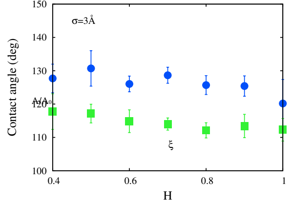
FIG. 14: The contact angle \theta as a function of Hurst exponent H for the rms roughness \sigma = 3 \text{ Å} . The circles and squares have the same meaning as that in Fig. 13. The fractal dimension is D_f = 3 - H . Adapted from Ref. [11].
