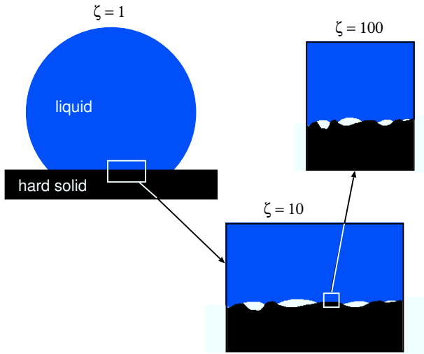
FIG. 4: Liquid droplet on a rough substrate. At the lowest magnification \zeta the surface appears flat and the liquid contact angle is \theta_0 . At increasing magnification surface roughness is observed and the liquid will in general only make contact with the substrate in some asperity contact regions.
