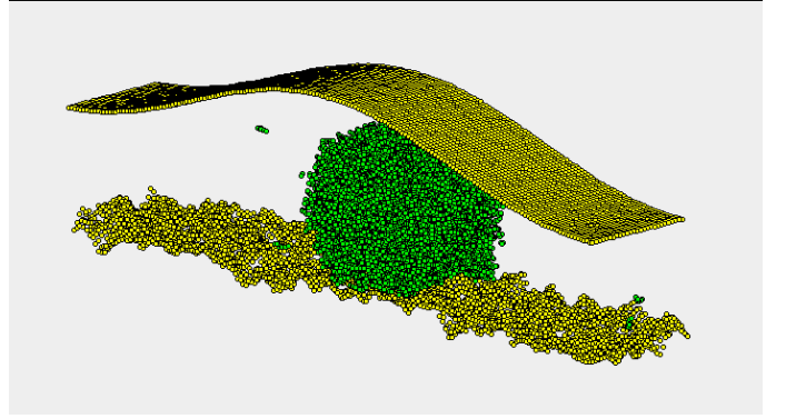
FIG. 9: 3D side-view snapshot of an octane liquid droplet on a hydrophobic and rough substrate. The rigid substrate comprises 200 \times 30 atoms disposed on a square lattice with lattice constant a = 2.53 Å. These atoms have been randomly displaced along the z coordinate, orthogonal to the wall, so to reproduce the desired roughness. The Lennard-Jones solid-liquid interaction potential V(r) = 4\epsilon[(r_0/r)^{12} - (r_0/r)^6] with r_0 = 3.28 Å, \epsilon = 4 meV for hydrophobic substrate and \epsilon = 8 meV for hydrophilic substrate.
