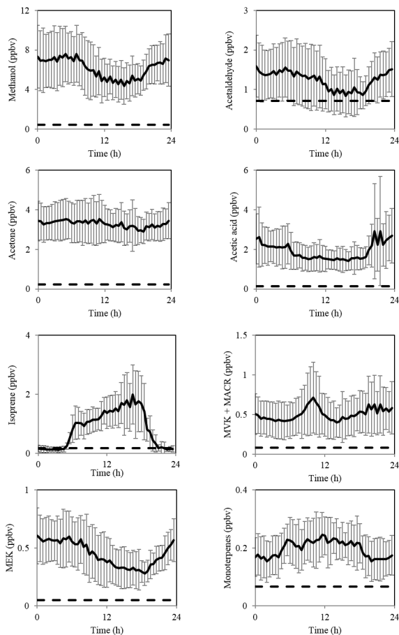
Figure 3. Mean 4 m above-canopy diurnal volume mixing ratios of volatile organic compounds measured during the Bosco Fontana field campaign. Error bars represent one standard deviation from the mean and the dashed line denotes limit of detection.
