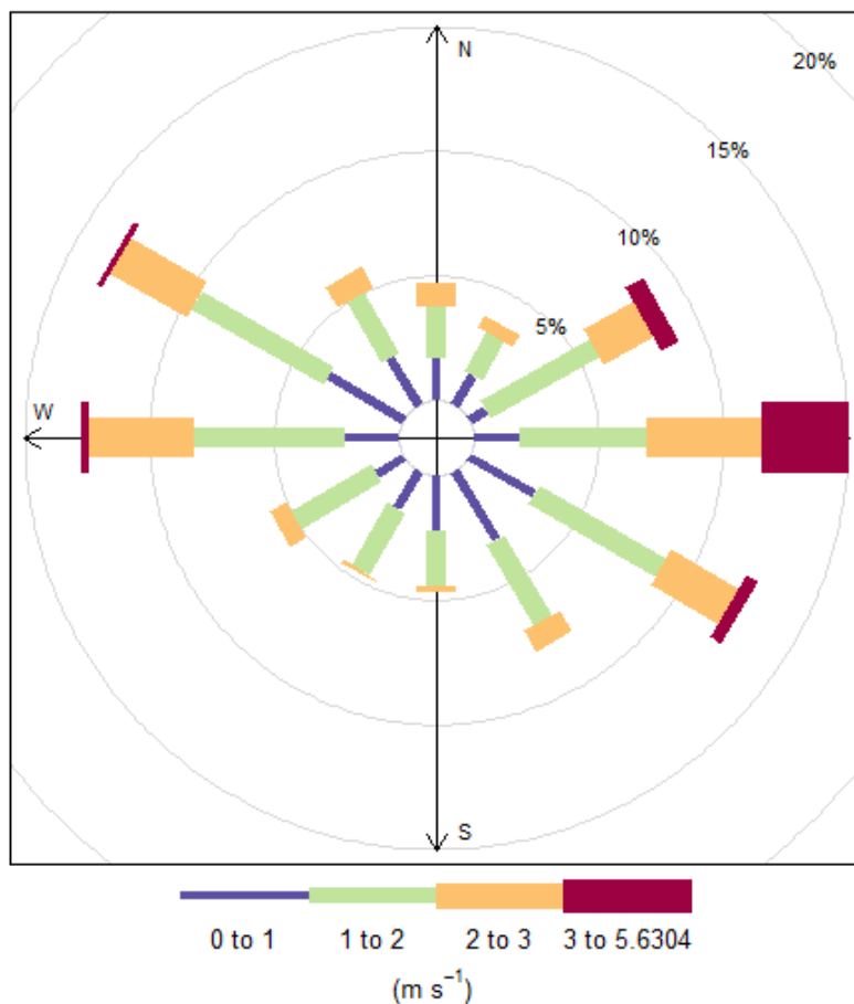
Figure 2. Wind direction and wind speed observed during the Bosco Fontana field campaign.
