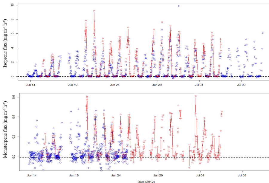
Figure 4. Time series of isoprene (top) and monoterpene (bottom) fluxes ( \text{mg m}^{-2} \text{h}^{-1} ) measured using the method of vDEC. Blue circles, triangles and diamonds represent 25 min averaged flux data from the PTR-MS which respectively passed all tests, fell below the u_* threshold or the LoD. Red circles and lines represent PTR-ToF-MS isoprene and monoterpene fluxes with 30 min averaged flux files failing the stationarity test removed.
