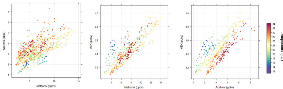
Figure 7. Scatter plots displaying the relationship between the volume mixing ratios of methanol, acetone and MEK measured 4 m above the canopy, coloured by temperature.
