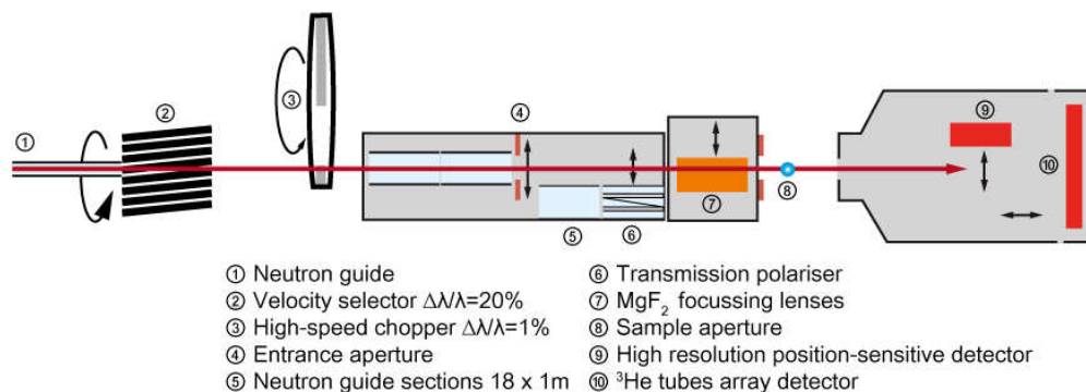
Figure 2: Schematic drawing of KWS-2.
