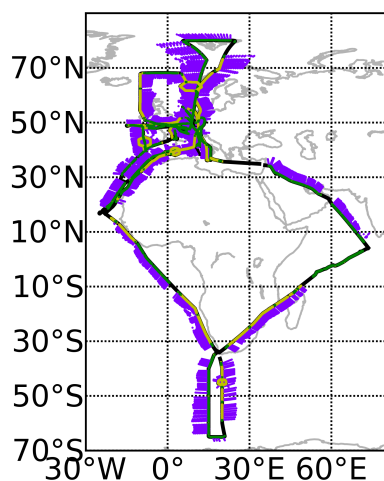
Figure 1. Overview over the flights performed during TACTS and ESMVAL. The flight paths are marked as black lines. Atmosphere measurements of GLORIA are overlayed in dark and light green for chemistry and dynamics mode, respectively. The tangent points of preliminarily processed profiles are shown in blue.
