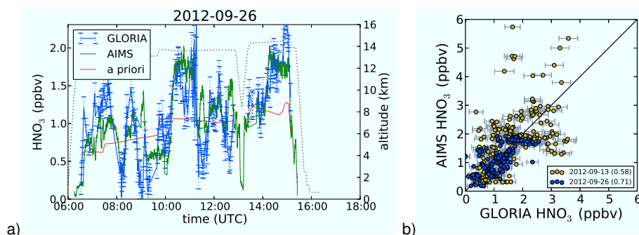
Figure 10. Comparison of retrieved \text{HNO}_3 125 m below flight level and \text{HNO}_3 measured by AIMS. See also Fig. 7 and Table 5. On 23 September 2012, AIMS has been operated in the water vapour mode; therefore no \text{HNO}_3 data are available for that flight.
