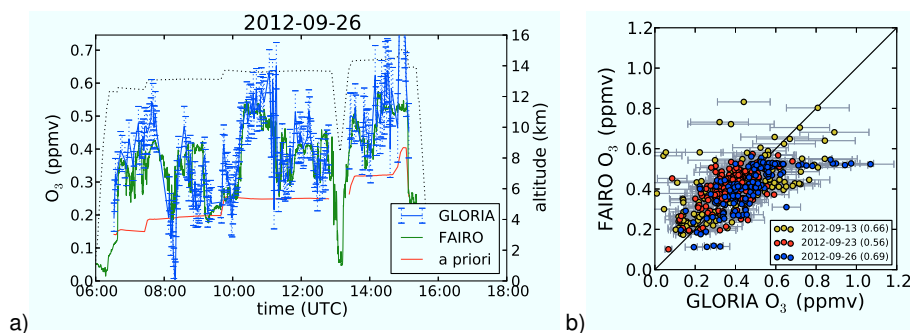
Figure 9. Comparison of retrieved \text{O}_3 125 m below flight level and \text{O}_3 measured by FAIRO. See also Fig. 7 and Table 5.
