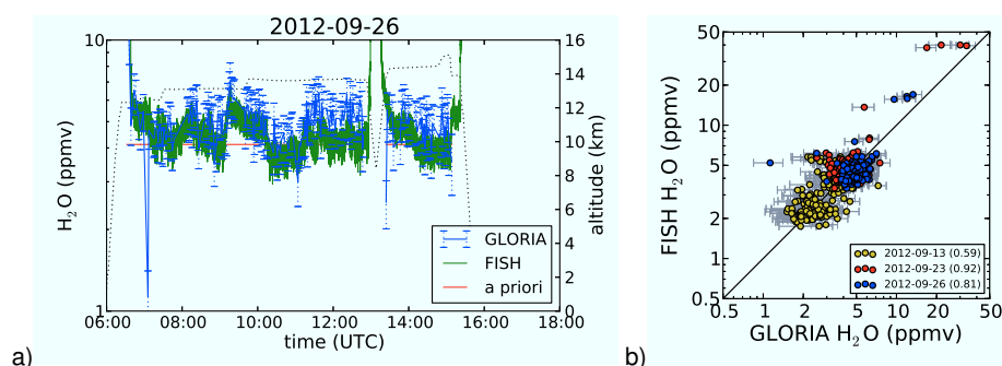
Figure 8. Comparison of retrieved \text{H}_2\text{O} 125 m below flight level and \text{H}_2\text{O} measured by FISH. See also Fig. 7 and Table 5.
