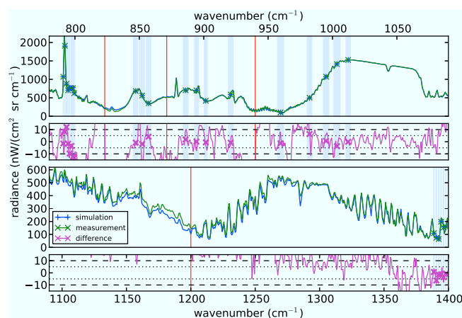
Figure 3. A measured and a simulated dynamics mode spectrum averaged over row 57 (tangent altitude 12.78\text{ km} ) of the detector taken at 14:40:12 UTC and 14.45\text{ km} aircraft altitude. The spectrum is split at 1090\text{ cm}^{-1} with the lower panels showing higher wavenumbers. The lines show the full spectral resolution of the spectra while the markers show the values of the ISWs used in the retrieval. The extent of the ISWs is overlaid as grey bars. The difference plots also contain the target (dots) and threshold (dashes) values for noise. The vertical red lines separate regions that employ different aerosol/extinction profiles. This simulation was performed using the band model. The large discrepancy in the lower panels is caused by \text{N}_2\text{O} and \text{CH}_4 , which are currently not retrieval targets.
