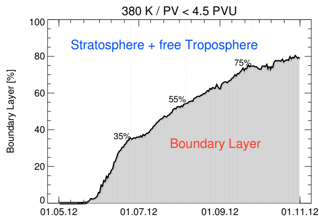
Figure 9. Temporal evolution of contributions of air masses from the boundary layer to the composition of the Asian monsoon anticyclone. The shown percentages are mean values calculated for air masses in Asia in the region between 15 and 50° N and 0 and 140° E at 380 \pm 0.5 K (see black rectangles in Fig. 7) with PV values lower than 4.5 PVU marking the edge of the anticyclone.
