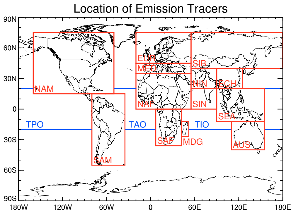
Figure 1. Global geographic location of artificial boundary layer source regions in the CLaMS model, also referred to as “emission tracers”. The latitude and longitude range for each emission tracer is listed in Table 1.
