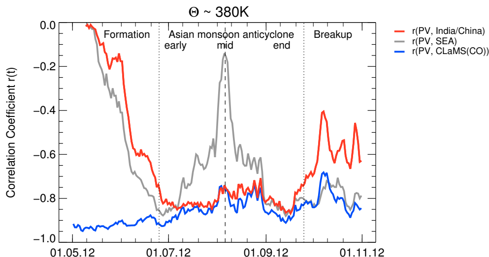
Figure 5. Time-dependent correlation coefficients for the spatial distribution between PV and the emission tracer for India/China (red), the emission tracer for Southeast Asia (grey), and CLaMS CO (blue) at 380 K potential temperature (see text for more details) in a region between 15 and 50° N and 0 and 140° E (shown as black rectangles in Figs. 2 and 3).
