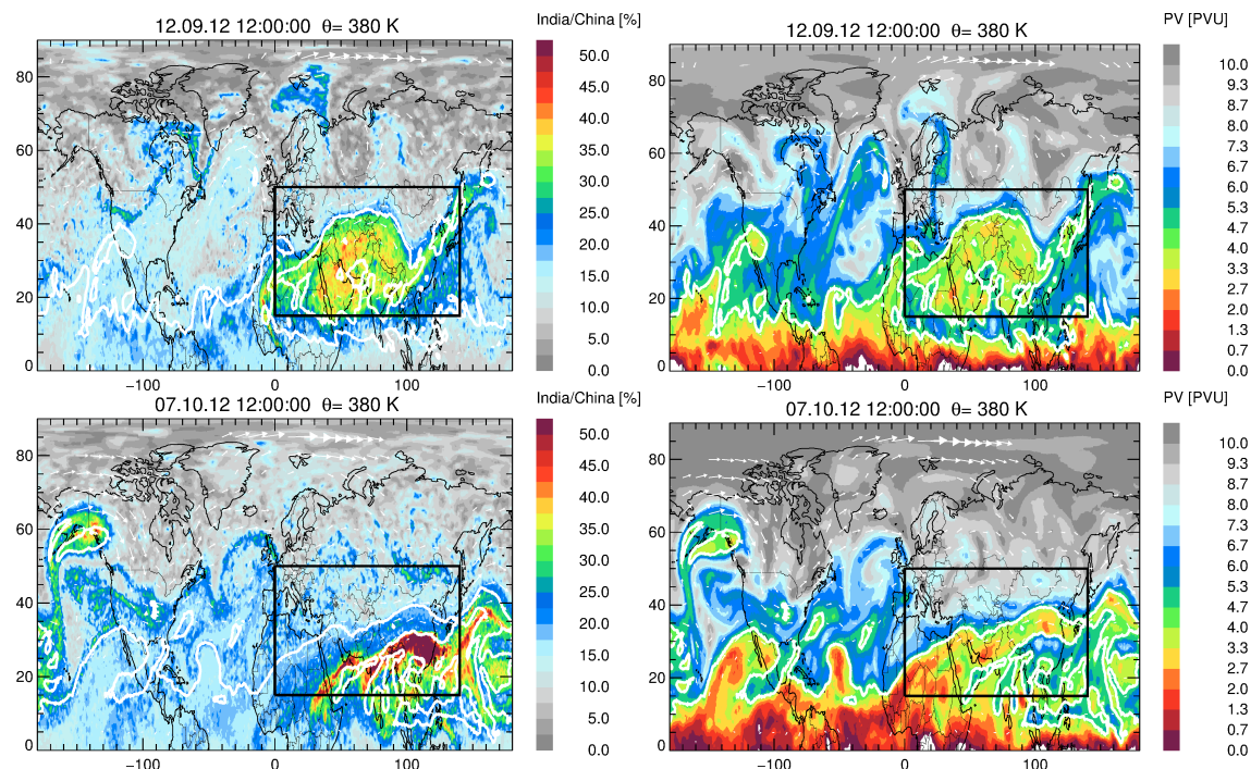
Figure 3. The same as Fig. 2 but on 12 September 2012 (top) during the late phase of the anticyclone and on 7 October 2012 (bottom) showing the distribution of emission tracers for India/China after the breakup of the anticyclone.
