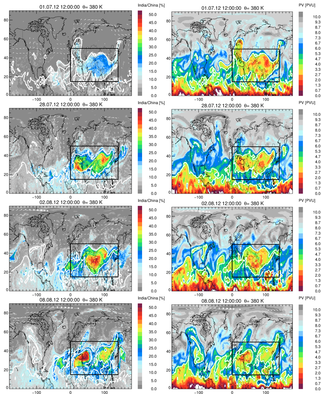
Figure 2. The horizontal distribution of the fraction of air originating in India/China (left) and PV (right) at 380 K potential temperature over Asia on 1 July 2012 (top), 28 July 2012 (second row), 2 August 2012 (third row), and 8 August 2012 (bottom). Please note that the order of the colour scale for India/China (left) and PV (right) is different, so that high contributions of emission tracers for India/China and low PV are marked in red. The horizontal winds are indicated by white arrows. The black rectangle (15–50° N, 0–140° E) highlights the region of the Asian monsoon anticyclone. The 4.5 PVU surface marks roughly the edge of the anticyclone shown as a thick white line.
