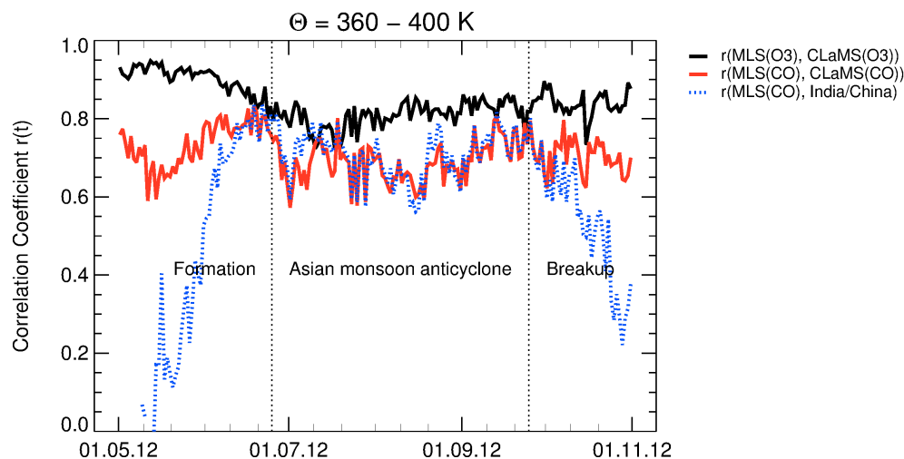
Figure 4. Correlation coefficients depending on time for tracer correlations patterns between MLS \text{O}_3 and CLaMS \text{O}_3 (black), between MLS CO and CLaMS CO (red), and between MLS CO and the CLaMS emission tracer for India/China (blue) for levels of potential temperature between 360 and 400 K (see text for more details) in a region between 15 and 50° N and 0 and 140° E (shown as black rectangles in Fig. 2 and 3).
