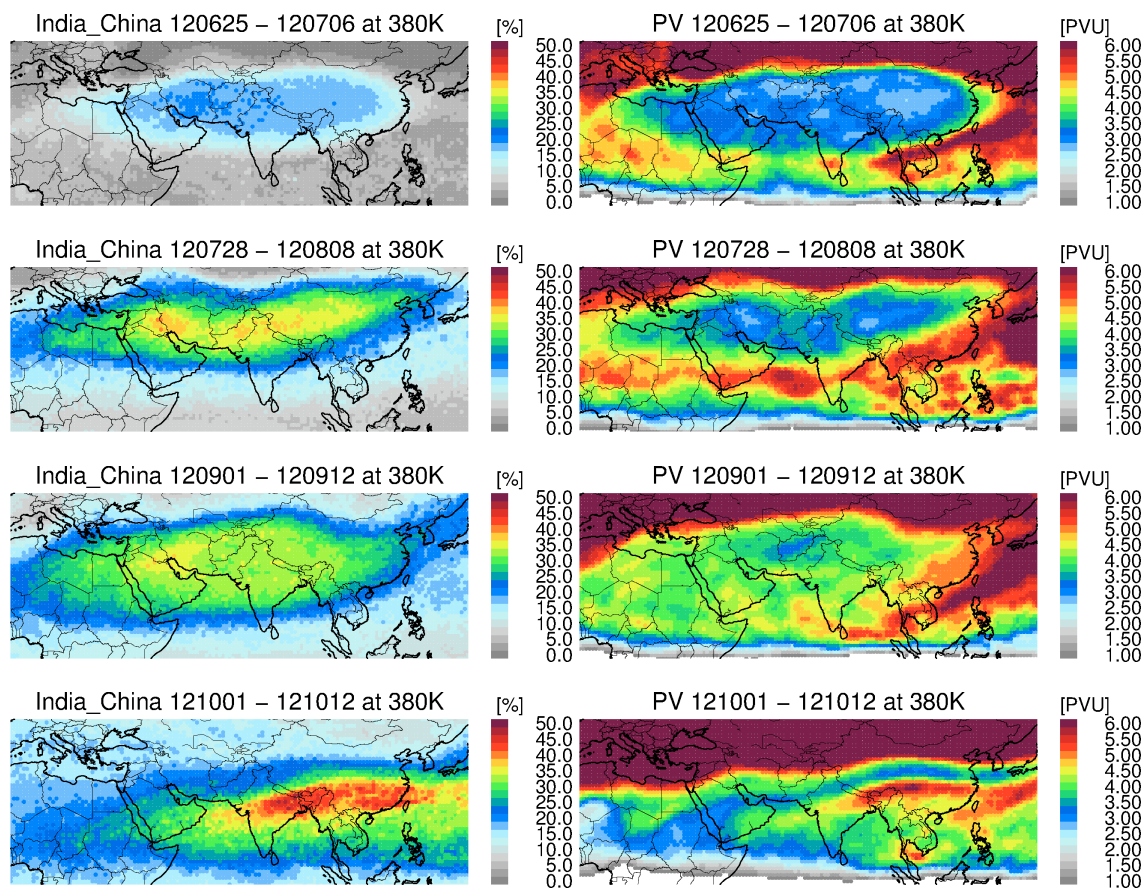
Figure 6. Twelve-day mean values of the contribution of the emission tracer for India/China (left) and PV (right) during four different phases of the Asian monsoon anticyclone: early phase (top), mid-phase (second row), end phase (third row) of the anticyclone, and after the breakup (bottom).
