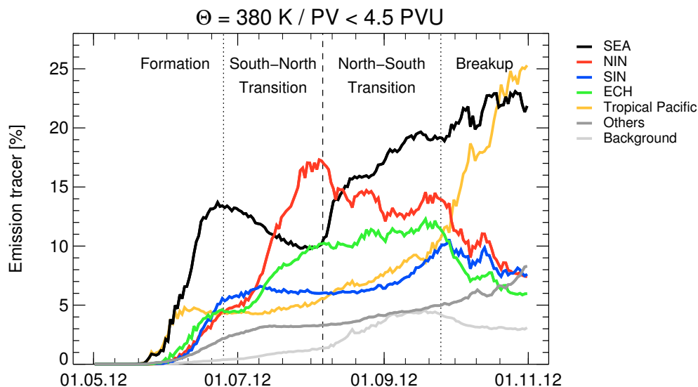
Figure 8. Temporal evolution of different emissions tracers from Southeast Asia (SEA, black), northern India (NIN, red), southern India (SIN, blue), eastern China (ECH, green), tropical Pacific Ocean (yellow), and from all other land masses plus tropical Atlantic/Indian Ocean (others, dark grey) within the Asian monsoon anticyclone at 380 K from May 2012 until the end of October 2012. Contributions of boundary sources not considered in the defined emissions tracers listed in Table 1 are summarized as background (light grey). The shown percentages are mean values calculated for air masses in Asia in the region between 15 and 50° N and 0 and 140° E at 380 \pm 0.5 K (see black rectangles in Fig. 7) with PV values lower than 4.5 PVU, marking the edge of the anticyclone.
