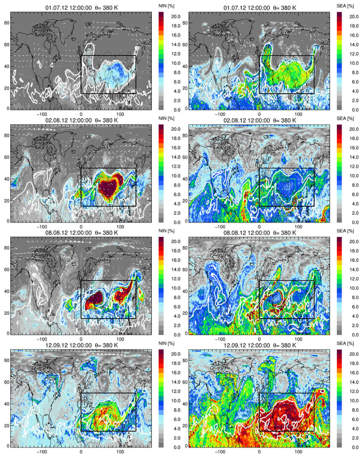
Figure 7. The horizontal distribution of the fraction of air originating in (left) northern India (NIN) and (right) Southeast Asia (SEA) at 380 K potential temperature over Asia on 1 July 2012 (top), 2 August 2012 (second row), 8 August 2012 (third row), and 12 September 2012 (bottom). The horizontal winds are indicated by white arrows. The black rectangle (15–50° N, 0–140° E) highlights the region of the Asian monsoon anticyclone. The 4.5 PVU surface marks roughly the edge of the anticyclone shown as a thick white line.
