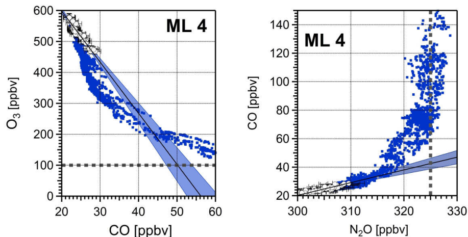
Figure 3. Linear fitting for ML 4 based on the FITEXY-routine described in Press et al. (1992). Blue dots: scatter plot of CO and O_3 (left), and N_2O and CO (right), respectively. White dots with black error bars: data points of ML 4 on the respective scatter plot. Solid black line: linear fit with confidence region (shaded area). Dotted lines: assumption of a tropospheric endmember of R(O_3)_{Trop} = 100 ppbv (top) and R(N_2O)_{Trop} = 325 ppbv (bottom).
