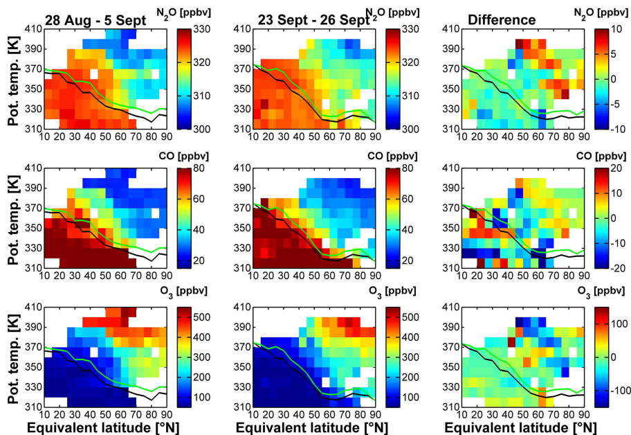
Figure 10. N_2O , CO, and O_3 distributions in potential temperature \Theta – equivalent latitude \phi_{eq} – coordinates for the TACTS 2012 campaign. Left: distributions for the initial phase of TACTS from the 28 August to 5 September. Center: distributions for the final phase of TACTS from the 23 to 26 September. Right: changes in the trace gas distributions during the TACTS 2012 campaign (final minus initial phase). The black and green line denotes the location of the dynamical (PV = 2 pvu) and thermal tropopause (WMO, 1957), respectively, for the associated time period from ECMWF data.
