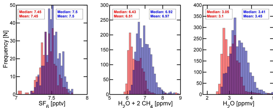
Figure 13. Histogram of trace gas mixing ratios of \text{SF}_6 (left), total water ( \text{H}_2\text{O} + 2\text{CH}_4 ) (center) and \text{H}_2\text{O} of the red and blue data points on the \text{N}_2\text{O} – \text{O}_3 -scatterplot in Fig. 12a. Purple areas display the overlap of both histograms.
