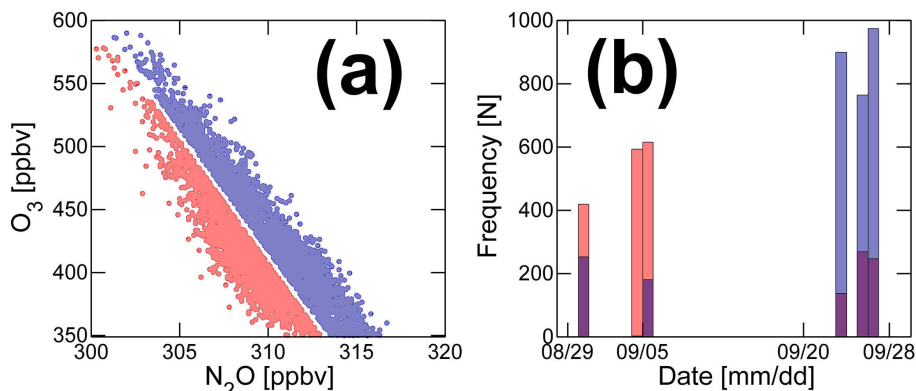
Figure 12. (a): N_2O – O_3 -scatterplot of all data points during TACTS 2012 with O_3 > 350 ppbv divided into higher (blue) and lower (red) O_3 mixing ratios on N_2O isopleths based on a linear fit regression. (b): histogram of the measurement date of the red and blue data points on the N_2O – O_3 -scatterplot. Purple areas display the overlap of both histograms.
