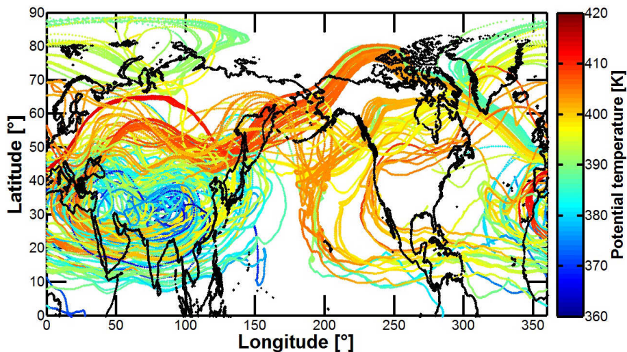
Figure 5. 50 day backward trajectories for all data points with \Theta > 370 K, PV > 7.5 pvu, and minimum \Theta along the backwards trajectories is at least 5 K smaller as \Theta at the measurement (cf. Fig. 4). Color: potential temperature along the backward trajectories based on ERA-Interim reanalysis data.
