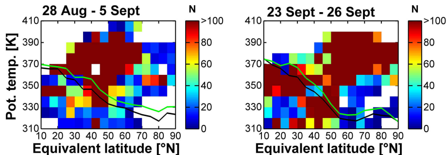
Figure 9. Data coverage (number of data points N in each bin) of TACTS 2012 in potential temperature \Theta – equivalent latitude \phi_{eq} – coordinates. Left: data coverage of the initial phase of TACTS from the 28 August to 5 September. Right: data coverage of the final phase of TACTS from the 23 to 26 September. The black and green line denotes the location of the dynamical ( PV = 2 pvu) and thermal tropopause (WMO, 1957), respectively, for the associated time period from ECMWF data.
