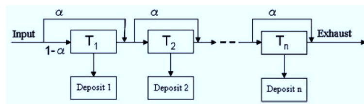
Figure 20. Schematic of the thermodynamic pseudo-equilibrium model [66].
