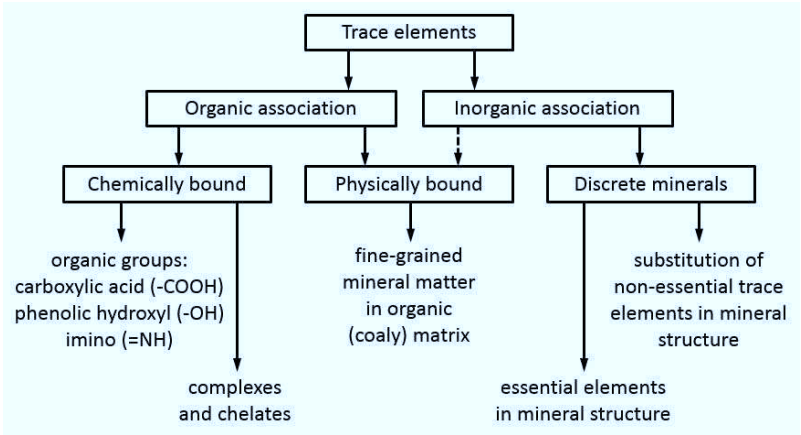
Figure 3. Modes of occurrence of trace elements in coal (adapted from [17]).
