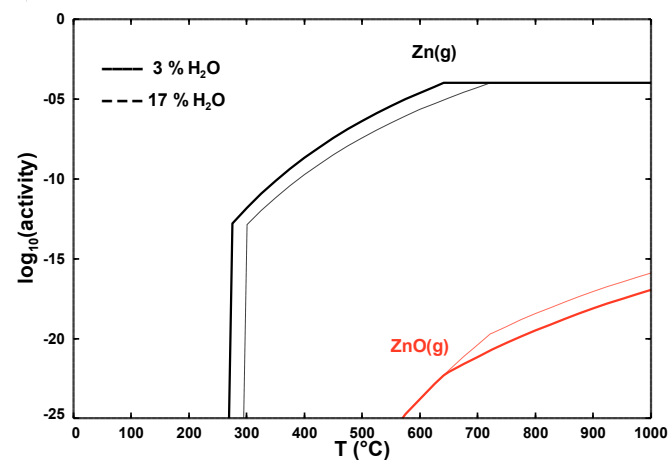
Figure 34. Gaseous zinc-containing species versus temperature in an atmosphere containing 3 – 17 % vol of H 2 O calculated by the Scheil-Gulliver cooling model.
