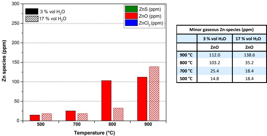
Figure 31. Concentration of minor gaseous zinc species at 900, 800, 700 and 500 °C when the atmosphere contained water vapour (3 – 17 % vol). Note that Zn(g), the major species in the gas phase, is not represented.
