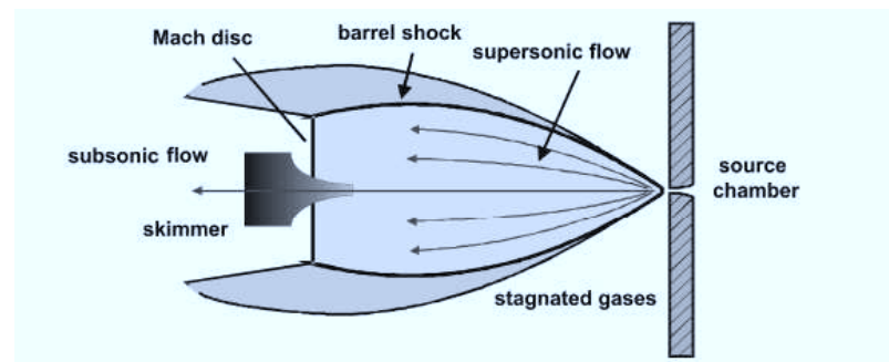
Figure 19. Schematic of the free-jet expansion [8].
