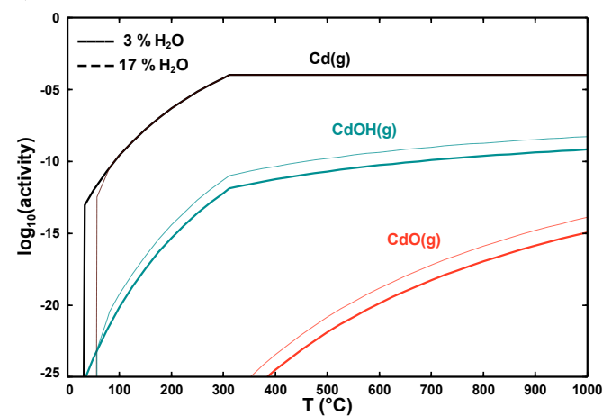
Figure 50. Gaseous cadmium-containing species versus temperature in an atmosphere containing 3 – 17 % vol of H 2 O calculated by the Scheil-Gulliver cooling model.
