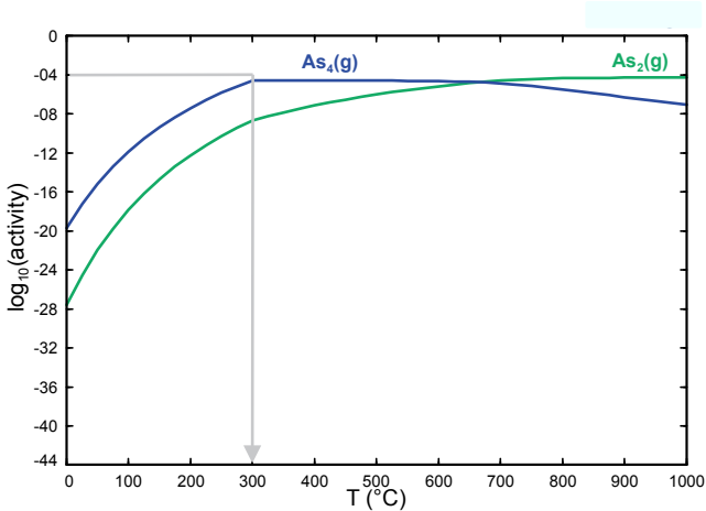
Figure 69. FactSage’s estimation of the necessary temperature for the vaporization of 100 ppm arsenic.
