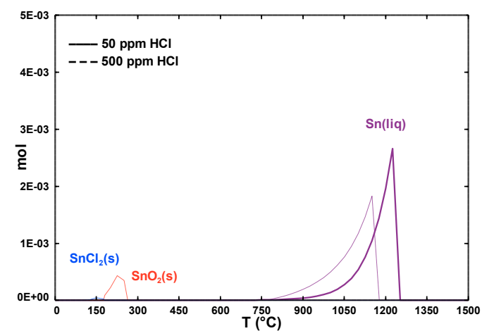
Figure 94. Speciation of the condensed phase during cooling from 1500 to 0 °C predicted by the Scheil-Gulliver cooling model in an atmosphere containing water HCl and tin.
