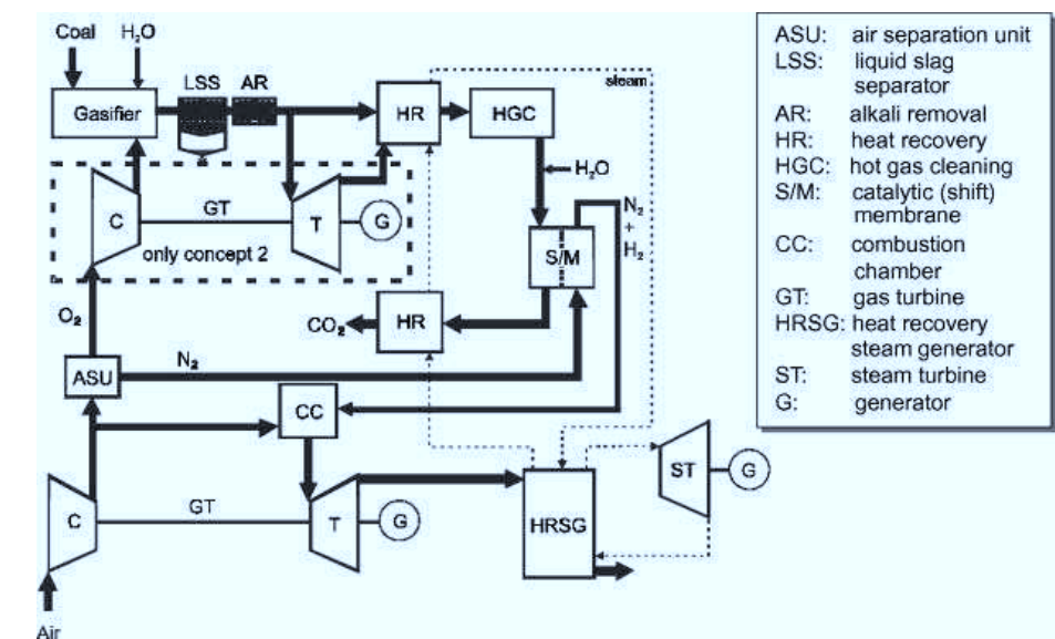
Figure 5. Flow chart of an IGCC power plant with integrated hot gas cleaning and CO 2 removal [42].
