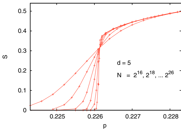
FIG. 22. (Color online) Average density S of the largest viable cluster on 5D lattices with N sites, plotted against p . Notice that we averaged here over all runs (even if they did not have a giant viable cluster), while the averages in Sec. III A (e.g., Fig. 2) were done only over runs that did have a giant cluster.
