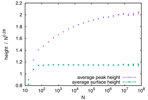
FIG. 7. (Color online) (a) Average “surface” heights at z = z_c plotted against networks network sizes on a log-log plot and average values of the peaks in each surface. Both curves clearly disagree with the scaling \propto N^{1/4} proposed in Ref. [7] but give rather an exponent 0.280(1); (b) the same data but divided by N^{0.280} .
