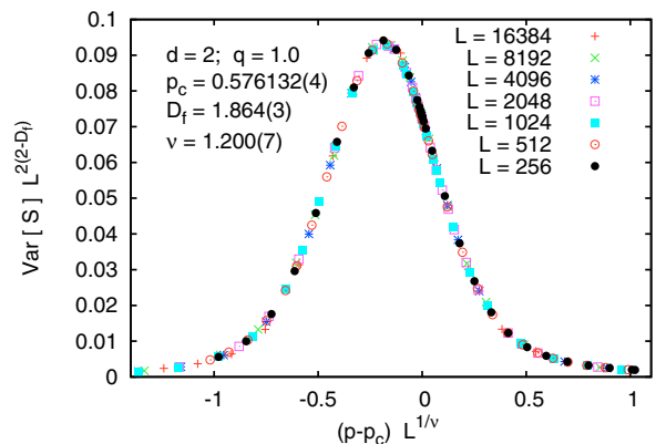
FIG. 13. (Color online) Data collapse plot for the variance of the size of the largest viable cluster on 2D lattices with q = 1.0 , plotted against rescaled values of p - p_c .
