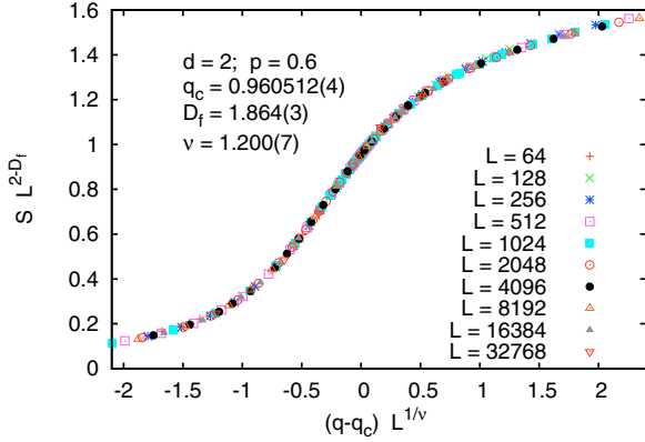
FIG. 10. (Color online) Data collapse plot for the size of the largest viable cluster on 2D lattices with p = 0.6 . The only perceptible deviation from a perfect collapse is at very large values of q , where the data for L = 256 and for L = 512 are systematically too high, due to finite-size corrections.
