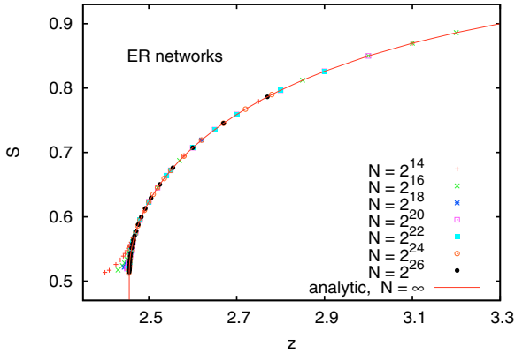
FIG. 2. (Color online) Order parameter (density of giant viable clusters) for ER networks plotted against the average degree z . The continuous curve is the prediction of Eq. (3), while the points are from simulations with N ranging from 2^{14} to 2^{26} . For S < 0.511700\dots the theoretical curve is strictly vertical, while it has square-root behavior above.
