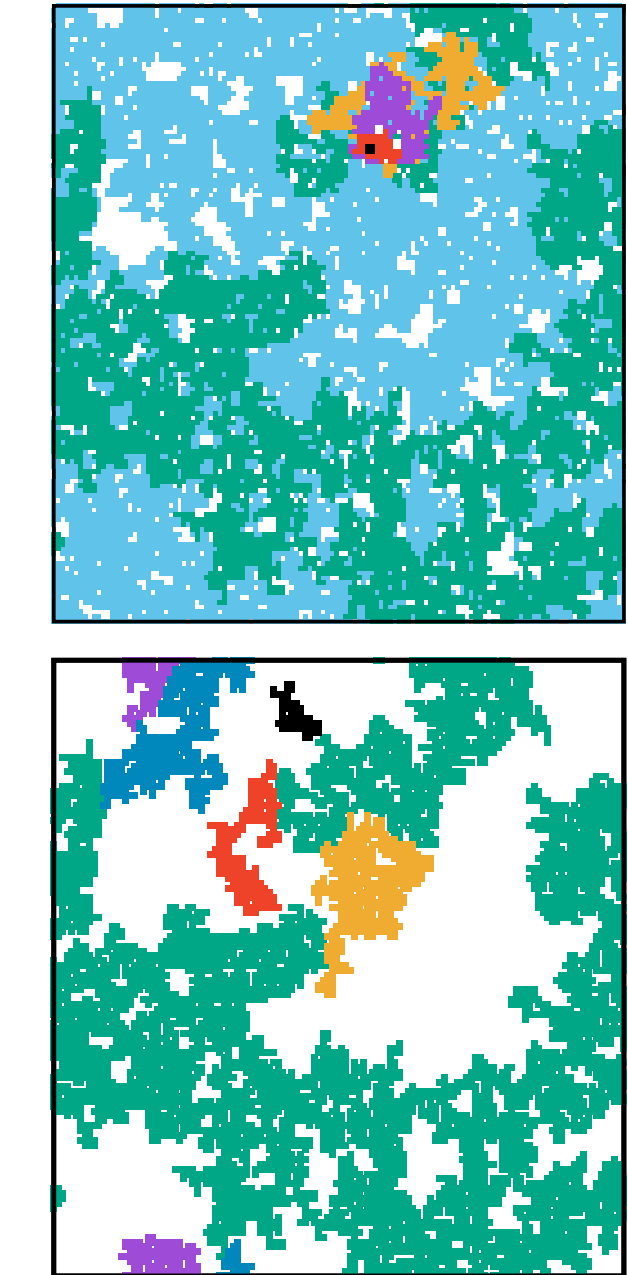
FIG. 1. (Color online) (a) Clusters \mathcal{C}_1 (all nonwhite points) to \mathcal{C}_5 (dark blue) attached to the site i indicated by the black dot. Each color corresponds to one terrace, with light blue < green < orange < magenta < red indicating increasing heights. (b) Six large clusters of height 2, all attached to points in the cluster \mathcal{C}_1 shown in panel (a). Notice that all these clusters are fully contained in \mathcal{C}_1 , and no two clusters overlap partially. They are either disjoint or one is a subset of the other. Notice also that some of these clusters touch each other, indicating the possibility that some adjacent terraces may have equal heights. The control parameter is set such that ordinary percolation would be supercritical, but mutually interdependent percolation of viable clusters is subcritical.
