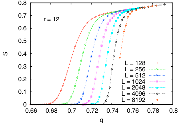
FIG. 29. (Color online) Densities of the largest viable cluster for the model of Ref. [35] with r = 12 , plotted against q for various system sizes. Here averages are taken over all runs, including those with no giant viable cluster.
