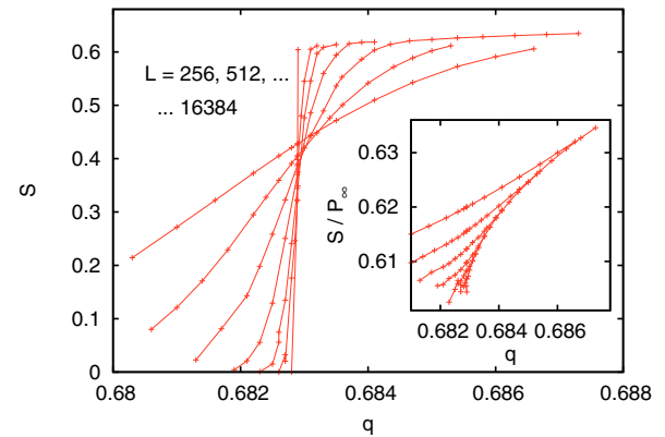
FIG. 26. (Color online) Average density S of the largest viable cluster on 2D lattices with random dependency links and dependency links between nearest neighbors, plotted against q . In the main figure, averages are taken over all runs (even they did not lead to a giant viable cluster, while the inset shows averages restricted to runs with giant viable clusters.
