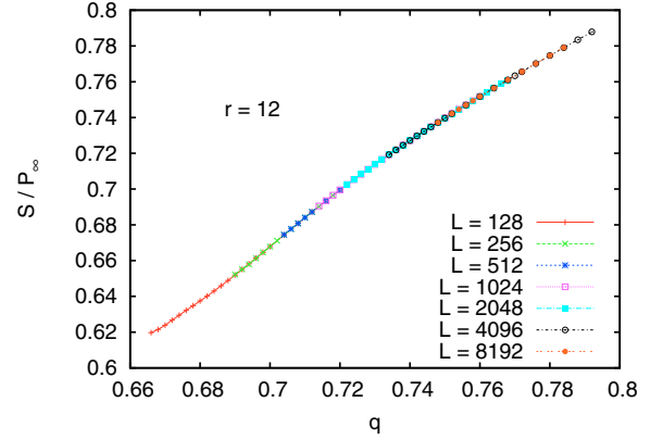
FIG. 30. (Color online) Densities of the largest viable cluster for the model of Ref. [35] with r = 12 (same data as in Fig. 28) but conditioned on clusters which do have a giant viable cluster.
