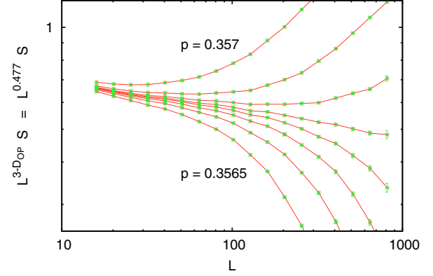
FIG. 15. (Color online) Log-log plot of L^3 S / L^{D_{OP}} against L for eight values of p close to p_c . Here D_{OP} = 2.523(1) is the fractal dimension in three-dimensional OP [55,56]. Indeed, since we used helical b.c., where the number N of lattice sites was always a power of 2, some of the lattices were not strictly cubes. In these cases, L was nevertheless defined as L = N^{1/3} , even if this was not an integer. The values of p are (from top to bottom) 0.357, 0.3568, 0.35673, 0.35670, 0.35668, 0.35665, 0.3566, and 0.3565.
