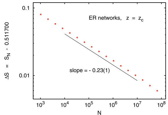
FIG. 4. (Color online) Differences between the data points for z = z_c and the theoretical value 0.511700 towards which they should converge for N \rightarrow \infty . We see indeed a straight line on a log-log plot, which leads to Eq. (5).
