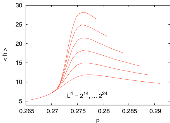
FIG. 18. (Color online) Average SOS landscape heights for 4D lattices, plotted against p .
