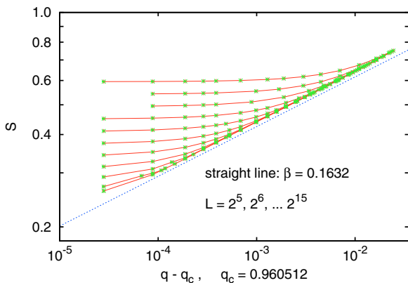
FIG. 11. (Color online) Log-log plot of S against q - q_c , demonstrating the power law S \sim (q - q_c)^\beta .
