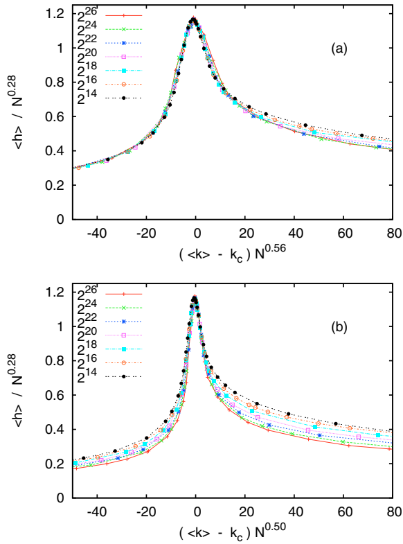
FIG. 9. (Color online) Data collapse plots of rescaled surface heights \langle h \rangle / N^\gamma against (z - z_c)N^{2\gamma} with 2\gamma = 0.56 (a) and against (z - z_c)N^{0.5} (b). Neither plot is fully satisfactory, but in spite of the bigger overall discrepancies we claim that panel (b) gives the correct collapse in the critical region.
