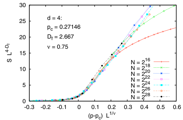
FIG. 20. (Color online) The same data as in Fig. 19 but plotted such that the collapse onto a single curve near the critical point.
