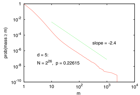
FIG. 24. (Color online) Log-log plot of the integrated mass distribution of finite 5D viable clusters at N = 2^{26} ( L \approx 37 ) and p = 0.22615 . The straight line indicates the scaling of finite but large viable clusters.
