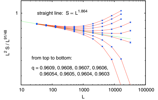
FIG. 12. (Color online) Log-log plot of L^2 S / L^{91/48} against L for eight values of q close to q_c . The power 91/48 = 1.8958\dots was chosen because it is the fractal dimension of the incipient giant cluster in critical OP. Thus any deviation of the critical curve from a horizontal line indicates that the present model and OP are in different universality classes.
