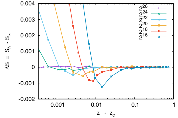
FIG. 3. (Color online) Differences between the data points and the theoretical curve in Fig. 2. To enhance the region z \approx z_c , the data are plotted against z - z_c on a logarithmic axis.
