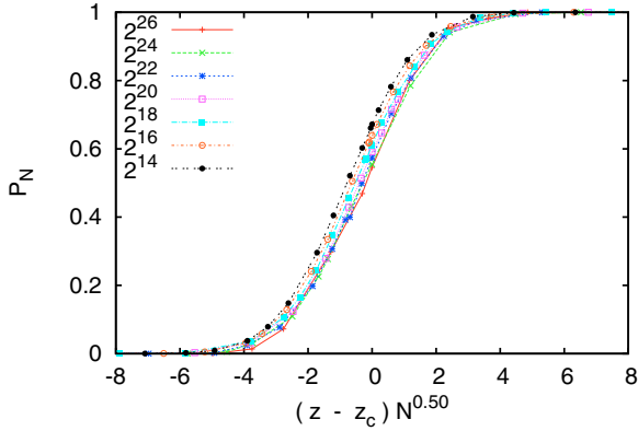
FIG. 5. (Color online) P_N(z) , the probability to have a giant viable cluster on an ER network of size N , plotted against (z - z_c)N^{1/2} .
