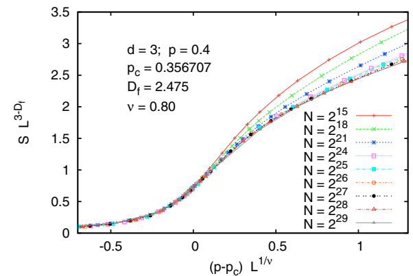
FIG. 16. (Color online) Data collapse plot for the size of the largest viable cluster on 3D lattices. In contrast to the 2D case we now have huge corrections to scaling in the supercritical region.
