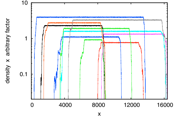
FIG. 33. (Color online) Densities of giant viable clusters on 2D lattices of size L_\perp \times L_\parallel = 2048 \times 16384 , with r = 9 and q = 0.772 (which is our best estimate for q_c at r = 9 ). Shown are the 1D projections of these densities for 10 typical realizations, multiplied with arbitrary factors to avoid overlaps. Due to local isotropy, we would expect that interface widths should become \sim L_\perp in the large system limit. Actual interfaces are much sharper.
