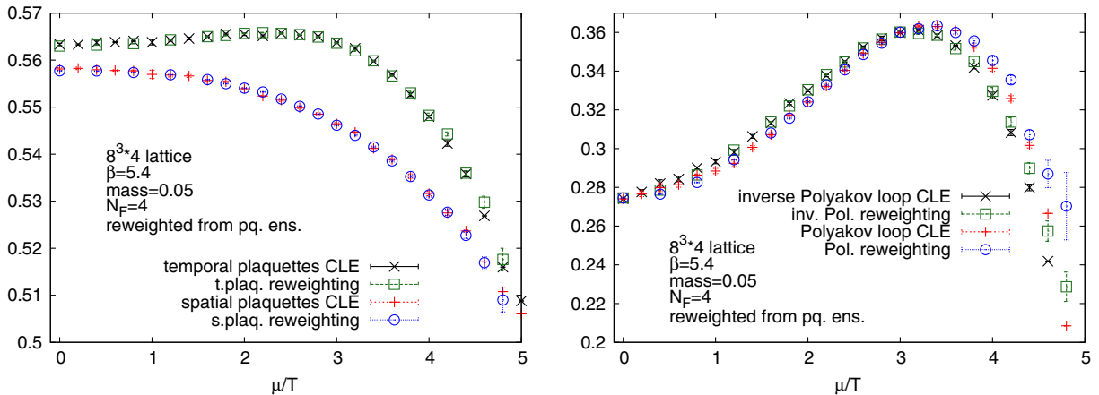
FIG. 5 (color online). Comparison of the plaquette averages and Polyakov loops as a function of \mu at a fixed \beta = 5.4 calculated with CLE and reweighting from the phase-quenched ensemble.
