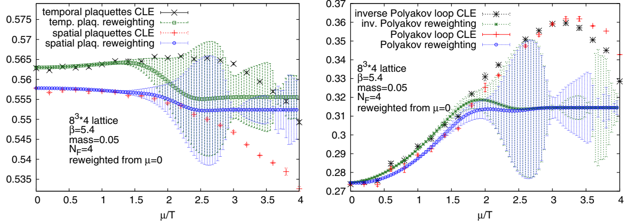
FIG. 1 (color online). Comparison of plaquette averages and Polyakov loops and inverse Polyakov loops [defined in and below Eq. (11)] calculated with CLE and reweighting from the \mu = 0 ensemble.
