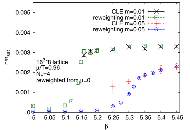
FIG. 11 (color online). Comparison of the fermionic density as a function of the \beta parameter at a fixed \mu/T = 0.96 , using m = 0.01 and m = 0.05 as indicated, calculated with CLE and reweighting from the \mu = 0 ensemble on 16^3 \times 8 lattices.
