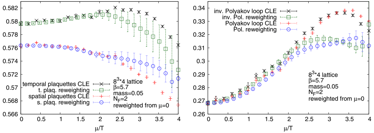
FIG. 4 (color online). Comparison of plaquette averages and Polyakov loops calculated with CLE and reweighting from the \mu = 0 ensemble. We use N_F = 2 fermion flavors for the data presented in this plot.
