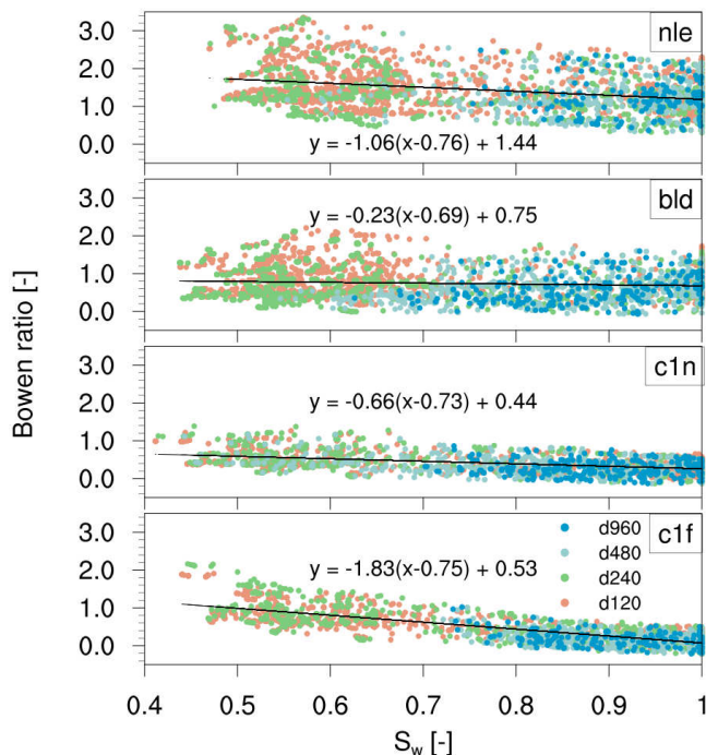
Figure 7. Distribution of the Bowen ratio as a function of relative soil moisture along cross-section AA'. The distribution is plotted separately for different land-use types in the sub-catchment.
