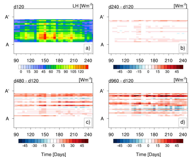
Figure 9. (a) Time evolution of 5-day mean latent heat flux (LH) along cross-section AA' for the d120 domain. (b) Difference in the time evolution of LH between the d240 and d120. (c) Difference in the time evolution of LH between the d480 and d120. (d) Difference in the time evolution of LH between the d960 and d120. For d120, d240 and d480, the LH fluxes were spatially aggregated to 960 m resolution.
