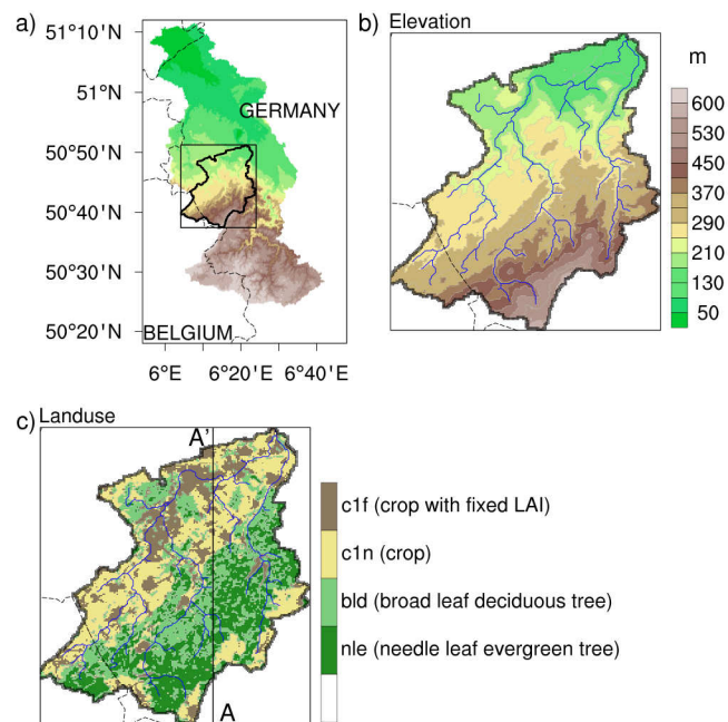
Figure 2. (a) Topography of the Rur catchment, which lies at the border of Germany, Belgium, Luxembourg and the Netherlands. (b) Topography of the sub-catchment of the Rur used in this study (catchment of the River Inde including the Wehebach tributary in the east), overlaid with the stream networks. (c) Land-use map of the sub-catchment.
