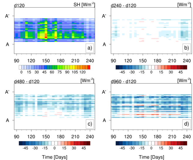
Figure 8. (a) Time evolution of 5-day mean sensible heat flux (SH) along cross-section AA' for the d120 domain. (b) Difference in the time evolution of SH between the d240 and d120. (c) Difference in the time evolution of SH between the d480 and d120. (d) Difference in the time evolution of SH between the d960 and d120. For d120, d240 and d480, the SH fluxes were spatially aggregated to 960 m resolution.
