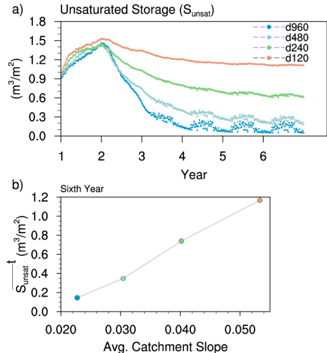
Figure 4. (a) Time series of unsaturated storage per unit catchment area ( S_{\text{unsat}} ) for the sub-catchment at the four grid resolutions. (b) Relationship between the annual average unsaturated storage ( \overline{S_{\text{unsat}}}^t ) and the average catchment slope for the four grid resolutions.
