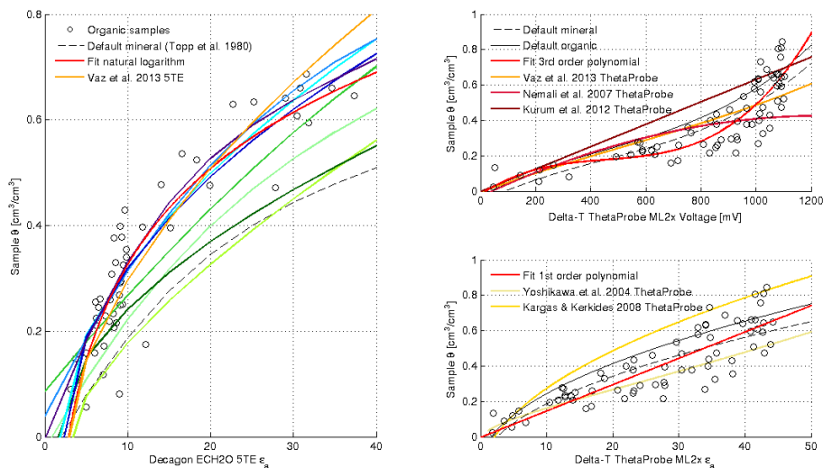
Figure 4. Comparison between reported pedrophysical and empirical relationships applied to our data measured in organic soil layers for the Decagon 5TE apparent relative permittivity \epsilon_a (left column), and ThetaProbe voltage [mV] (upper right column) as well as \epsilon_a (lower right column) against volumetric moisture content \theta including respective manufacturer's default calibration curves and best fits.
