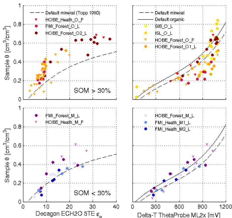
Figure 2. Decagon 5TE apparent relative permittivity \varepsilon_a (left) and ThetaProbe voltage [mV] (right column) against volumetric moisture content \theta for organic (SOM > 30 %, top row) and mineral soil horizons (SOM < 30 %, bottom row), laboratory • and field ▼ data, with color codes from highest to lowest SOM content (yellow – dark red and purple – dark blue, respectively). For mineral horizons, blue and purple signatures mean SOM < 10 and > 10 %, respectively. Manufacturer’s default calibration curves (black dashed and continuous lines) are also included. Regarding the specifications of sample names and respective SOM fractions, please see Table 1.
