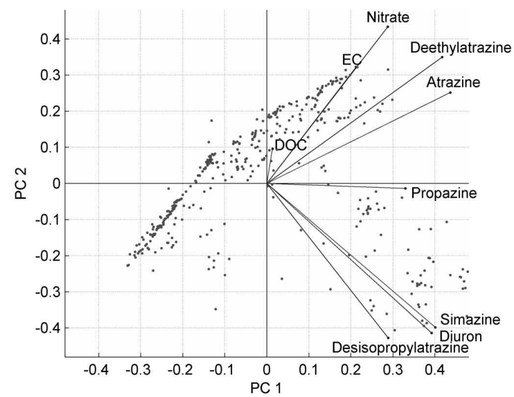
Figure 13: Loadings and scores plot of PCA.
