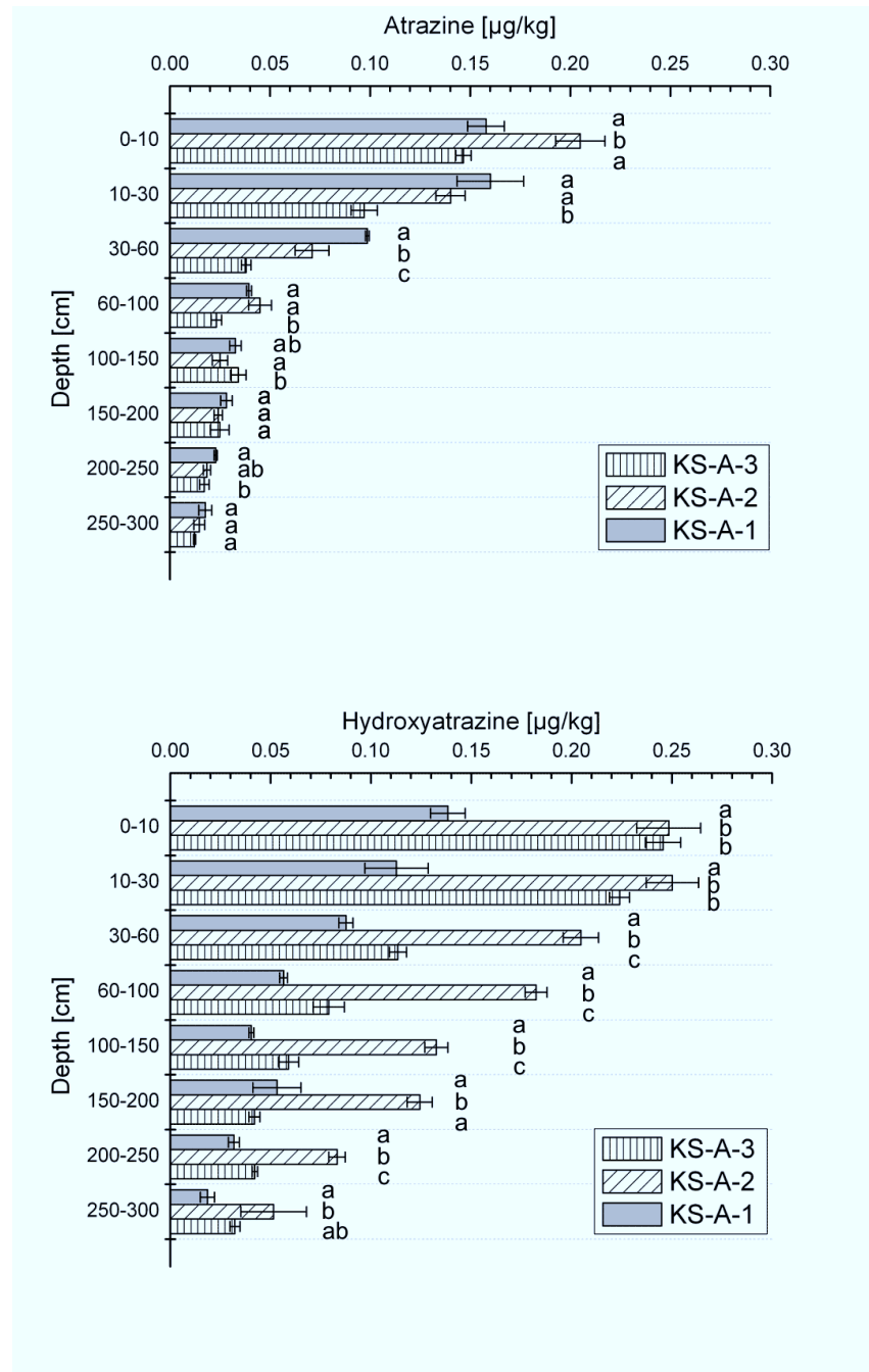
Figure 15: Concentration profiles of atrazine and 2-hydroxyatrazine residues determined by three soil cores (KS-A-1 to 3) of the Krauthausen gleyic cambisol, 21 years after the ban of atrazine. Error bars show standard deviations of triplicates. Different letters indicate significant differences of mean atrazine concentrations between Krauthausen soil profiles for p < 0.05 , using the Tukey test.
