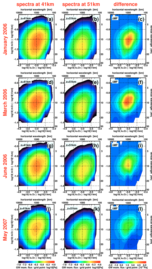
Figure 6. HIRDLS gravity wave momentum flux spectra for the four cases illustrated in Fig. 4. Upper row (a–c): January 2006, westward vertical shear of the zonal wind, u(z_1) < 0 and u(z_2) < 0 ; second row (d–f): March 2006, eastward wind shear, u(z_1) < 0 and u(z_2) > 0 ; third row (g–i): June 2006, westward wind shear, u(z_1) > 0 and u(z_2) < 0 ; and lower row (j–l): May 2007, eastward wind shear, u(z_1) > 0 and u(z_2) > 0 . The left column (a, d, g, j) shows spectra for 41 km altitude, and the middle column (b, e, h, k) for 51 km altitude. These altitudes correspond to the lower and upper levels z_1 and z_2 , respectively, in Fig. 4. The right column (c, f, i, l) shows the differences between the spectra at 41 km and the spectra at 51 km altitude.
