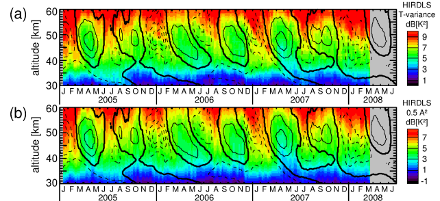
Figure B1. Altitude–time cross sections of HIRDLS gravity wave (a) temperature variances (no vertical window applied), and (b) squared temperature amplitudes determined in 10 km vertical windows from the HIRDLS altitude profiles. Values in (b) were divided by 2 to be comparable to the variances in (a). Units in (a) and (b) are \text{dB}(\text{K}^2) . Values in (a) and (b) are averages over the latitude band 10^\circ \text{S} – 10^\circ \text{N} . Contour lines indicate the zonal wind: westward wind is dashed, and the bold contour line indicates zero wind. Contour increment is 20 \text{ m s}^{-1} .
