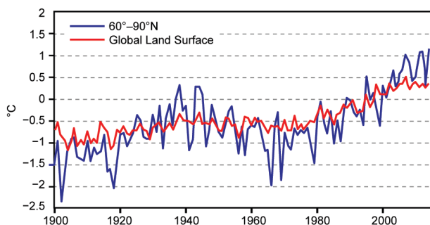
FIG. 5.1. Arctic and global mean annual surface air temperature anomalies ( ^{\circ}\text{C} ) for the period 1900–2014 relative to the 1981–2010 mean value. The data are for land stations only. Results are based on the CRUTEM4v dataset.
