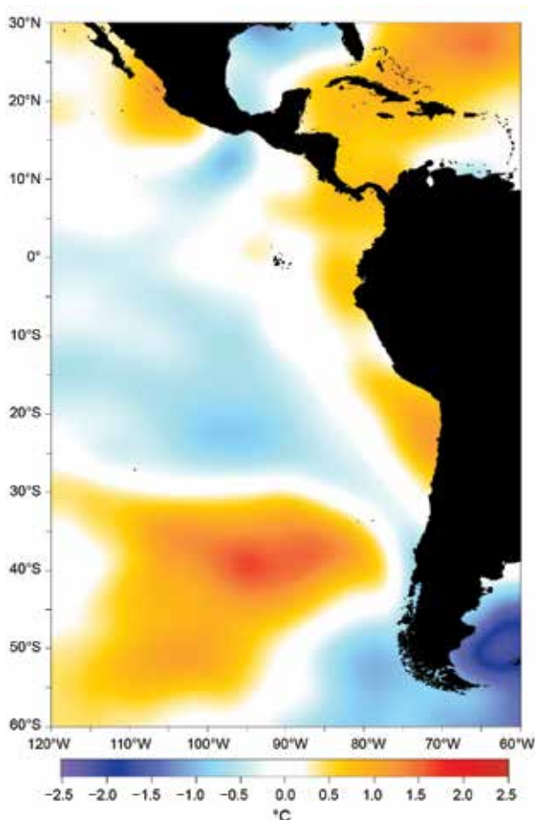
FIG. 7.11. Mean annual sea surface temperature anomalies ( ^\circ\text{C} ; 1971–2000 base period). Data source: NOAA/NCEP/EMC/CMB/GLOBAL Reyn_Smith Olv2. (Processed by CIIFEN, 2015.)
