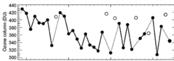
FIG. 5.5. Time series of area-averaged minimum total ozone for March in the Arctic, calculated as the minimum of daily average column ozone poleward of 63° equivalent latitude (Butchart and Remsburg 1986). Open circles represent years in which the polar vortex broke up before March. Ozone in those years was relatively high because of mixing with air from lower latitudes and higher altitudes and a lack of significant chemical ozone depletion. Data are adapted from Müller et al. (2008) and WMO (2014), updated using ERA-Interim reanalysis data (Dee et al. 2011a). Ozone data from 1979–2012 are based on the combined total column ozone database version 2.8 produced by Bodeker Scientific ( www.bodekerscientific.com/data/total-column-ozone ). Data for 2013 and 2014 are from the Ozone Monitoring Instrument aboard the NASA Aura satellite.
