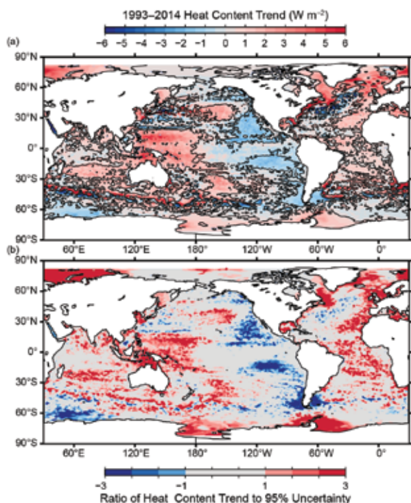
FIG. 3.6. (a) Linear trend from 1993–2014 of the combined satellite altimeter and in situ ocean temperature data estimate of upper (0–700 m) ocean heat content anomaly ( \text{W m}^{-2} ) analyzed following Willis et al. (2004) but relative to a monthly Argo climatology. Areas with statistically significant trends (red and blue areas in panel b) are outlined in black. (b) Signed ratio of the linear trend to its 95% uncertainty estimate, with increasing color intensity showing regions with increasingly statistically significant trends.
