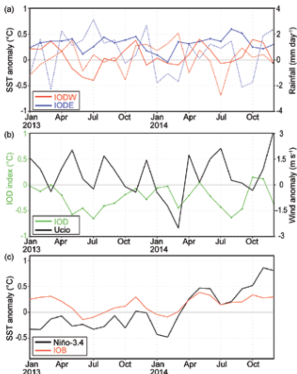
FIG. 4.41. (a) Monthly anomalies of SST ( ^{\circ}\text{C} , solid lines) and precipitation ( \text{mm day}^{-1} , dashed lines) in the eastern (IODE, 90^{\circ}\text{--}110^{\circ}\text{E} , 10^{\circ}\text{S--}0^{\circ} , blue lines) and western pole (IODW, 50^{\circ}\text{--}70^{\circ}\text{E} , 10^{\circ}\text{S--}10^{\circ}\text{N} , red lines) of IOD. (b) As in (a), but for the IOD index (measured by the SST difference between IODW and IODE, green line) and surface zonal wind anomaly ( \text{m s}^{-1} ) in the central equatorial IO (Ucio, 70^{\circ}\text{--}90^{\circ}\text{E} , 5^{\circ}\text{S--}5^{\circ}\text{N} , black line). (c) As in (a), but for the SST anomalies in Niño-3.4 region ( 170^{\circ}\text{--}120^{\circ}\text{W} , 5^{\circ}\text{S--}5^{\circ}\text{N} , black line) and the tropical IO (IOB, 40^{\circ}\text{--}120^{\circ}\text{E} , 20^{\circ}\text{S--}10^{\circ}\text{N} , red line). Anomalies calculated relative to the 1982–2013 climatology. These are based on the NCEP optimum interpolation SST (Reynolds et al. 2002), monthly GPCP precipitation analysis, and JRA-55 atmospheric reanalysis (Ebita et al. 2011).
