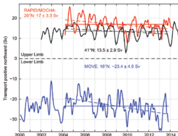
FIG. 3.22. Estimates of Atlantic Ocean meridional overturning circulation from the Argo/Altimetry estimate at 41°N (black; Willis 2010), the RAPID/MOCHA/WBTS 26°N array (red; McCarthy et al. 2015), and the German/NOAA MOVE array at 16°N (blue; Send et al. 2011) shown versus year. All time series have a 3-month second-order Butterworth low-pass filter applied. Horizontal lines are mean transports during similar time periods as listed in the corresponding text. Dashed lines are trends for each series over the same time period. For the MOVE data, the net zonal and vertical integral of the deep circulation represents the lower limb of the MOC (with a negative sign for southward flow) and hence a stronger negative southward flow represents an increase in the MOC.
