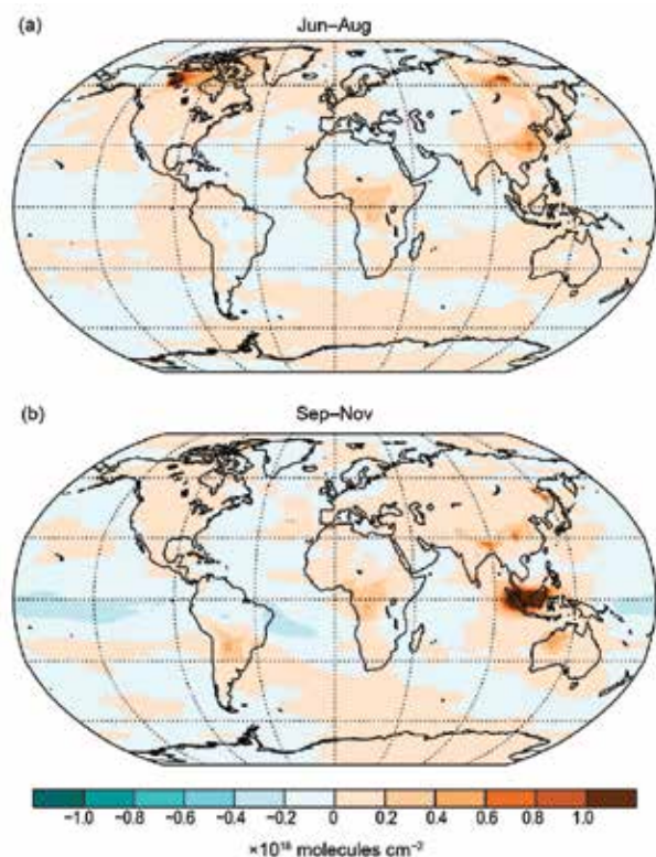
FIG. 2.51. MACC anomalies of the total column CO for (a) Jun–Aug and (b) Sep–Nov 2014 with respect to the period 2003–14 ( \times 10^{18} \text{ molecules cm}^{-2} ).
