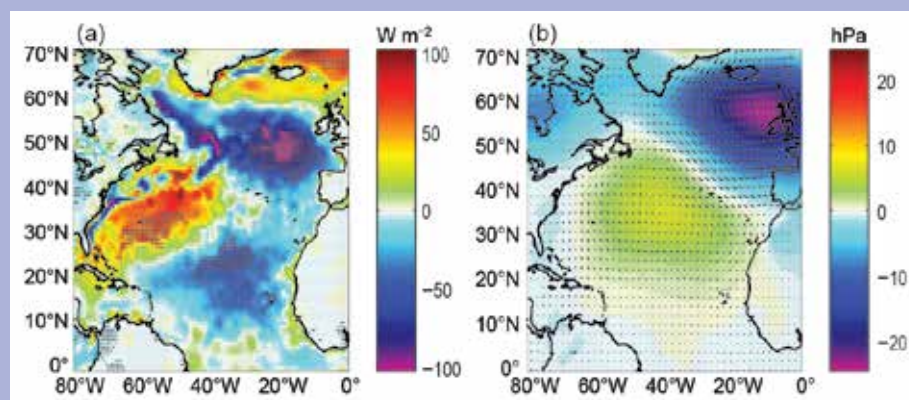
FIG. SB3.2. (a) ERA-Interim net heat flux anomaly (colored field, blue shows increased net ocean heat loss in W m -2 ) for Jan–Feb 2014 relative to the 1972–2012 climatological mean for these months. Stippling indicates regions in which the net heat flux anomaly in Jan–Feb 2014 was the strongest in this two month interval since 1979. (b) Corresponding OAF flux wind field anomaly and ERA-Interim sea level pressure anomaly.
