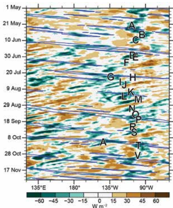
FIG. 4.26. Longitude-time Hovmöller of OLR ( \text{W m}^{-2} , Lee 2014) averaged 10^{\circ}\text{--}20^{\circ}\text{N} . Unfiltered anomalies from a daily climatology are shaded. Negative anomalies (green) indicate enhanced convection. Anomalies filtered for Kelvin waves are contoured in blue at -10 \text{ W m}^{-2} . Letters indicate the genesis of ENP TCs.
