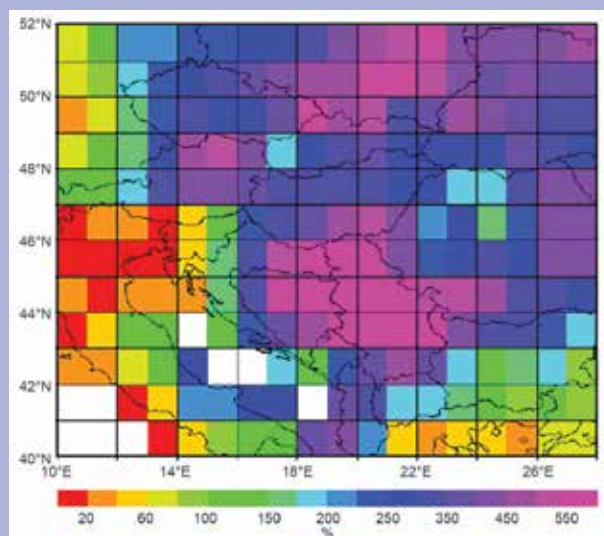
FIG. SB7.4. Relative anomaly of precipitation (%) for southeast Europe on 13–18 May 2014 based on a long-term mean for a 6-day period in May. (Source: GPCC.)
