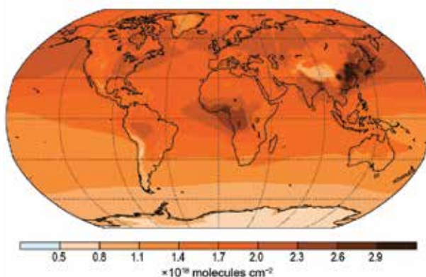
FIG. 2.50. Monitoring Atmospheric Composition and Climate (MACC) reanalysis average total column CO for the period 2003–14 ( \times 10^{18} \text{ molecules cm}^{-2} ).
