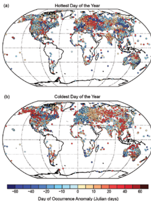
FIG. 2.7. The anomaly in Julian days of the date of the hottest and coldest day in 2014 using ISD-Lite.
