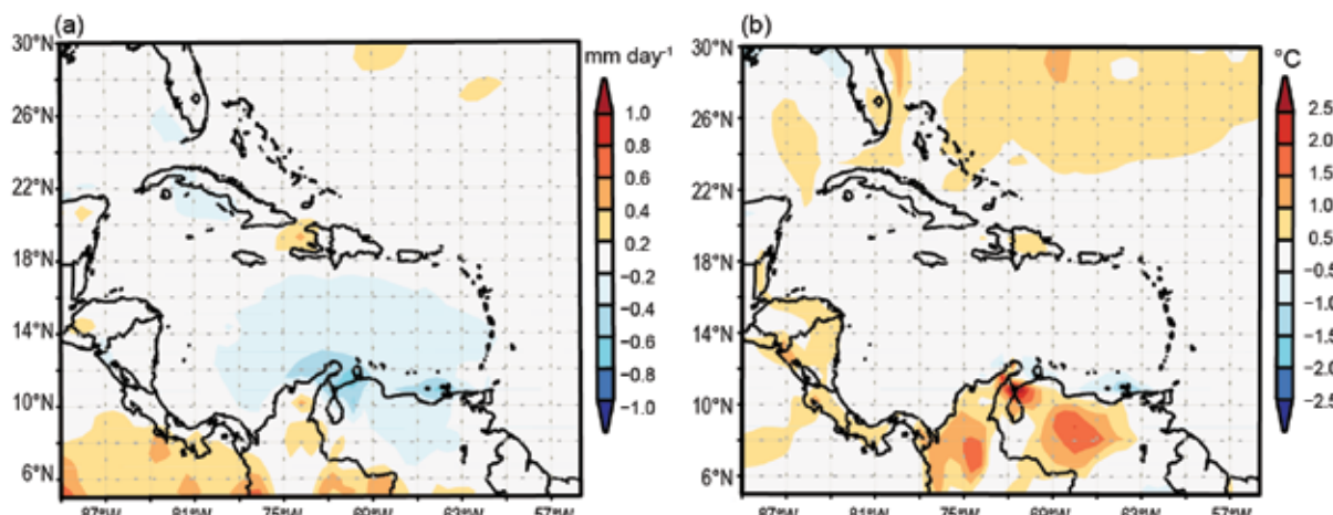
FIG. 7.10. 2014 annual (a) rainfall (mm day -1 ) and (b) temperature (°C) anomalies across the Caribbean basin. Anomalies are with respect to 1981–2010 mean. (Source: ERA-Interim.)
