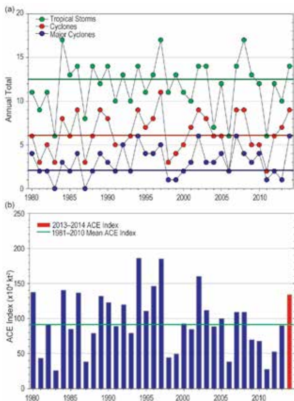
FIG. 4.32. Annual TC statistics for the SIO for 1980–2014: (a) number of tropical storms, cyclones, and major cyclones and (b) the estimated annual ACE index ( \text{kt}^2 \times 10^4 ) for all TCs during which they were at least tropical storm or greater intensities (Bell et al. 2000). The 1981–2010 means (green lines) are included in both (a) and (b). Note that ACE Index is estimated due to lack of consistent 6-h sustained winds for each storm.
