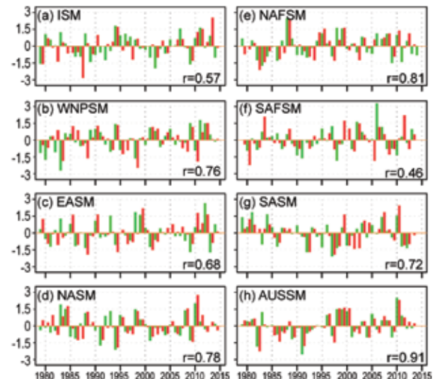
FIG. 4.11. Normalized summer monsoon mean precipitation (green) and circulation (red) indices in each of eight regional monsoons (a)–(h). The indices are normalized by their corresponding standard deviation. The correlation coefficient between seasonal mean precipitation and circulation indices is shown in the lower right corner of each panel. The monsoon regions indicated here are defined in Table 4.1.
