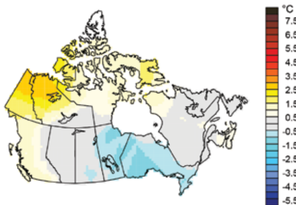
FIG. 7.2. Annual average temperature anomalies ( ^{\circ}\text{C} ) in Canada for 2014 (base period: 1961–90). (Source: Environment Canada.)
