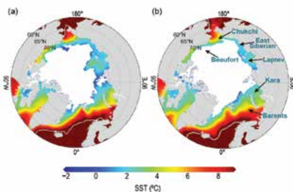
FIG. 5.24. (a) Mean SST ( ^{\circ}\text{C} ) in Aug 2014. White shading is the Aug 2014 mean sea ice extent. (Source: NSIDC) (b) Mean SST in Aug during 1982–2010. White shading indicates the median ice extent in Aug for 1982–2010. Gray contours in both panels indicate the 10^{\circ}\text{C} isotherm.
