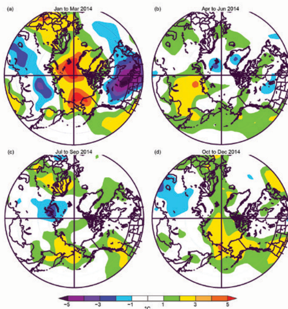
FIG. 5.2. Seasonal anomaly patterns (relative to the baseline period 1981–2010) for near-surface air temperatures ( ^{\circ}\text{C} ) in (a) winter, (b) spring, (c) summer, and (d) fall 2014. Temperature analyses are from slightly above the surface layer (at 925-mb level) to emphasize large spatial patterns rather than local features. Data are from NCEP/NCAR Reanalysis.
