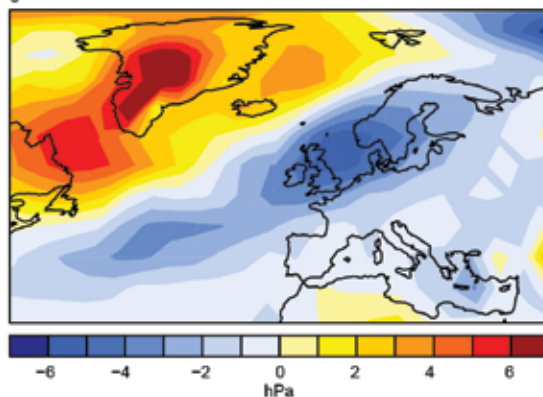
FIG. 2.27. Jul–Aug PMSL patterns for 2014. (a) Daily SNAO index anomalies from 1981–2010 for summer 2014 using NCEP reanalysis MSLP data. PMSL anomaly patterns (hPa) over Europe and the North Atlantic from 1981–2010 shown separately for (b) Jul and (c) Aug using the HadSLP2r dataset.
