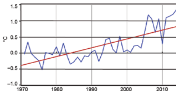
FIG. 7.6. Annual mean temperature anomalies (°C) for Mexico (base period 1971–2000). A linear trend is depicted by the red line. (Source: Servicio Meteorológico Nacional de Mexico.)
