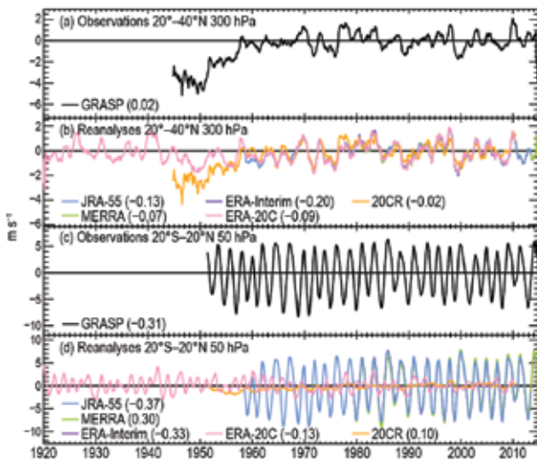
FIG. 2.32. Time series of zonal mean U-wind component ( \text{m s}^{-1} ): (a),(b) in belt 20^{\circ} – 40^{\circ}\text{N} at 300 hPa and (c),(d) in the tropical belt 20^{\circ}\text{S} – 20^{\circ}\text{N} at 50 hPa, calculated from ERA-Interim, MERRA, and JRA-55 reanalyses, 20CR, ERA-20C (Poli et al. 2013) surface data only reanalyses (20CR subsampled to where balloon data exist) and pilot balloon/radiosonde winds (GRASP). Values in legend are linear trends in interval 1981–2010 in units \text{m s}^{-1} \text{ decade}^{-1} . Note that positive (negative) changes in the zonal wind speed imply an increase in westerlies (easterlies). Data have been smoothed using a 12-point boxcar filter.
