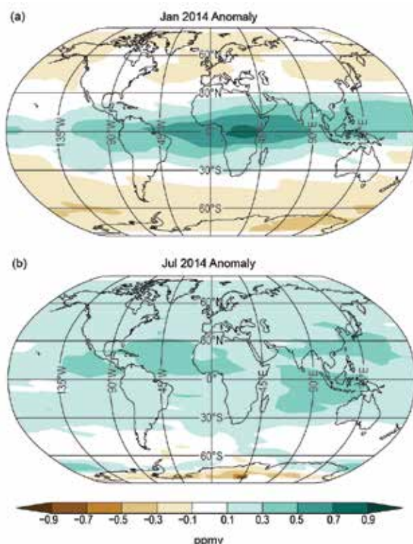
FIG. 2.46. Global stratospheric water vapor anomalies (ppmv) centered on 82 hPa in (a) Jan and (b) Jul 2014 from the Aura MLS. In Jan 2014 positive (wet) anomalies were observed in the tropics and subtropics while extratropical anomalies were weakly negative (dry). By Jul 2014 the tropical and subtropical wet anomalies had propagated to higher latitudes.
