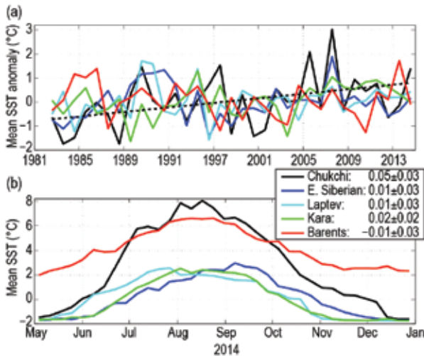
FIG. 5.26. Time series of area-averaged SST (°C): (a) SST anomalies for Aug of each year relative to the Aug mean for the period 1982–2010 for each of the marginal seas (see Fig. 5.24b) of the Arctic Ocean. The dotted black line shows the linear SST trend for the Chukchi Sea (the only marginal sea to show a trend significantly different from zero). Numbers in the legend are the linear trends (with 95% confidence intervals) in °C yr -1 . (b) SST from May to Dec 2014 for each of the marginal seas, where the OISST Version 2 weekly product has been used in the calculation.
