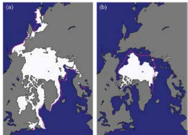
FIG. 5.21. Sea ice extent in (a) Mar 2014 and (b) Sep 2014, illustrating the respective monthly averages for the winter maximum and summer minimum extents. The magenta lines indicate the median ice extents in Mar and Sep, respectively, for the period 1981–2010. (Source: NSIDC, http://nsidc.org/data/seaice_index .)
