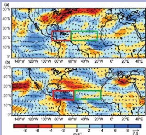
FIG. SB4.3. 60-day average vertical (200–850 hPa) wind shear ( \text{m s}^{-1} ) across the Caribbean (red box) and Main Development Region (green box) for the approximate climatological peak of the Atlantic hurricane season from 17 Aug–15 Oct.
