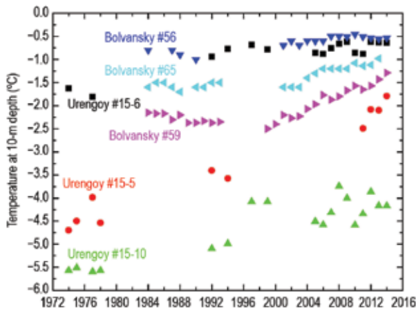
FIG. 5.18. Time series of mean annual permafrost temperatures (°C) at 10-m depth at six research sites in the European north of Russia (Bolvensky #56, 59, and 65) and in the western Siberian Arctic (Urengoy #15-5, 15-6, and 15-10).
