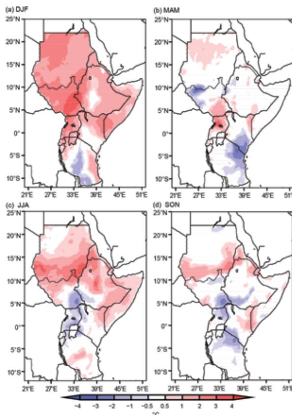
FIG. 7.21: Eastern Africa seasonal anomalies of the maximum temperature 90th percentiles (°C) with respect the 1981–2010 90th percentile mean.
