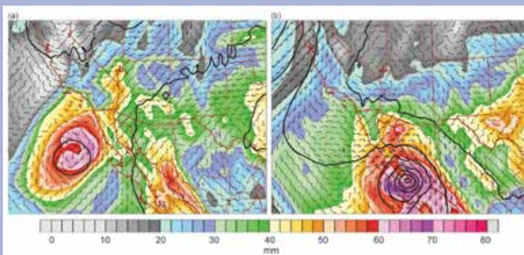
FIG. SB4.5. (a) Hurricane Norbert just off the coast of Baja California, Mexico, at 0000 UTC 9 Sep 2014, and (b) Hurricane Odile over the Baja peninsula at 0000 UTC 16 Sep 2014. Black lines denote 700-hPa height contours. Shaded regions are column precipitable water (mm). Wind barbs show wind speed and direction at 700-hPa, valid at the time of the image. Wind is plotted following the standard wind barb convention, with a half-barb representing 5 kt, a full barb 10 kt, and a filled pennant 50 kt. Orange lines denote state and country outlines.
