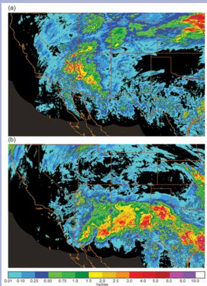
FIG. SB4.6. (a) Radar-estimated precipitation (in) for a 72-hour period ending at (a) 1200 UTC 10 Sep for the remnants associated with Hurricane Norbert, and (b) 1200 UTC 19 Sep for the remnants associated with Hurricane Odile.
