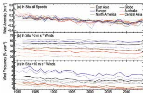
FIG. 2.28. Regional annual time series for 1981–2014 of land surface wind speeds using ISD-Lite (solid), HadISD (dashed) and McVicar et al. (2008) for Australia, showing (a) anomalies relative to 1981–2010 ( \text{m s}^{-1} ), (b) occurrence frequencies (%) for wind speeds >3 \text{ m s}^{-1} , (c) occurrence frequencies (%) for wind speeds >10 \text{ m s}^{-1} . Frequencies for Australia are not shown in (b) and (c).
