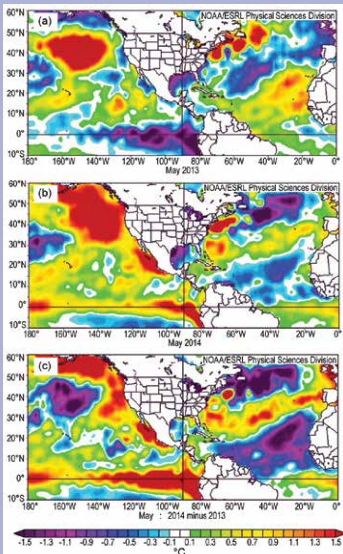
Fig. SB4.1. NOAA OI SST anomalies ( ^\circ\text{C} ) for (a) May 2013, (b) May 2014, and (c) May 2014–May 2013.
