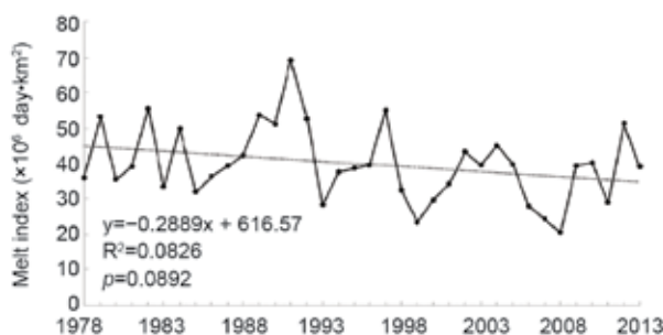
FIG. 6.8. Melt index ( 10^6 day- \text{km}^2 ) from 1978/79 to 2013/14, showing a slight negative trend ( p not significant at 95%). A record low melt was observed during 2008/09. (The year on the x-axis corresponds to the start of the austral summer melt season, e.g., 2008 corresponds to summer 2008/09.)
