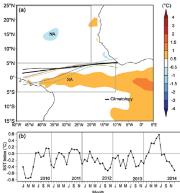
FIG. 4.16. (a) Atlantic ITCZ position inferred from outgoing longwave radiation during May 2014. The colored thin lines indicate the approximate position for the six pentads of the month. The black thick line indicates the Atlantic ITCZ climatological position. The SST anomalies for May 2014 based on the 1982–2013 climatology are shaded ( ^{\circ}\text{C} ). The two boxes indicate the areas used for the calculation of the Atlantic index in (b). (b) Monthly SST anomaly time series averaged over the South American sector (SA region, 10^{\circ} – 50^{\circ}\text{W} , 5^{\circ}\text{S} – 5^{\circ}\text{N} ) minus the SST anomaly time series averaged over the North Atlantic sector (NA region, 20^{\circ} – 50^{\circ}\text{W} , 5^{\circ} – 25^{\circ}\text{N} ) for the period 2010–14, forming the Atlantic index. The positive phase of the index indicates favorable conditions for enhanced Atlantic ITCZ activity.
