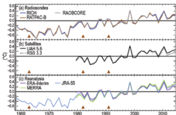
FIG. 2.2. Global average lower tropospheric temperature annual anomalies ( ^{\circ}\text{C} ; 1981–2010 base period) for the MSU 2LT equivalent layer. (a) Radiosondes: RATPAC (Free et al. 2005; 85 stations), RAOBCORE (Haimberger et al. 2012; 1184 stations) and RICH (Haimberger et al. 2012; 1184 stations). (b) Satellites: UAHv5.6 (Christy et al. 2011) and RSSv3.3 (Mears and Wentz 2009). (c) Reanalyses: ERA-Interim, MERRA, and JRA-55 are shown as described in Fig. 2.1. Major volcanic eruptions which cause 2–3 year cooling episodes are indicated by triangles in 1963, 1982, and 1991.
