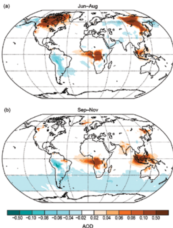
FIG. 2.40. Carbonaceous aerosol optical depth (AOD) anomalies for (a) Jun–Aug 2014 and (b) Sep–Nov 2014, from the MACC reanalysis.
