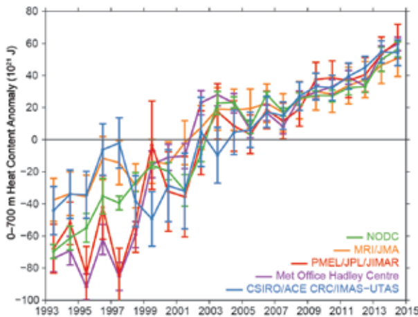
Centre estimate is computed from gridded monthly temperature anomalies (relative to 1950–2014) calculated from EN4.0.2 (Good et al. 2013) data following Palmer et al. (2007). An updated version of the instrument bias corrections of Gouretski and Reseghetti (2010) is applied. Uncertainty estimates follow Palmer and Brohan (2011). For comparison, all estimates have been individually offset (vertically on the plot), first to their individual 2005–14 means (the best sampled time period), and then to their collective 1993–2014 mean (the record length).
