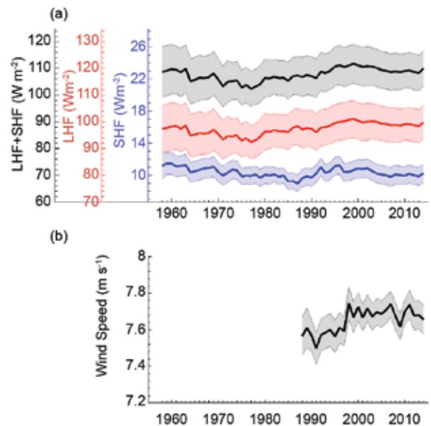
FIG. 3.10. (a) Year-to-year variations of globally averaged annual mean latent plus sensible heat flux ( LHF + SHF ; black curve), latent heat flux ( LHF ; red curve), and sensible heat flux ( SHF ; blue curve). (b) Year-to-year variations of globally averaged annual mean wind speed. Shaded areas indicate fluxes and wind speed estimate uncertainties at the 95% confidence level.
