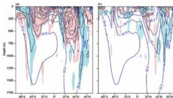
FIG. 3.15. Zonally averaged (a) 2014 salinity anomaly and (b) 2014 minus 2013 salinity field for the Atlantic Ocean. Details follow Fig. 3.14.
