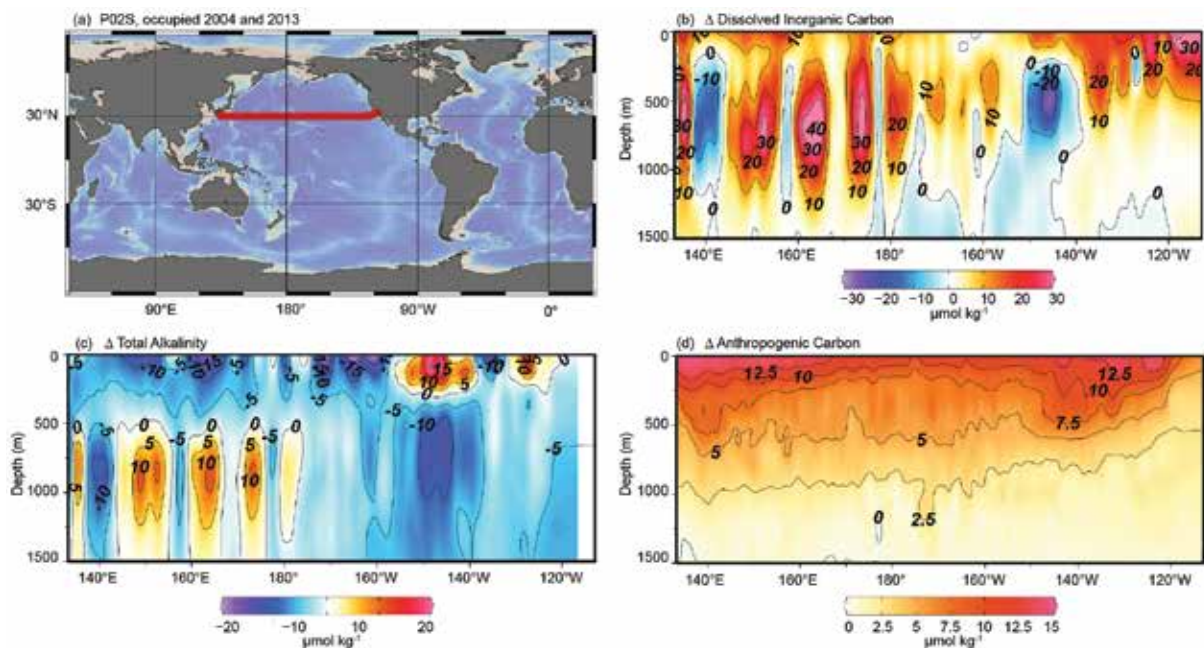
FIG. 3.33. (a) Location (red line) of WOCE hydrographic section P02 repeats. Vertical-zonal sections of 2013 minus 2004 changes in (b) total dissolved inorganic carbon ( C_T ) concentrations, (c) total alkalinity concentrations, and (d) anthropogenic carbon ( C_{Anth} ) concentrations for P02 (in \mu\text{mol kg}^{-1} ).
