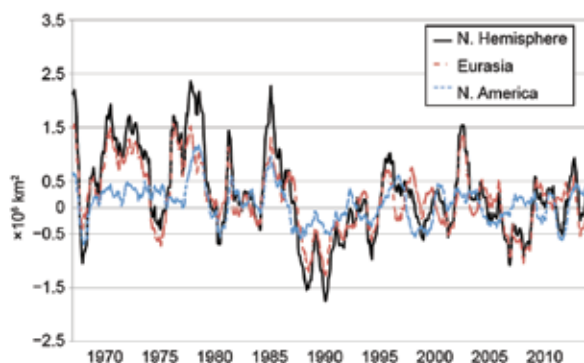
FIG. 2.9. Twelve-month running anomalies of monthly snow cover extent ( \times 10^6 km 2 ) over Northern Hemisphere lands as a whole, Eurasia, and North America (including Greenland) separately between Nov 1966 and Dec 2014. Anomalies are calculated from NOAA snow maps. Mean hemispheric snow extent is 25.1 \times 10^6 km 2 for the full period of record. Monthly means for the period of record are used for 9 missing months between 1968 and 1971 in order to create a continuous series of running means. Missing months fall between June and October, no winter months are missing.
