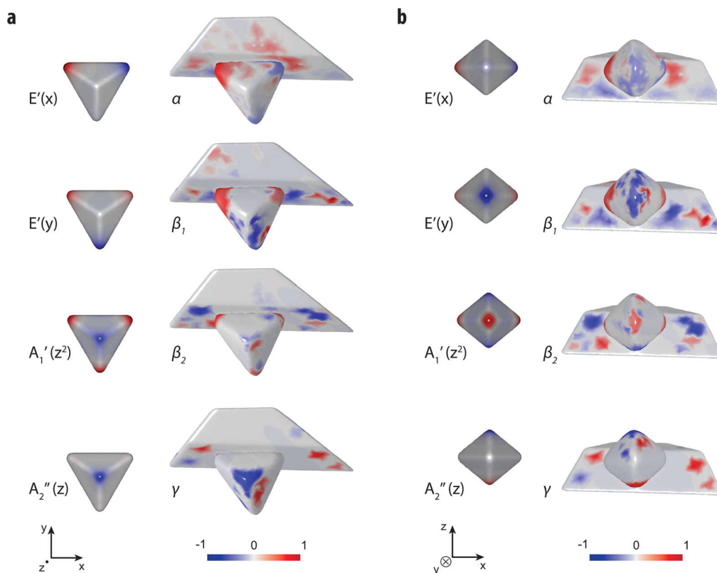
Figure 5. Corner eigenmodes and corresponding surface charge reconstructions for a silver right bipyramid on a \text{MoO}_3 dielectric substrate. (a, b) For each eigenmode, one orientation along the C_3(z) axis of the bipyramid (a) and one perpendicular orientation (b) are shown corresponding to the indicated coordinate axes. The color scale is normalized for each mode. Greek letters refer to the corresponding spectral features as in Figures 1 and 2. Symmetry labels are given for an isolated bipyramid ( D_{3h} point group).
