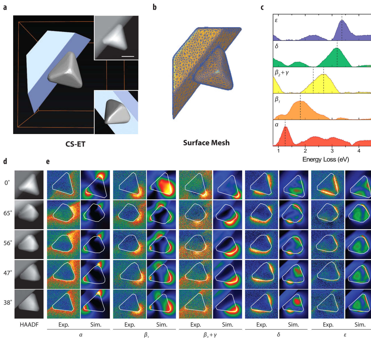
Figure 2. Electron tomography and tilt-series EELS of the surface plasmon modes of a silver right bipyramid on a \text{MoO}_3 substrate. (a) Surface representation of a compressed sensing electron tomography (CS-ET) reconstruction from tilt-series high angle annular dark field (HAADF) STEM. Insets show the 0^\circ tilt HAADF micrograph and a plan-view perspective of the right bipyramid. The inset scale bar is 25 nm. (b) Surface mesh derived from the CS-ET reconstruction used for simulations in (e). (c) Spectral NMF decomposition factors for tilt-series EELS spectrum imaging corresponding to surface plasmon mode excitations of the bipyramid. Dashed vertical lines serve as a guide to the surface plasmon mode resonance energies. (d) HAADF micrographs at tilts recorded simultaneously with the EELS spectrum imaging. (e) Experimental NMF component maps and simulated loss probability maps at the corresponding tilt angles. Intensities are plotted on a normalized scale within each column. Greek letters denote spectral features and associated modal components as in Figure 1.
