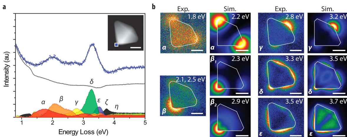
Figure 1. Plan-view EELS spectrum imaging of a silver right bipyramid. (a) Non-negative matrix factorization (NMF) of EELS for a selected area (blue square, inset). The decomposition is shown for a 4.3 \text{ nm} \times 4.3 \text{ nm} ( 9 \text{ pixel} \times 9 \text{ pixel} ) region. Blue dots represent the summed raw spectra, the black line is the sum of all decomposition components, the gray line corresponds to the spectral signature of the zero loss peak (ZLP), and each of the remaining components corresponds to a spatial map that exhibits a dominant contribution matching a surface plasmon mode of the bipyramid ( \alpha – \epsilon ), the bulk plasmon ( \zeta ), or the \text{MoO}_3 substrate band edge ( \eta ). (b) NMF component maps (Exp.) and simulated energy loss probability maps (Sim.). Intensities are plotted on a normalized scale for each map. Subscripts on \beta denote fully resolved peaks in simulated spectra represented in the single experimental NMF component \beta . Energies refer to peak maxima in the respective experimental and simulated spectra. Scale bars are 25 nm.
