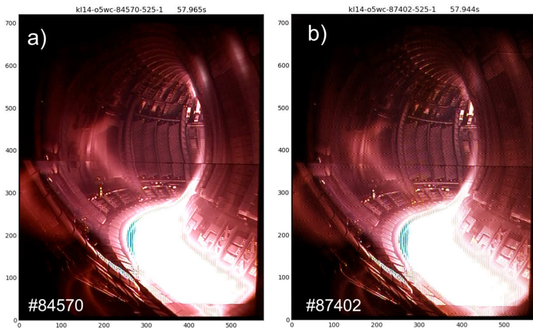
Figure 5: Two images taken by the colour cameras a) directly after the installation of the wide angle KL14 video systems (#84570) and b) at the end of the experimental campaign (#87402). Qualitatively no degradation of the picture can be observed, which is in line with results from quantitative comparisons at various key image areas (see Figure 4).
