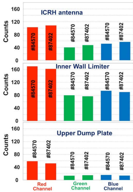
Figure 4: Comparison of the colours channels of the colour camera for two monitoring pulses: directly after the installation of the wide angle KL14 video systems (#84570) and at the end of the experimental campaign (#87402).
