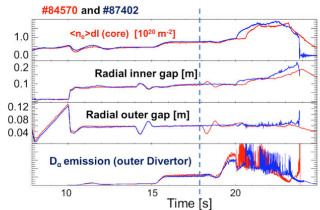
Figure 3: Time evolution of typical monitoring L-mode discharges which correspond to the next figure 5.
