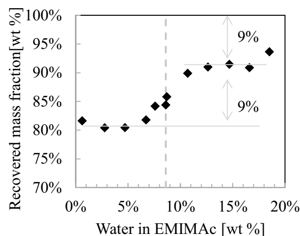
Fig. 3 Recovered mass fraction after pretreatment of beech wood in EMIMAc/water mixtures. The dashed line indicates the transition center at 8.6 wt% water content in EMIMAc. The numbers depict the amount of extracted material at the two plateaus
