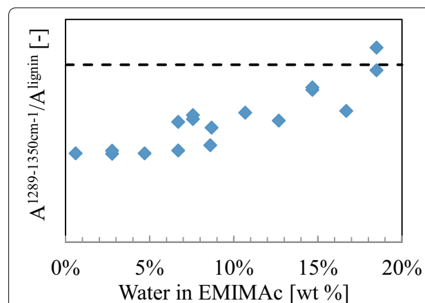
Fig. 4 Semi-quantitative concentration of functional groups from Raman spectra. The areas were calculated to depict the relative change of functional groups. The dashed line shows the average value obtained with native beech wood
