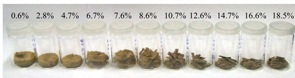
Fig. 1 Morphology of beech chips pretreated in EMIMAc-water mixtures. The water mass fraction increases from left to right as indicated above the samples. While the material is completely disintegrated at low water content, it retains the original morphology at highest water content
