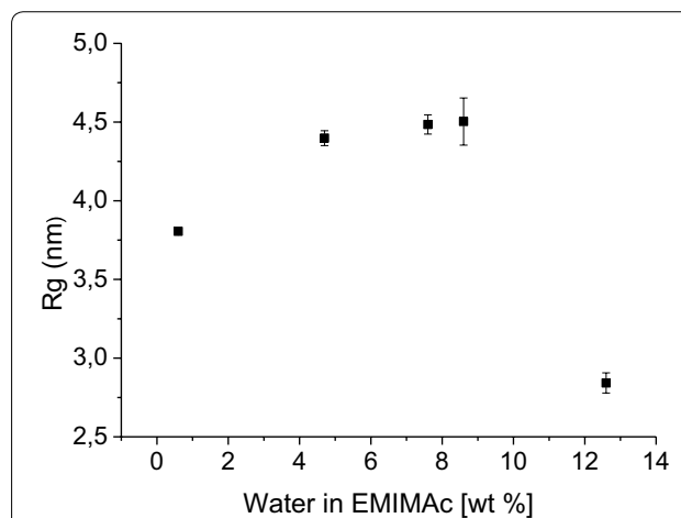
Fig. 8 Radii of gyration ( R_g ) of cellulose fibrils as a function of the water content of EMIMAc during the disintegration process. The radii are larger in the disintegrated samples than those in the sample at 12.6 wt% water content during pretreatment and seem to decrease after processing in concentrated EMIMAc
