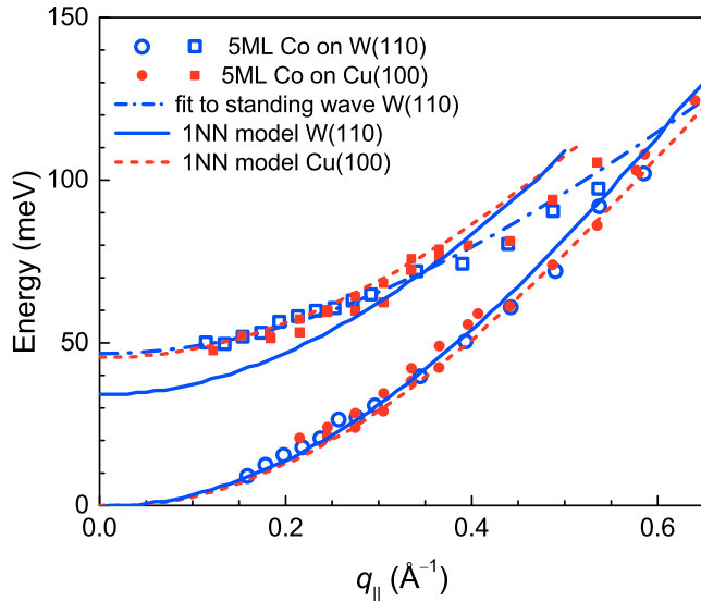
FIG. 16. (Color online) Comparison of the dispersion of 5ML hcp Co(0001) films on W(110) (blue open symbols) and fcc Co(100) films on Cu(100) (red solid symbols) along the \bar{\Gamma}\bar{K} and \bar{\Gamma}\bar{X} directions of the Brillouin, respectively. The solid and dashed lines are calculated within the nearest-neighbor Heisenberg model with J = 15 meV for hcp and fcc films, respectively. The dash-dotted line is a fit to the experimental data on W(110) as described earlier.
