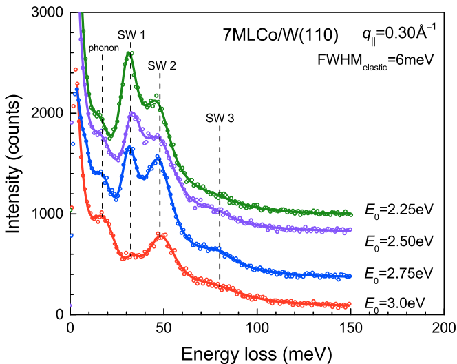
FIG. 7. (Color online) Energy loss spectra as function of the electron impact energy for a 7ML cobalt film at q_{||} = 0.30 \text{ \AA}^{-1} . The absolute as well as the relative intensities of the various spin wave signals depend critically on the impact energy.
