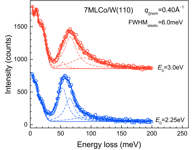
FIG. 8. (Color online) Two energy loss spectra for a 7ML cobalt film at q_{||} = 0.40 \text{ \AA}^{-1} taken with two different electron impact energies, 2.25 eV and 3.0 eV.
