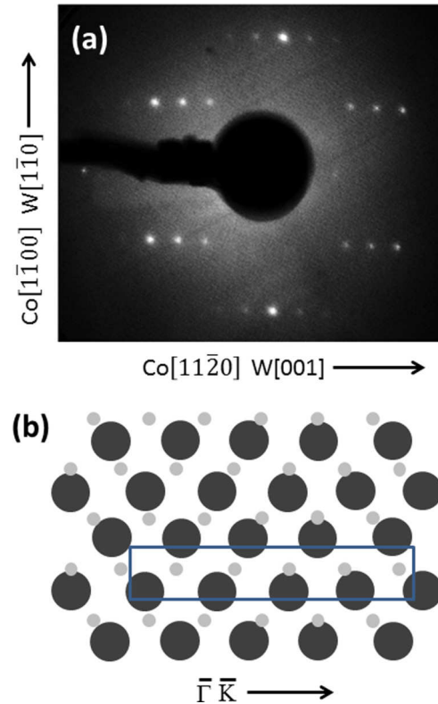
FIG. 4. (Color online) (a) LEED pattern of a 4ML cobalt film on a W(110) surface. Electron energy is 200 eV. The superstructure is caused by the misfit along the W[001] direction. (b) real-space illustration of the W(110) surface (large black spheres) and a single layer of cobalt (small gray spheres). Shown is a 4 \times 1 unit cell, however, the real structure is incommensurate along the W[001] direction.
