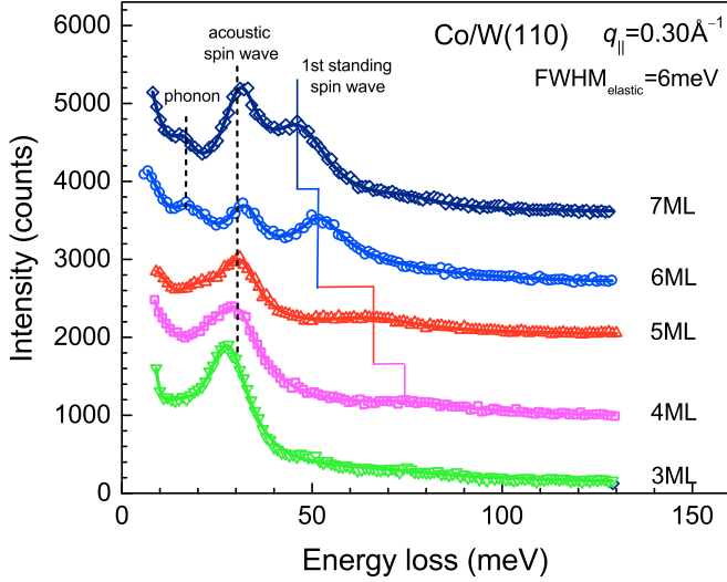
FIG. 6. (Color online) Energy loss spectra for 3–7ML cobalt films at q_{||} = 0.30 \text{ \AA}^{-1} . The impact energy was 3 eV for 2–6ML and 2.25 eV for 7ML. The lowest spin wave mode at 30 meV is independent of the film thickness. It is therefore assigned to the acoustic mode. The other losses are due to standing spin waves.
