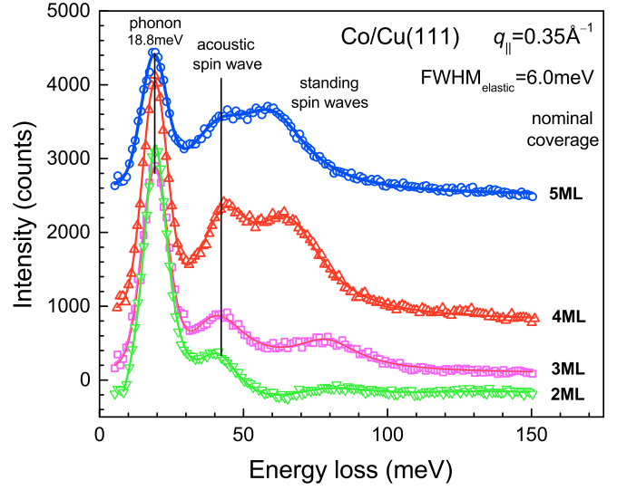
FIG. 11. (Color online) A series of energy loss spectra at wave vector q_{\parallel} = 0.35 \text{ \AA}^{-1} as function of the nominal coverage defined as the coverage in layers, which existed if cobalt were to grow as a continuous pseudomorphic film. The peak at 18.8 meV is due to a phonon resonance as discussed before (see also supporting material). The higher-energy losses are due to spin wave excitations as identified by their dispersion.
