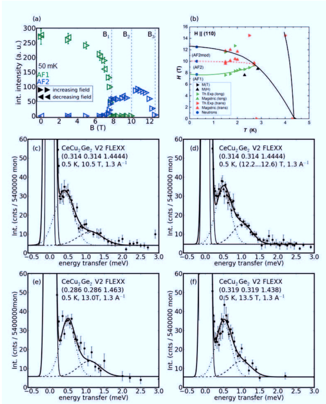
Figure 5: (a): Field dependence of the intensity of the magnetic Bragg peaks in the phases AF1 and AF2. Data are taken from Ref. [13]. (b): Magnetic phase diagram of \text{CeCu}_2\text{Ge}_2 in [110] direction from Ref. [14] (c) and (d): Constant-Q spectra at the \Gamma -point of the magnetic unit cell corresponding to the propagation vector of the phase AF2 in the field region between B_2 and B_3 . In (d) data of spectra obtained at 12.2 T, 12.5 T and 12.6 T are integrated to achieve better statistics. (e) and (f): Constant-Q spectra for the yet unknown phases above 12 T at magnetic fields of 13.0 T and 13.5 T. Data taken V2 FLEXX as indicated in the figures.
