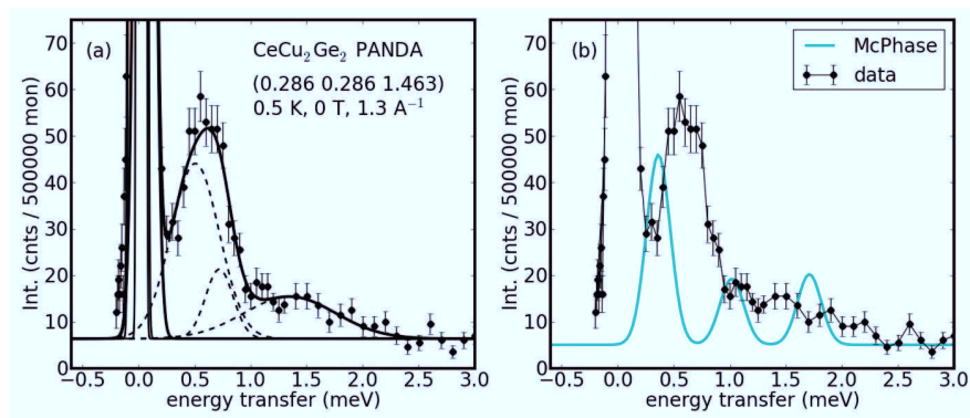
Figure 1: (a) Constant-Q spectra at the \Gamma -point of the magnetic unit cell for the low-field magnetic structure AF1 at zero field. The solid line is a fit using three Gaussians (dashed lines) for the inelastic part. (b) Same INS data as in (a) together with the McPhase calculation for the zero field spin wave spectrum.
