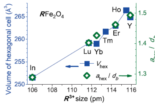
Figure 1.10 \text{R}^{3+} ion size effect on cell volume and ratio of intralayer Fe–Fe distance a_{\text{hex}} to bilayer thickness d_b . Taken from [Angst, 2013].
