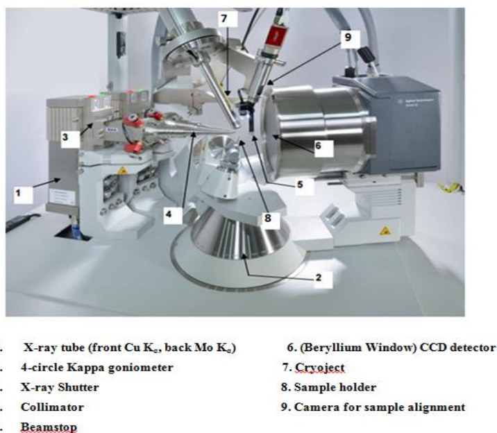
Figure 2.8 Supernova diffractometer. Taken from [Supernova User Manual, 2014].
