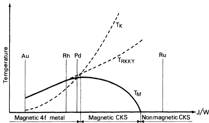
Fig. 1. Tentative classification of the condensed Kondo systems (CKS) according to the relative magnitudes of the two characteristic temperatures T_K and T_{\text{RKKY}} (dashed lines). T_M (solid line) is the magnetic ordering temperature ( T_M \equiv T_N for antiferromagnets, as considered in this paper), J the 4 f -conduction electron exchange integral ( J_{sf} in the text), and W is a scaling factor. Vertical marks correspond to the estimated J/W parameter values for selected \text{CeT}_2\text{Si}_2 systems ( T = \text{Au, Rh, Pd, Ru} ) (taken from Ref. 3).
