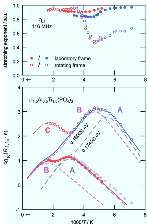
Fig. 3 (bottom) Arrhenius plot of the ^7\text{Li} NMR SLR rates R_1 and R_{1p} of \text{Li}_{1.5}\text{Al}_{0.5}\text{Ti}_{1.5}(\text{PO}_4)_3 investigated in the laboratory (filled circles) and the rotating frame of reference (empty circles), respectively. The resonance frequency was \omega_0/2\pi = 116 \text{ MHz} . The red data points were recorded using a ceramic high-temperature probe, and the blue ones employing a cryoprobe. (top) Stretching exponents corresponding to the NMR SLR rates shown in the lower part of the figure. See the text for further discussion.
