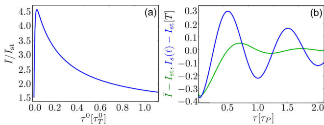
FIG. 11. (Color online) (a) Ratio \bar{I}/\bar{I}_{st} as a function of the duration \tau^0 in units of the electron dwell time \tau_T^0 = 1/I_{st}^0 \approx 4.7 \times 10^4/T . Here \bar{I} is the average current (39) for the pulsing scheme and \bar{I}_{st} is the stationary current obtained if the QD was in the stationary state all the time. The gate voltage V_g = V_g^* = 59.8T is tuned to the resonance and \tau = 2500/T \approx 0.53\tau_P so that a nearly maximal enhancement of the current occurs after the precession. (b) Average current \bar{I} and time-dependent current I_s(t) as function of the pulse time \tau with \tau_P \approx 4.7 \times 10^3/T and \tau^0 = 10/T = 2.1 \times 10^{-3}\tau_P \ll \tau . We subtract the stationary current I_{st} flowing at gate voltage V_g = V_g^* . The results shown in (a) and (b) are computed for a single pulse, N = 1 [ t = \tau^0 + \tau in Eq. (39)], and all other parameters are the same as in Fig. 10.
