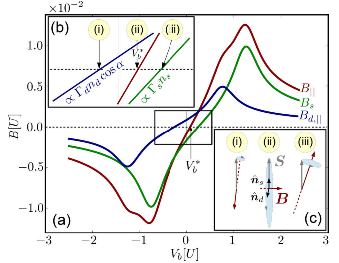
FIG. 3. (Color online) Main panel (a) and sketched zoom-in (b): Exchange field component along \hat{\mathbf{n}}_s from the source electrode ( B_s , green), the drain electrode ( B_{d,\parallel} , blue), and their sum ( B_s + B_{d,\parallel} , red) as a function of V_b for V_g = 0.375U , with other parameters as in Fig. 2. (c) Illustration of the spin precession (gray) for different directions of the exchange field (red), taken for different V_b as indicated in (b). The opening angle is maximal for (ii) at V_b = V_b^* where Eq. (15) holds.
