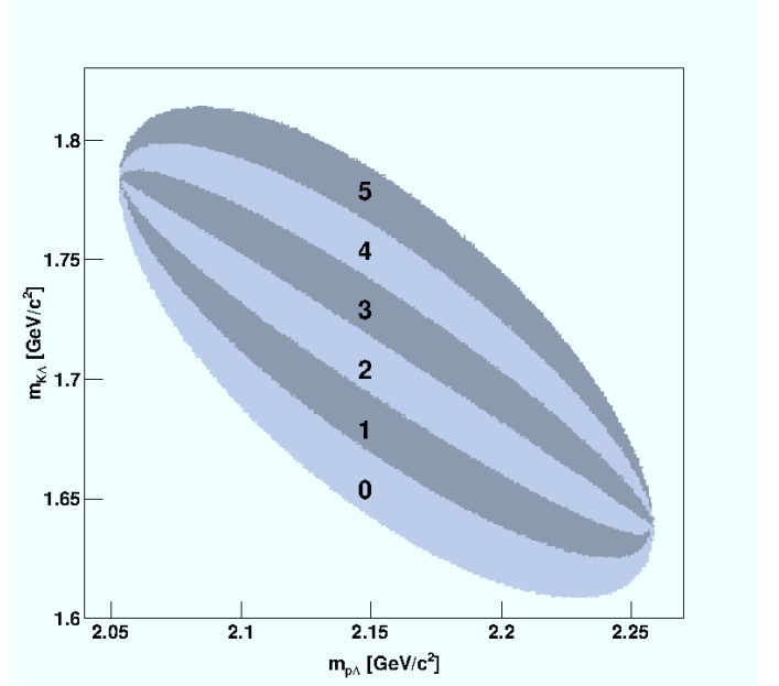
Fig. 11. The division of the Dalitz plot into six slices by selecting ranges of the helicity angle between proton and kaon in the p\Lambda subsystem is shown. If the Dalitz plot is filled according to the phase-space, the projection of the slices i = 0..5 onto the invariant mass p\Lambda results in identical distributions.
