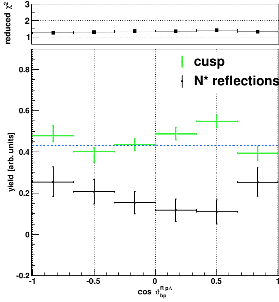
Fig. 14. The height of the cusp (green crosses) and the amount of the reflections at the cusp position (black crosses) for the different regions of \cos \vartheta_{bp}^{R p \Lambda} . The blue dashed line shows the fit result of the height of the cusp of the total data set. As the errors of the fit parameter CT_0 are found to be asymmetric, the errors of the MIGRAD routine of the ROOT [47] program are shown. The upper small figure shows the corresponding reduced \chi^2 of the fit.
