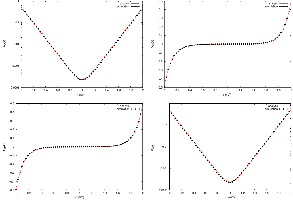
FIG. 12. The matrix of correlators G_{ij}(\tau) for 2-site Hubbard model with \beta = 2 \text{ eV}^{-1} and \kappa = 2.7 \text{ eV} , and U/\kappa = 2 . The solid lines are the analytical results. The points are from a full lattice calculation with N_t = 64 timesteps. Errorbars, obtained via bootstrap, are too small to be visible.
