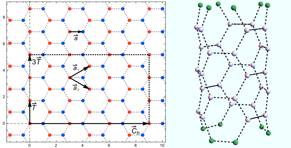
FIG. 1. Construction of nanotubes from a planar hexagonal lattice. The left panel shows the hexagonal lattice from which the tubes are formed. The vectors \vec{T} and \vec{C}_h are shown for the (3,3) chirality. Also shown are the hexagonal unit vectors \vec{a}_1 and \vec{a}_2 . The hexagonal lattice can be described in terms of two triangular lattices A and B (colored red and blue, respectively) shifted by the vector \vec{a} . The rectangle defined by the vectors \vec{C}_h and 3\vec{T} can be cut and rolled along the longitudinal direction to form a nanotube with N_L = 3 , shown in the right panel. The ends of the tube are identified, due to the periodic boundary conditions applied in the longitudinal direction.
