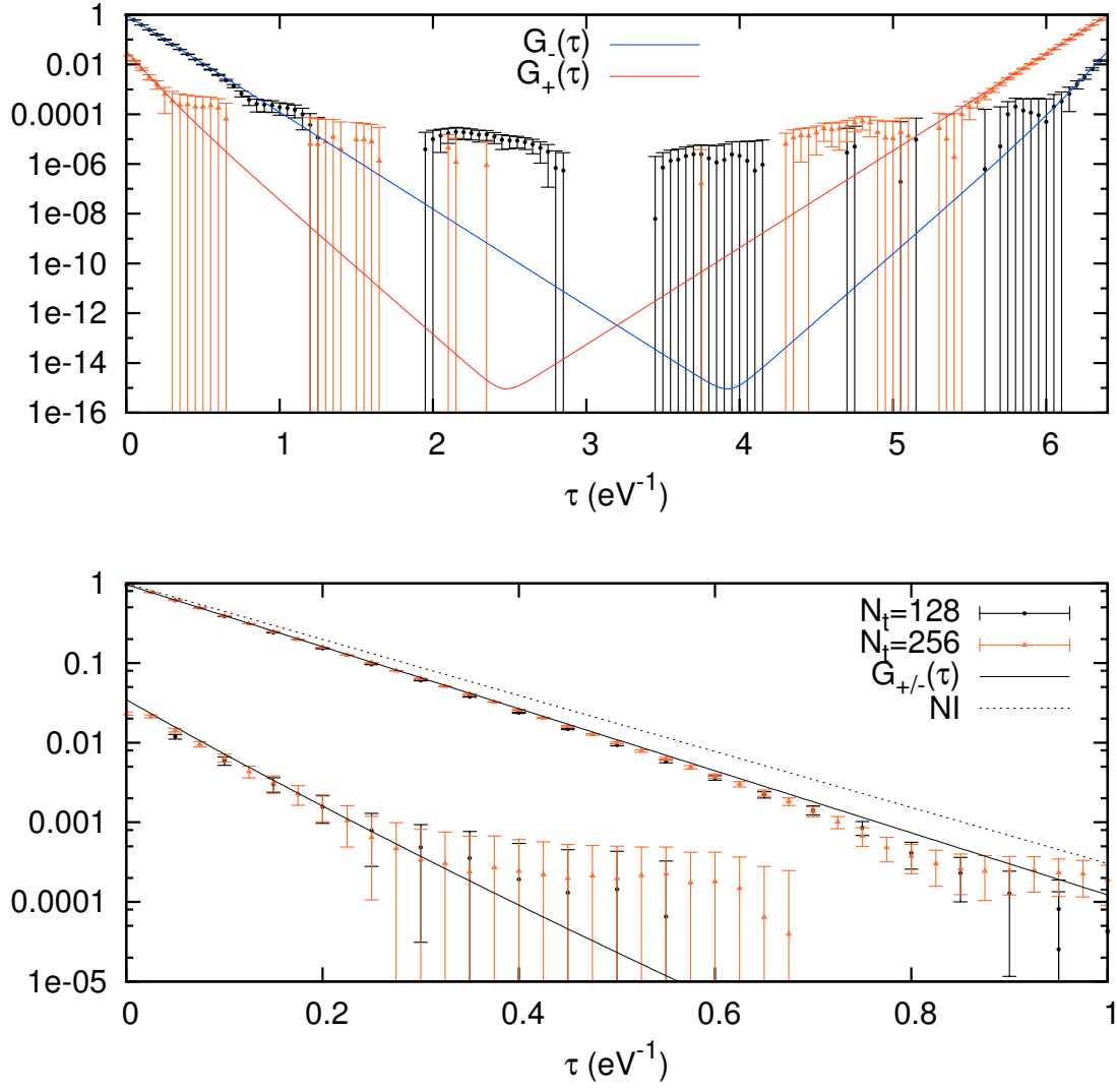
FIG. 15. 4-site Hubbard calculation of \vec{k}_1 momentum correlators with U_{00} = 9.3 eV and \beta = 6.4 \text{eV}^{-1} . Bottom plot is a close up and shows the non-interacting results (dashed line).
