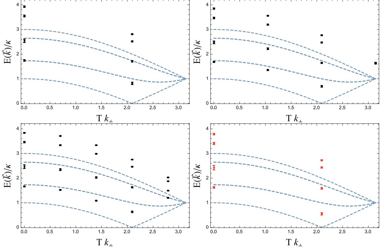
FIG. 11. Continuum-limit extrapolated spectrum of quasi-electron (black points) compared to non-interacting dispersion relation (dashed line) for the (3,3) tube with N_L = 3 (upper left), 6 (upper right), and 9 (bottom left) calculations. The bottom right panel shows the infinite-volume extrapolation of points common to all N_L = 3 , 6, and 9 systems, given by the last column in Table VI.
