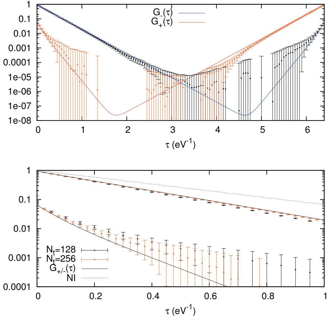
FIG. 16. 4-site Hubbard calculation of \vec{k}_2 momentum correlators with U_{00} = 9.3 eV and \beta = 6.4 \text{eV}^{-1} . Bottom plot is a close up and shows the non-interacting results (dashed line).
