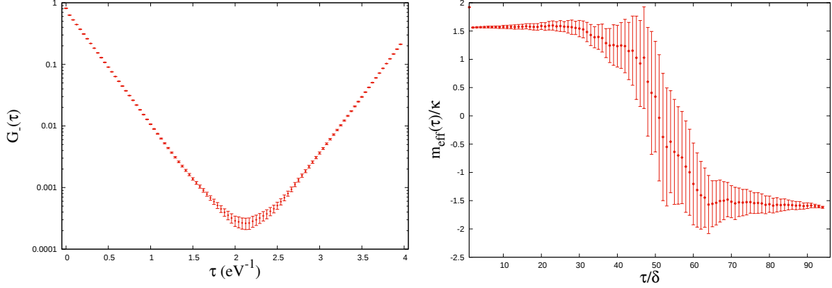
FIG. 5. Example of G_-(\tau) correlator (left panel) with momentum |\vec{T}|(|k_\perp|, |k_{||,i}|) = \left(\frac{2\pi}{3}, \frac{4\pi}{3\sqrt{3}}\right) . The corresponding effective mass plot (in units of hopping parameter \kappa ) is given underneath with \Delta = 2 (right panel). Calculations were performed with N_L = 9 and N_t = 96 .
