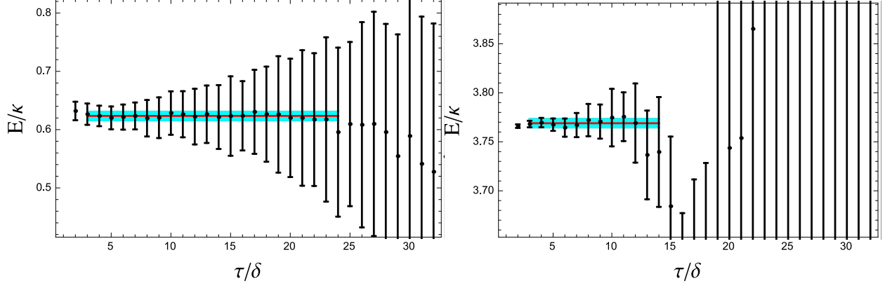
FIG. 7. The extracted energy at the Dirac point (left panel, cyan band) for the N_L = 9 , N_t = 96 calculation using the fitting procedure described in the text. The right panel shows extracted energy at the \Gamma point. The effective mass points are given by the black data points and are shown for comparison. They were not used in the fitting procedure (see text). In both plots, the fitted Gaussian term has been subtracted from the effective mass points.
