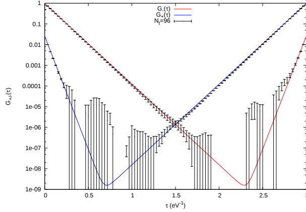
FIG. 14. Comparison of numerical calculation of G_{\pm}(\tau) with analytic result for \beta = 3 \text{ eV}^{-1} , \kappa = 2.7 \text{ eV} , U/\kappa = 4 , and N_t = 96 timesteps. The solid line is the analytic result.
