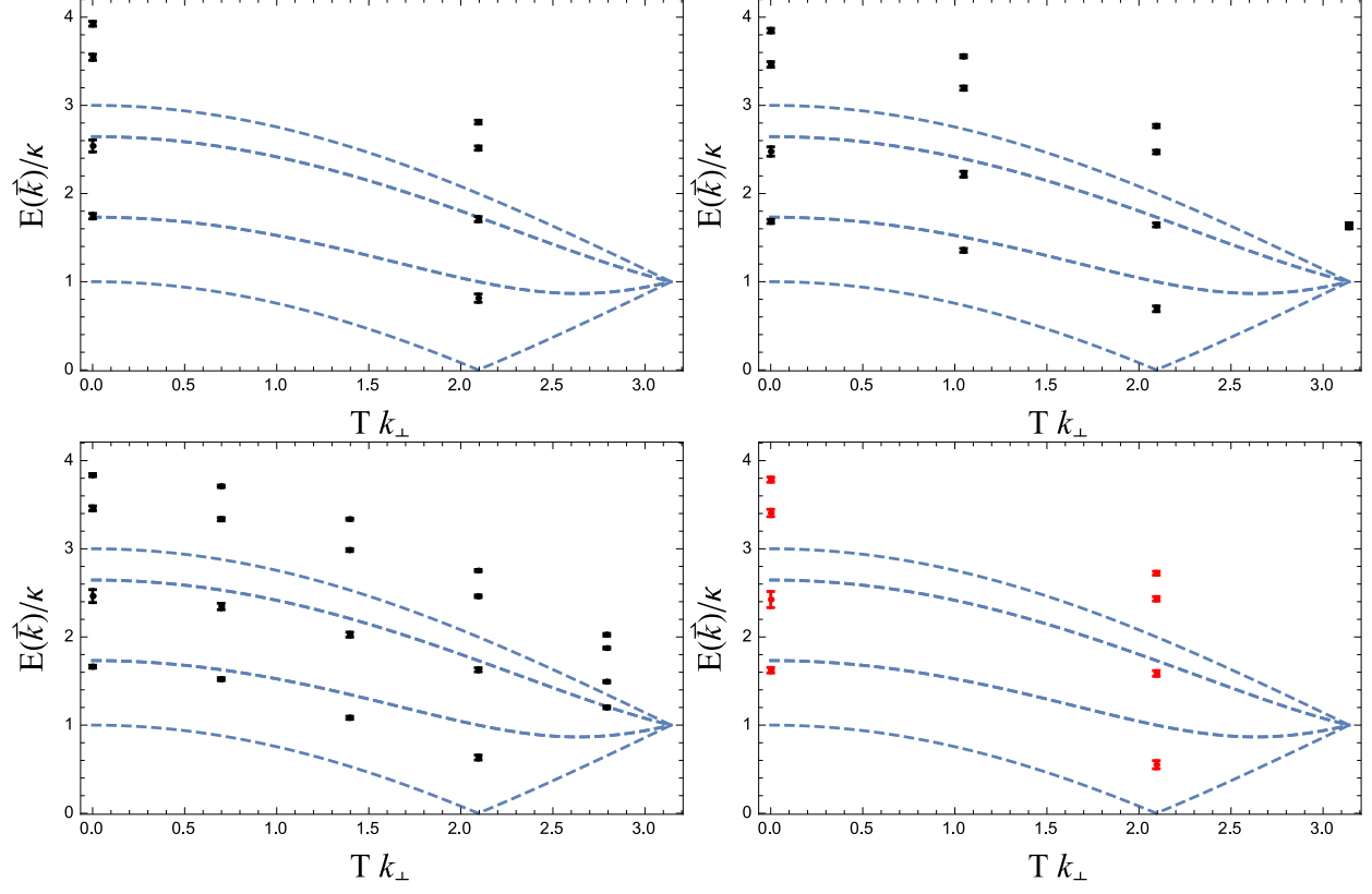
FIG. 11. Continuum-limit extrapolated spectrum of quasi-electron (black points) compared to non-interacting dispersion relation (dashed line) for the (3,3) tube with N_L = 3 (upper left), 6 (upper right), and 9 (bottom left) calculations. The bottom right panel shows the infinite-volume extrapolation of points common to all N_L = 3 , 6, and 9 systems, given by the last column in Table VI.
