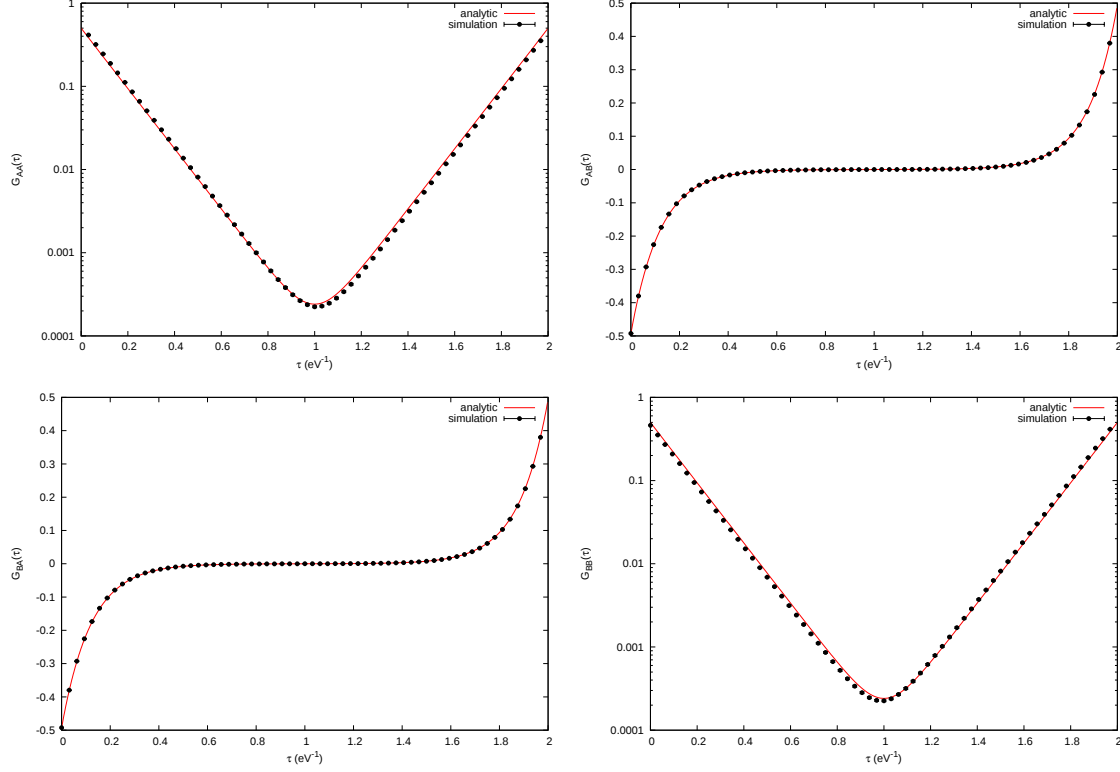
FIG. 12. The matrix of correlators G_{ij}(\tau) for 2-site Hubbard model with \beta = 2 \text{ eV}^{-1} and \kappa = 2.7 \text{ eV} , and U/\kappa = 2 . The solid lines are the analytical results. The points are from a full lattice calculation with N_t = 64 timesteps. Errorbars, obtained via bootstrap, are too small to be visible.
