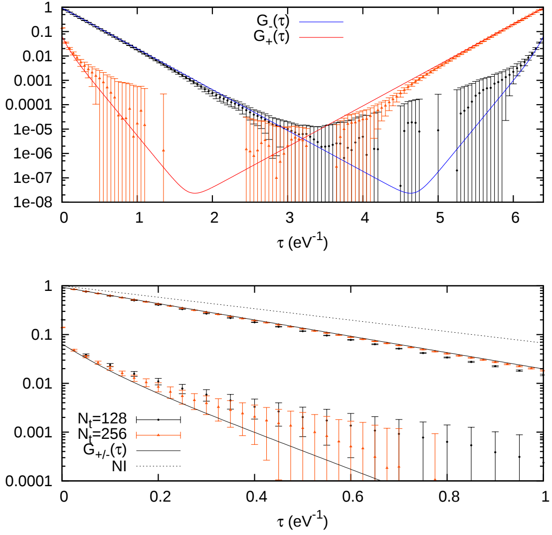
FIG. 16. 4-site Hubbard calculation of \vec{k}_2 momentum correlators with U_{00} = 9.3 eV and \beta = 6.4 \text{eV}^{-1} . Bottom plot is a close up and shows the non-interacting results (dashed line).
