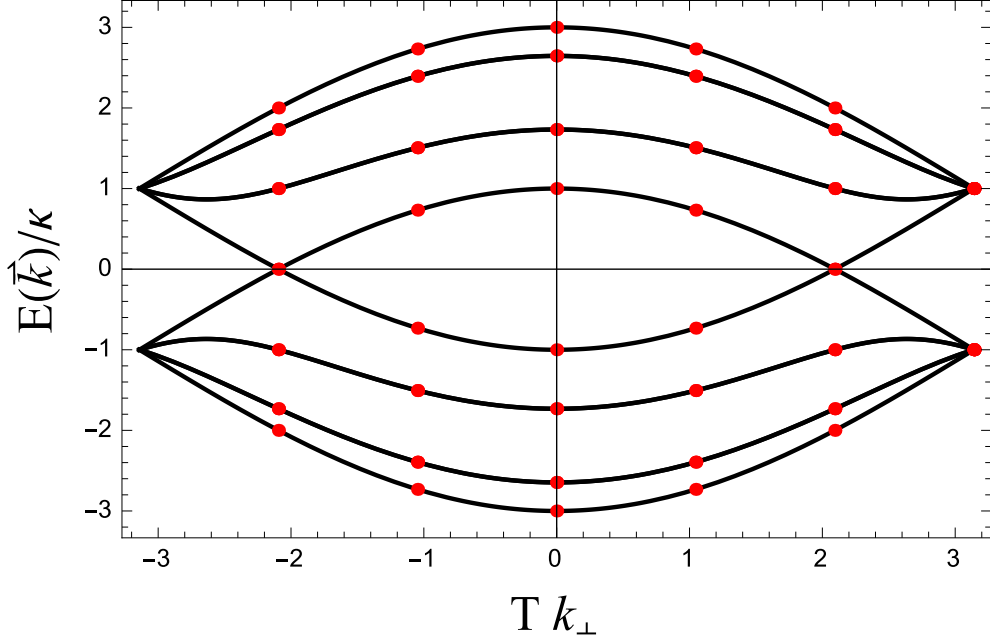
FIG. 2. Non-interacting (tight-binding) dispersion relation for a (3,3) nanotube of infinite length (solid black lines) and one with N_L = 6 unit cells (red points). The abscissa shows the momentum |\vec{T}|k_\perp perpendicular to the tube axis, while the ordinate shows the energy (in units of \kappa ) for a single quasiparticle. Positive energies denote particles, and negative energies denote holes.
