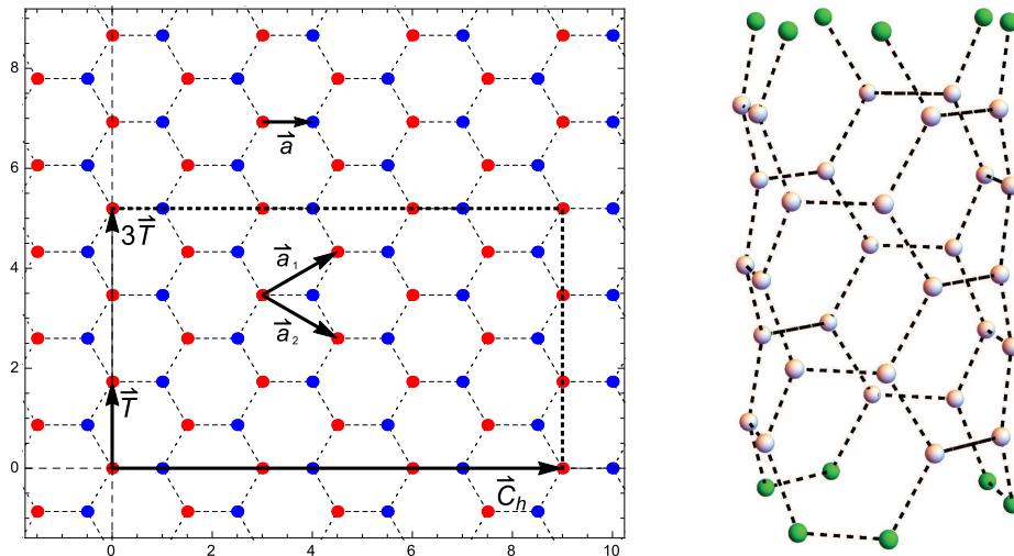
FIG. 1. Construction of nanotubes from a planar hexagonal lattice. The left panel shows the hexagonal lattice from which the tubes are formed. The vectors \vec{T} and \vec{C}_h are shown for the (3,3) chirality. Also shown are the hexagonal unit vectors \vec{a}_1 and \vec{a}_2 . The hexagonal lattice can be described in terms of two triangular lattices A and B (colored red and blue, respectively) shifted by the vector \vec{a} . The rectangle defined by the vectors \vec{C}_h and 3\vec{T} can be cut and rolled along the longitudinal direction to form a nanotube with N_L = 3 , shown in the right panel. The ends of the tube are identified, due to the periodic boundary conditions applied in the longitudinal direction.
