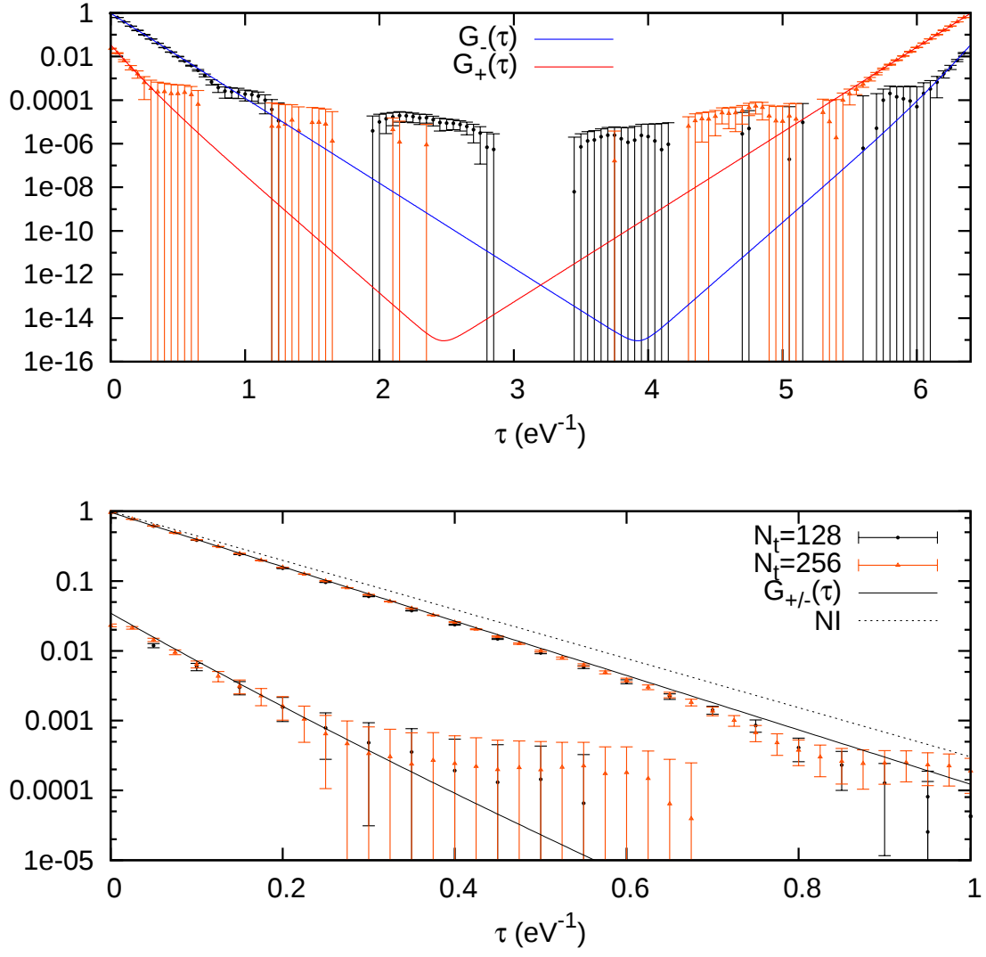
FIG. 15. 4-site Hubbard calculation of \vec{k}_1 momentum correlators with U_{00} = 9.3 eV and \beta = 6.4 \text{eV}^{-1} . Bottom plot is a close up and shows the non-interacting results (dashed line).
