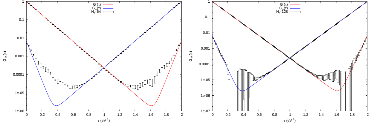
FIG. 13. G_{\pm}(\tau) correlators for 2-site Hubbard model with \beta = 2 \text{ eV}^{-1} and \kappa = 2.7 \text{ eV} , and U/\kappa = 2 . The solid lines are the analytical results. Left (right) plot has N_t = 64 (128) timesteps.
