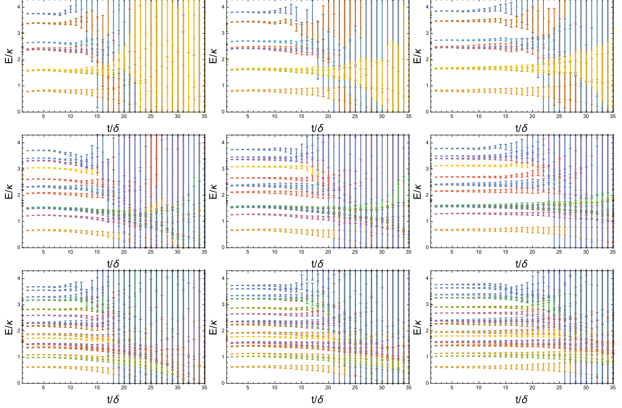
FIG. 9. The effective masses from all accessible momenta points, with Gaussian term subtracted. From top to bottom, the rows label N_L = 3, 6 , and 9 calculations, respectively. From left to right, the columns represent N_t = 64, 80 , and 96 calculations, respectively.
