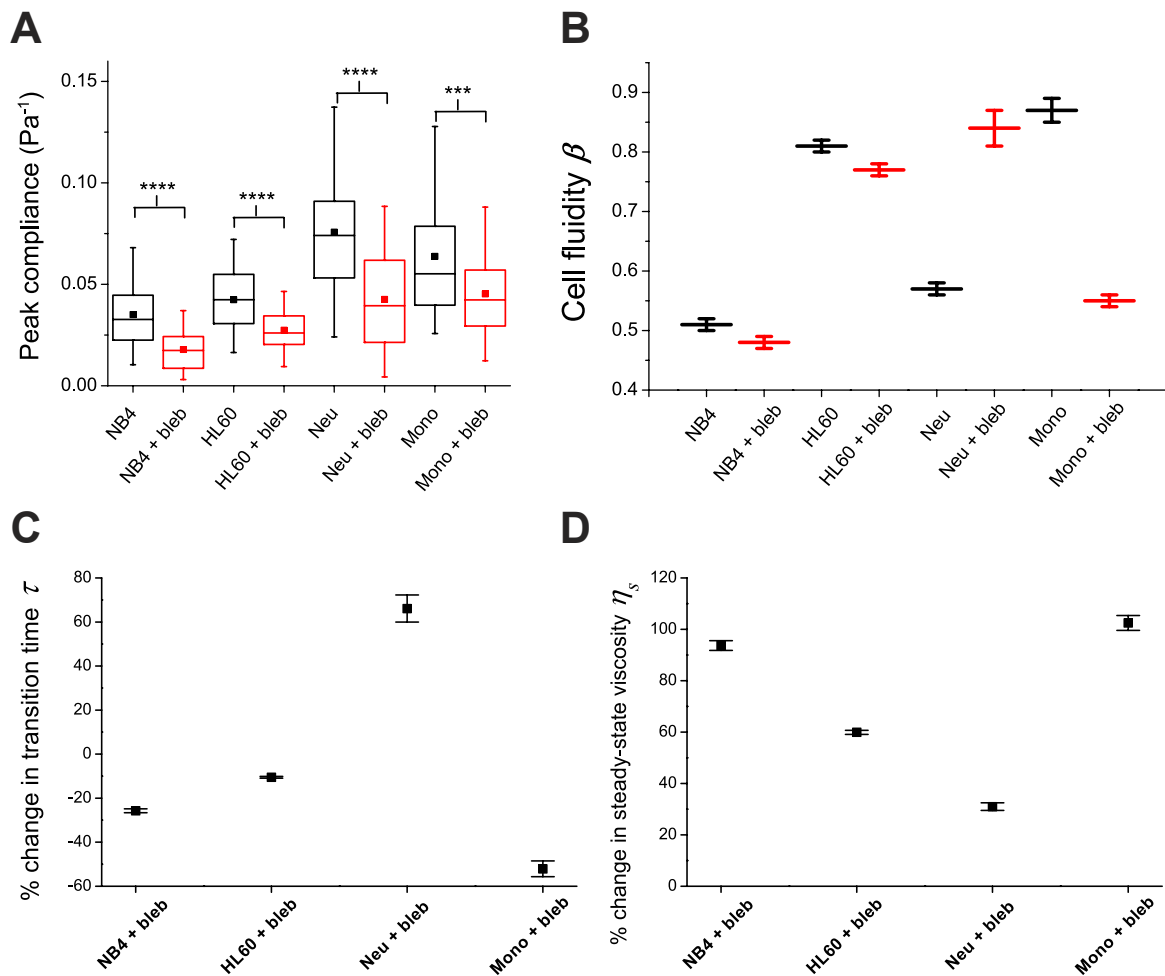
Figure 5: Changes in viscoelastic parameters of naturally suspended cells following myosin inhibition by blebbistatin. A. Box plots of the peak compliance for various cell lines. For all cell lines tested, the peak compliance for blebbistatin-treated cases was significantly lower than for controls. **** p < 0.0001 and *** p < 0.001 . B, C, D. Cell fluidity, % change in transition times, and % change in steady-state viscosity, respectively, for various cell lines treated with blebbistatin compared to their controls. Error bars are standard errors of the fit parameters.
