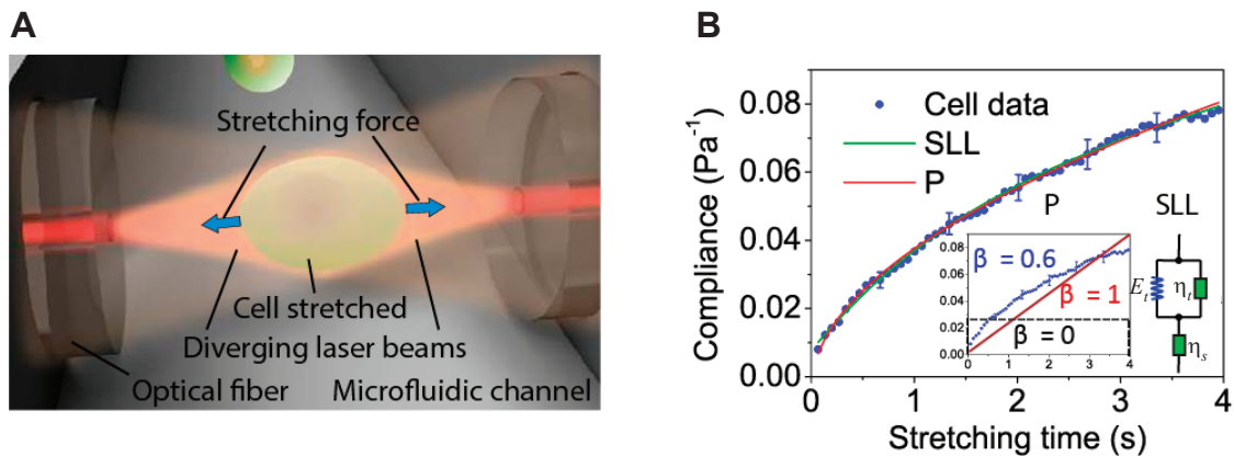
Figure 1: Schematic of an optical stretcher experiment and data analysis. A. Cells flowing through the microfluidic channel are serially trapped and stretched by two diverging, counter-propagating laser beams emanating from single-mode optical fibers. The momentum transfer of light to the surface of the cell results in (mainly axial) optically induced surface stresses, leading to cellular deformation along the optical axis. B. Creep compliance curve for a representative HL60 cell stretched at 0.9 Pa. The creep compliance curve can be fitted to a power law (P) model or a Standard Linear Liquid (SLL) mechanical model. In the power law model, the creep response follows a power law, with \beta = 0 for purely elastic materials, unity for a purely viscous fluid, and 0 < \beta < 1 for viscoelastic materials, such as cells (see inset). The SLL model comprises of the transient elastic ( E_t ) and viscous components ( \eta_t ), and the steady-state viscous component ( \eta_s ).
