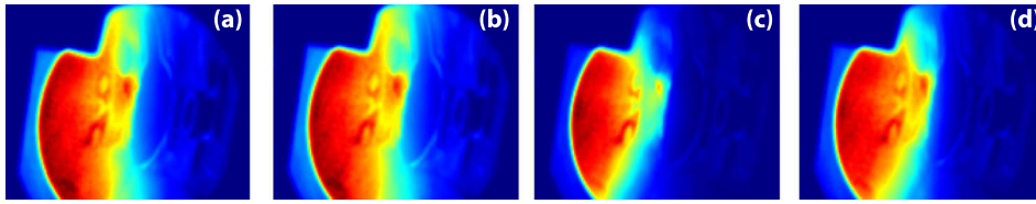
FIG. 6. Temporal evolution of the IR radiation patterns of the discharge No. 119874 taken at (a) t = 2.057 s, (b) t = 2.062 s, (c) t = 2.088 s, and (d) t = 2.093 s. A small red spot at the right field side of the image presents the heated scintillator probe tip.
