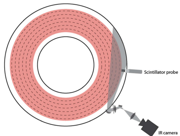
FIG. 1. Schematic top view of experimental setup. Solid black lines indicate the vacuum chamber wall. A gray area represents the field of view of the IR camera. The scintillator probe is placed at the last closed flux surface.
