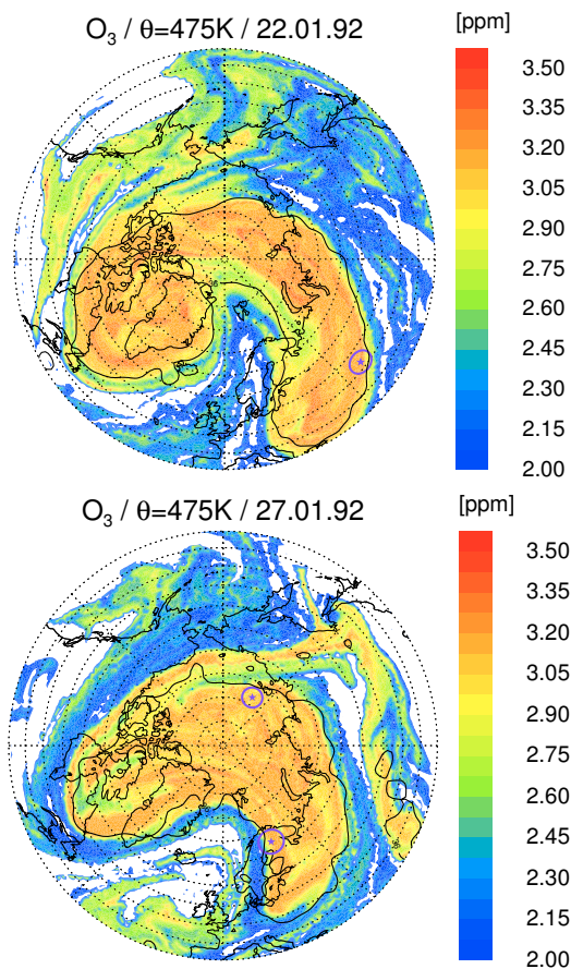
Fig. 2. Simulated ozone mixing ratio for 22 January (top) and 27 January (bottom). The violet stars and circles show the location and Match radius of two individual Match trajectories. The black contour corresponds to the 36 PVU line which is used here as the definition of the vortex edge. White areas indicate ozone mixing ratios below 2 ppm.
