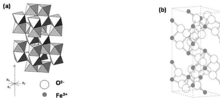
Figure 2.1: (a) HCP structure of hematite. (b) Model of the Unit cell. Images taken from [Cornell, Schwertmann, 2003].
