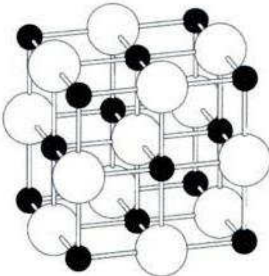
Figure 2.4: Structure of Wustite: Black spheres represent iron- and white spheres oxygen-atoms. Image taken from [Teixeira et al, 2012].
