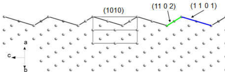
Figure 4.23: Surface reconstruction of sapphire upon annealing.
