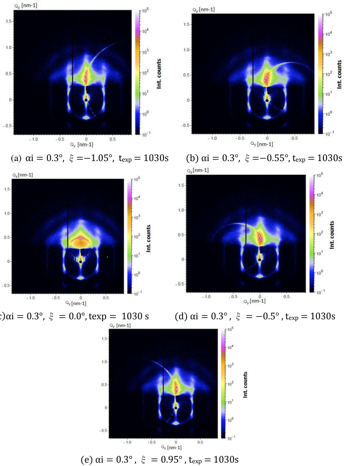
Figure 4.20 : (a, b, c, d) GISAXS pattern of an 20 nm iron oxide nanoparticles deposited on a pre-structured Si wafer, measured at constant incident angles \alpha_i = 0.3^\circ and different \xi angles. \delta = 0.05 . Time of each exposure is 1030s. The period of the gratings is 300nm and depth is 100nm. The ring, which crosses the specular reflection and the primary beam, corresponds to the scattering from Si gratings. The spots correspond to the ordering of nanoparticles.
