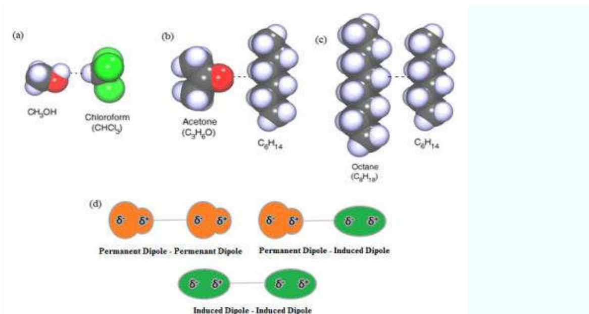
Figure 2.20: (a) Keesom forces. They exist only between polar molecules, (b) Debye force. It arises from the distortion of the charge cloud induced by a polar molecule nearby, (c) London forces, They result from electrostatic attraction between temporary dipoles and induced dipoles caused by movement of electrons; these are attraction forces that operate between all molecules and among isolated atoms in noble gases. (d) Interactions between molecules—temporary and permanent dipoles. Image taken from [Leite et al, 2012].
