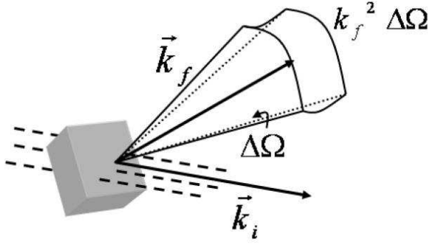
Figure 2.24: The solid angle subtended by the scattered beam at a detector [Nelsen, McMorro, 2011].
