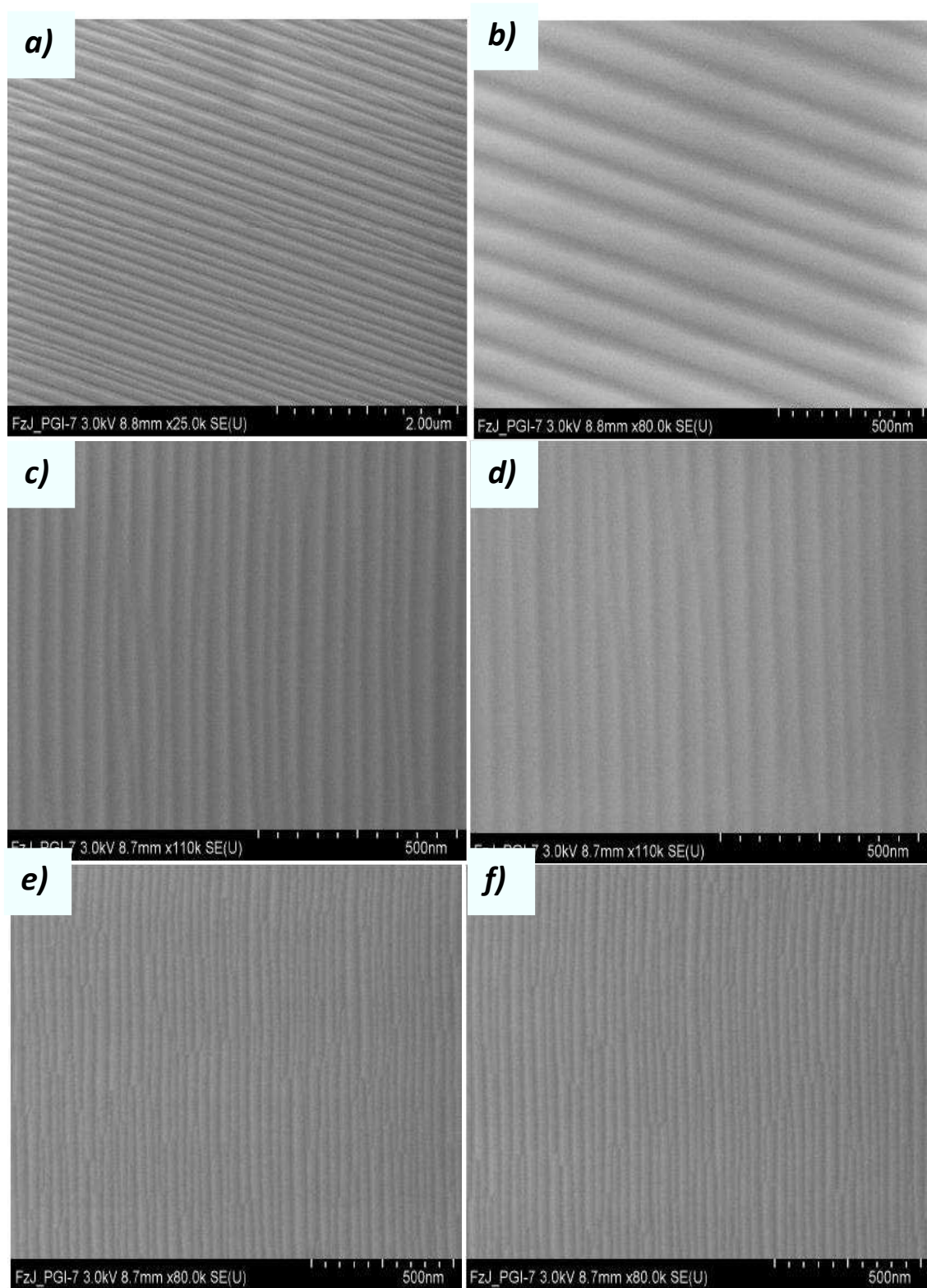
Figure 4.24: SEM image for Sapphire substrate after heat-treatment. a-b) on 1500°C for 24 h . c-d) on 1400°C for 24 h. e-f )on 1300°C for 24 h.
