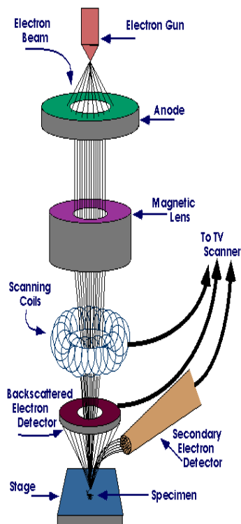
Figure 3.3: a) diagram of scanning electron microscope. Image taken from [Scanning Electron Microscope, 2003] b) principal set-up of an electron optical column: Between the electron gun and the sample holder several electro-optical lenses are mounted to focus the electron beam and set the magnification. Image taken from [Wilbs, 2013].
