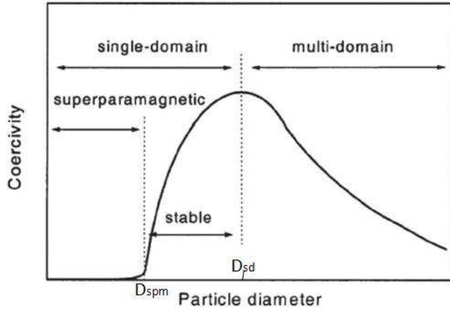
Figure 2.11: Size dependence of coercivity of magnets. Image taken from [Ce et al, 2014].
