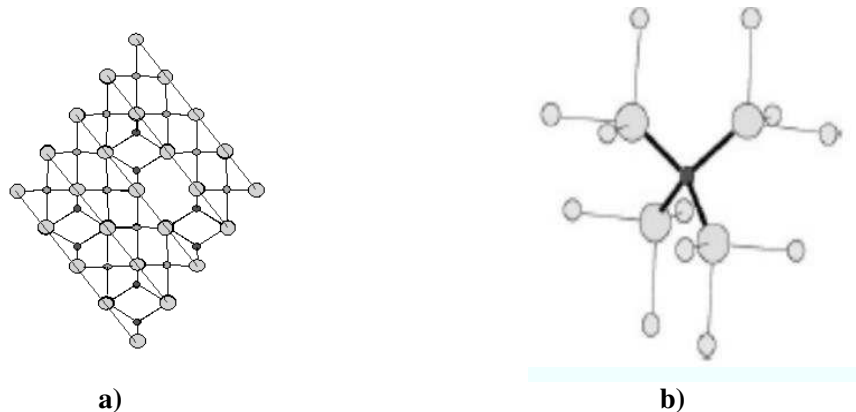
Figure 2.3: Structure of Maghemite: Large spheres represent oxygen- and small spheres iron-atoms. a) Projection of the lattice in the xy-plane. b) unit cell of Maghemite. Images taken from [Cudennec, Lecerf, 2005].
