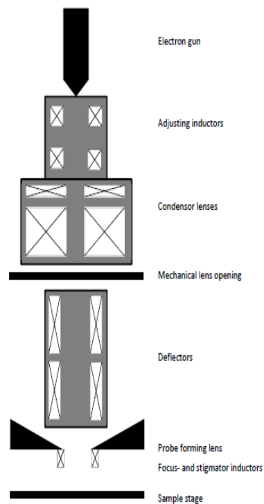
Figure 3.3: a) diagram of scanning electron microscope. Image taken from [Scanning Electron Microscope, 2003] b) principal set-up of an electron optical column: Between the electron gun and the sample holder several electro-optical lenses are mounted to focus the electron beam and set the magnification. Image taken from [Wilbs, 2013].
