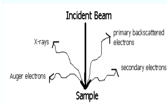
Figure 3.1: beam hits the sample in the SEM, electrons and X-rays are ejected from the sample.
