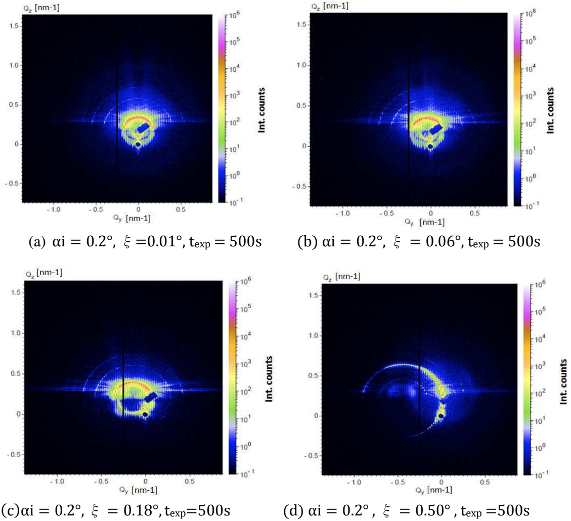
Figure 4.16: (a, b, c, d) GISAXS pattern of a pre-structured Si wafer without nanoparticles, measured at fixed incident angle \alpha_i = 0.2^\circ and variable \xi angles. \delta = 0.0 . Exposure time is 500s. The gratings period is 300nm and depth is 100nm. The ring, which crosses the specular reflection and the primary beam, corresponds to the scattering from Si gratings.
