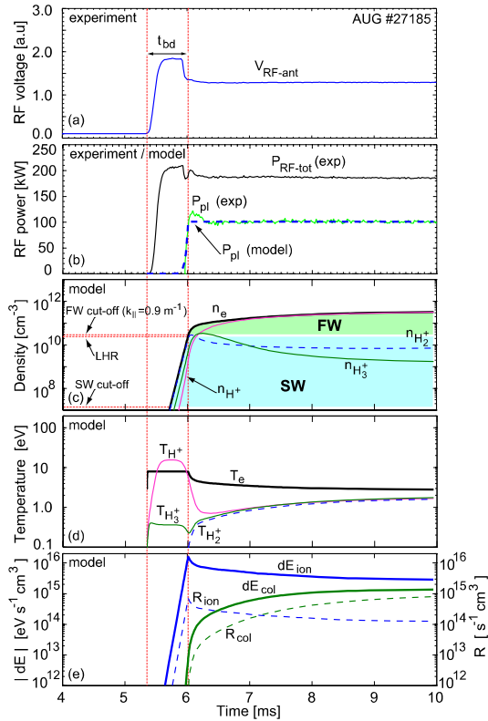
Figure 1. 0-D simulation of the H_2 breakdown with AUG ICRF antenna in monopole phasing (#27185): B_T(0)=2.32 T, p_{H_2}=4.7 \times 10^{-4} mbar, P_{RF-ant}=210 kW, P_{pl}/P_{RF-ant}=0.48 , P_{H^+}=0.01P_{pl} , f=30 MHz, n_{e-bd \text{ model}} \approx 2.8 \times 10^{10} \text{ cm}^{-3} .
