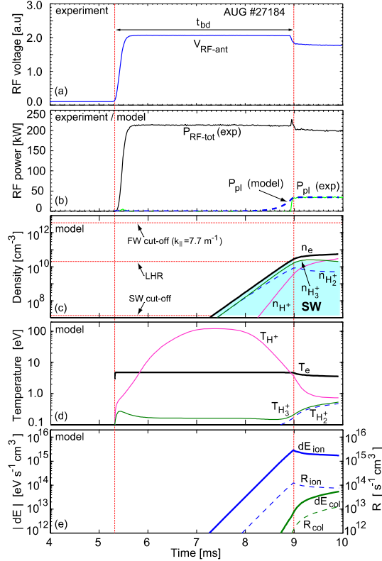
Figure 2. 0-D simulation of the H_2 breakdown with AUG ICRF antenna in dipole phasing (#27184): B_T(0)=2.32 T, p_{H_2}=4.7 \times 10^{-4} mbar, P_{RF-ant}=210 kW, P_{pl}/P_{RF-ant}=0.17 , P_{H^+}=0.03P_{pl} , f=30 MHz, n_{e-bd \text{ model}} \approx 2.7 \times 10^{10} \text{ cm}^{-3} .
