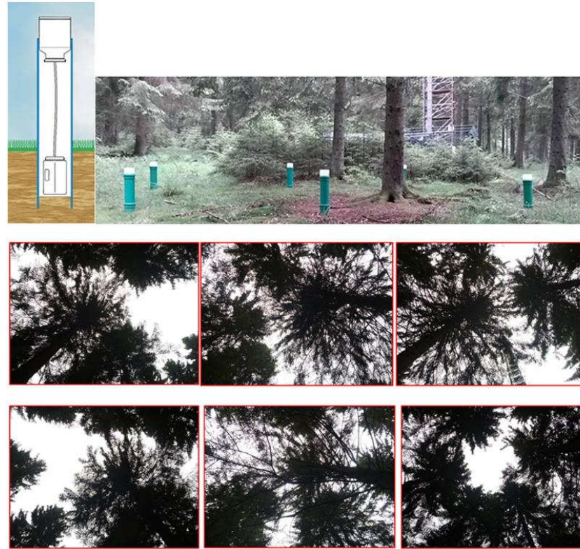
Figure A1. UMS deposition collector RS200 schematic (available at http://www.ums-muc.de ) used as funnel TF samplers with upward view, indicating the covered heterogeneity of the canopy structure.
