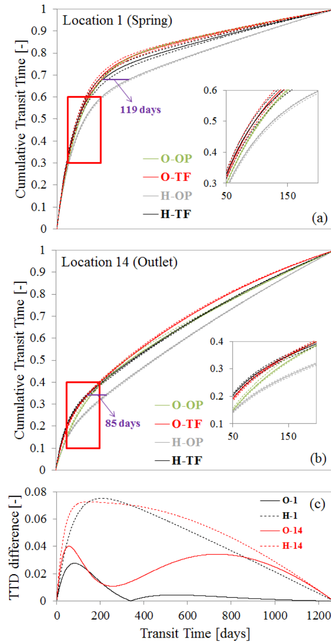
Figure III.3. TTDs derived by using \delta\text{OP} and \delta\text{TF} and isotope tracer data of either \delta^{18}\text{O} (O-OP and O-TF) or \delta^2\text{H} (H-OP and H-TF) for (a) the spring (location 1) and (b) the outlet (location 14).
