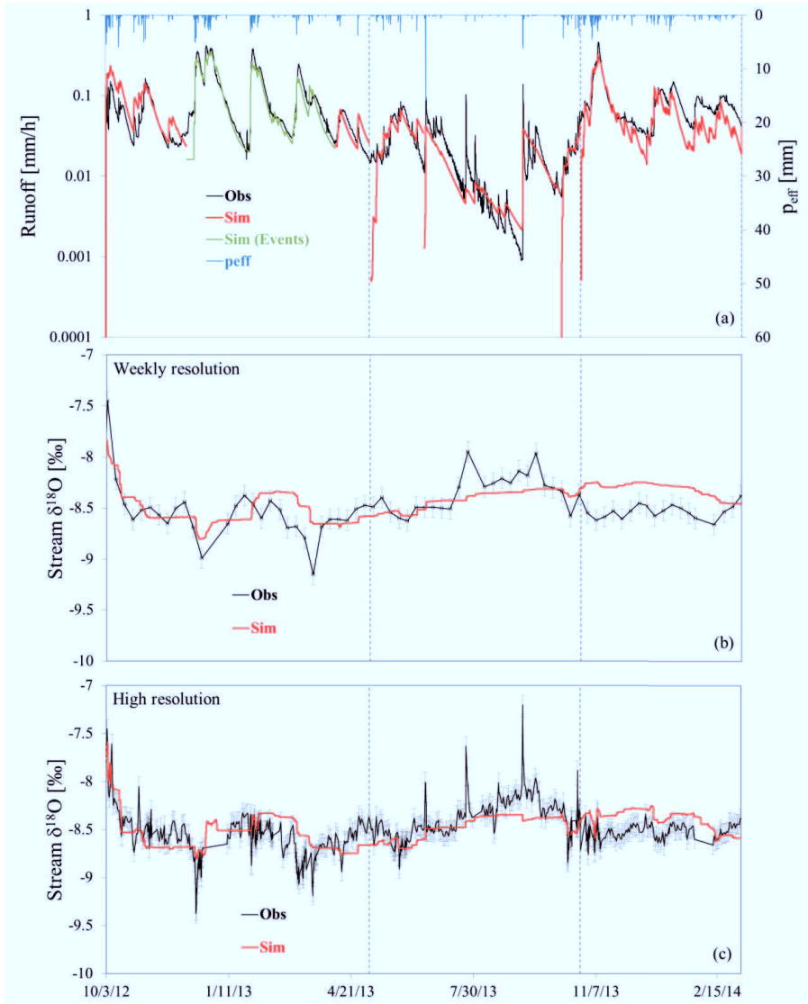
Figure IV.6. (a) Simulated runoff (Sim) with event modeling (Sim (Events)) plotted against observed runoff (Obs). Effective precipitation ( p_{eff} ) is shown as blue bars from the top. (b) and (c) Stream isotope modeling results (Sim) plotted against observed stream isotopes (Obs) using weekly and high temporal resolution. Vertical, dashed grey lines in all panels denote the three modeling periods.
