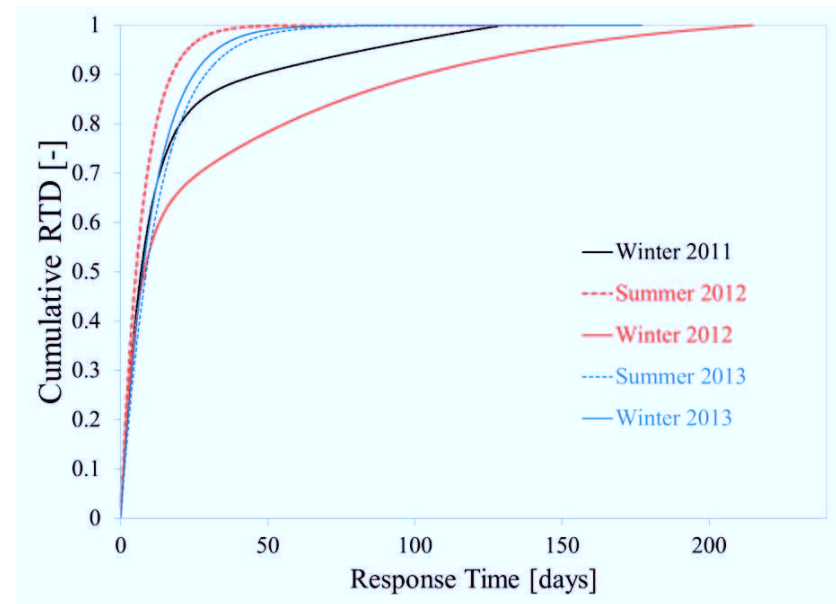
Figure A7. Response Time Distributions of the 3 modeling periods (Winter 2012, Summer 2013 and Winter 2013) and, for reasons of comparison, the year before the modeling period of this study (Winter 2011 and Summer 2012).
