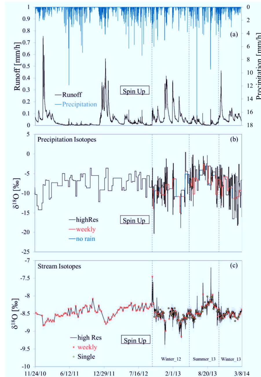
Figure IV.3. Measured and calculated data of the Erkensruhr catchment used for TTD estimation: (a) runoff and precipitation, (b) precipitation isotopes and (c) stream isotopes. Isotopes were measured in high resolution (high Res) and calculated for weekly resolution (weekly), with manually taken stream
