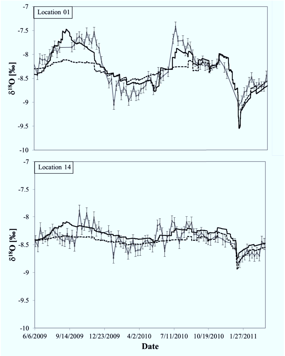
Figure II.7. Stream isotope simulations for (top) location 1 and (bottom) 14. Observed isotope values (gray line with error bars), simulation result with changing active catchment area (black line) and simulation results with 38.5 ha active catchment area throughout the whole modeling period (dashed line). Location 1 with VE = 0.9788 and NSE = 0.74; location 14 with VE = 0.9855 and NSE = 0.34.
