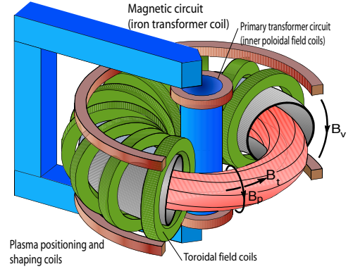
FIG. 5: Schematic diagram of a tokamak.
