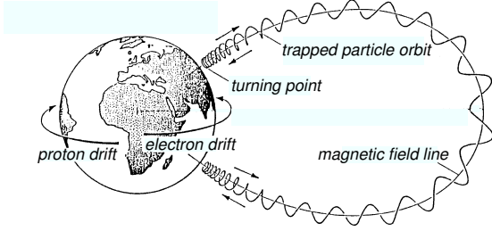
Figure 6: Electron and proton drifts in the Earth magnetic field.
