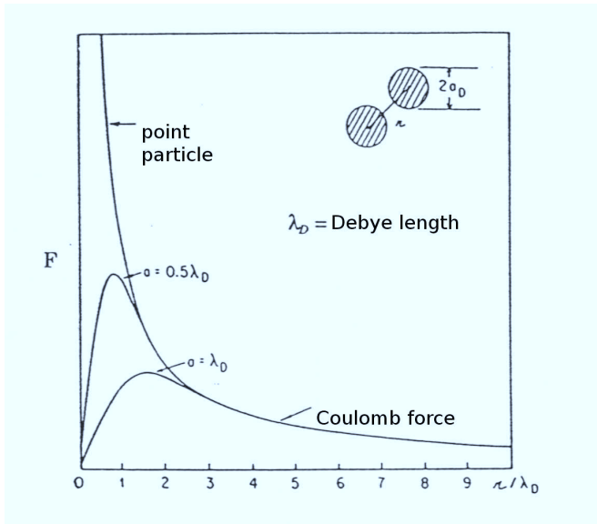
Figure 4: Interactions between finite size particles. Reproduced from [Daw83].
