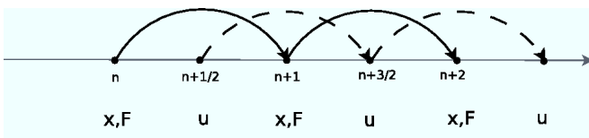
Figure 7: Visual representation of the leap-frog algorithm.
