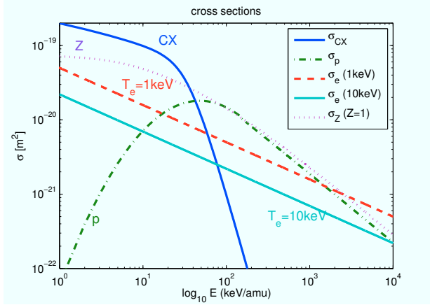
Figure 4: Cross sections for ionization of fast neutrals by charge-exchange (CX), electron impact (for two different electron temperatures T_e = 1\text{keV} and 10\text{keV} ), and by proton impact (p). The curve Z is the normalized \tilde{\sigma} for impurities.
