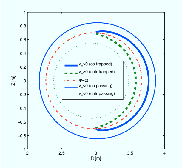
Figure 3: Poloidal projection of the drift trajectories of beam ions for perpendicular injection (trapped trajectory) and for parallel co- and counter-injection for common toroidal angular momentum and energy; 'co' and 'counter' are defined w.r.t. the plasma current. Also the magnetic surface on which the banana tips lie is depicted.
