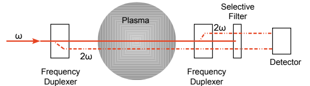
Figure 3: Principle scheme of a dispersion interferometer from [7].
