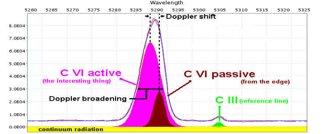
Figure 5: Typical carbon spectrum of the TEXTOR Charge Exchange Recombination System. The measured line originated from C^{5+}(n = 8 \rightarrow n = 7) at \lambda = 529\text{nm} . Without the neutral beam, only a passive line originating from the plasma edge is observed. When the beam is switched on the active component appears: its width being representative of the carbon temperature, its Doppler shift is related to the ion rotation along the line of sight and the intensity is a measure of the carbon density.
