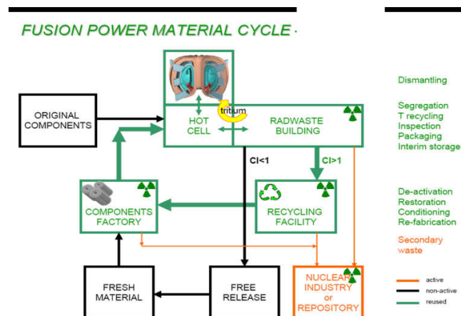
Figure 9: Fusion power potential material cycle [11]
