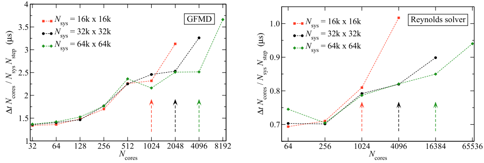
Figure 1. Strong scaling test of GFMD simulations (left) and the Reynolds solver (right) run on JUQUEEN for system sizes of N_{\text{sys}} = 16, 384^2, 32, 768^2 , and 65,536^2 . The abscissae correspond to the number of MPI ranks, N_{\text{cores}} , while the ordinates show the extrapolated time it would take one core to propagate one grid point by one time step. Here, \Delta t stands for the wall-clock time and N_{\text{step}} for the number of time steps or iterations. The arrows indicate a stripe width of 16 (for GFMD), and 512 \times 512 grid points per process (Reynolds).
