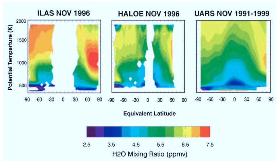
Figure 9. November water vapor monthly mean in PV-based equivalent latitude and potential temperature coordinates derived from ILAS 1996 measurements (left), HALOE 1996 measurements (center), and the UARS (9 years of 1991–1999) (right). Note the sampling range of HALOE instrument for this month was poleward limited to \sim 60^\circ\text{N} in geographical latitude.
