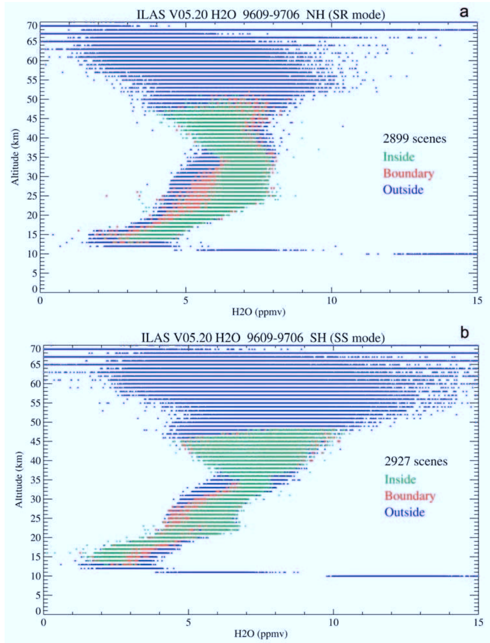
Figure 2. Vertical profiles of all available ILAS version 5.20 water vapor data for the Northern Hemisphere (a), and the Southern Hemisphere (b). Data are categorized into inside (green), boundary (red), and outside (dark blue) of the polar vortex.
