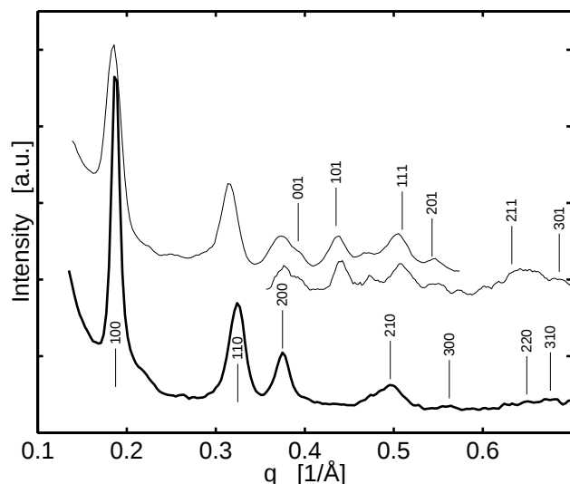
Figure 4 Scattering intensity of dehydrated HFBI on silicon surface. The indexing is according to hexagonal structure with a = b = 38.7 \text{ Å} , c = 16.0 \text{ Å} and \gamma = 120^\circ . The thick curve below is the intensity from the out-of-plane scan and the two upper curves are in-plane scans, lower of which is measured with better angular resolution using a receiving slit of 0.03^\circ .
