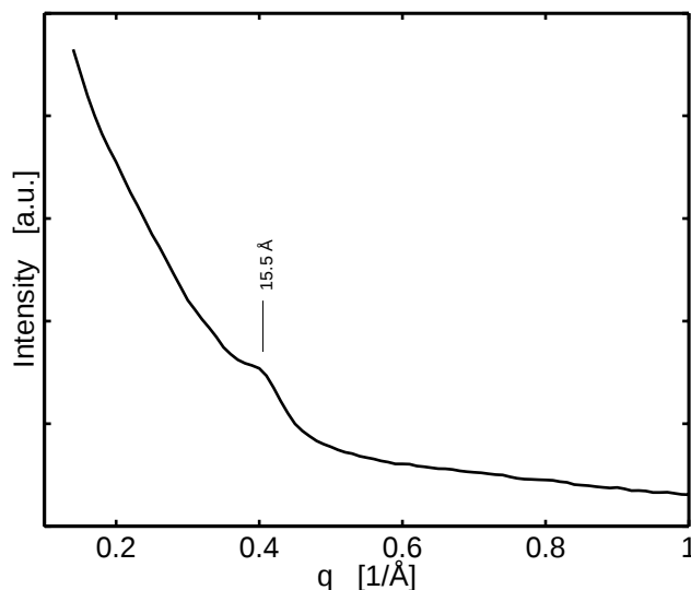
Figure 2 Scattering intensity of HFBI from the surface of a water droplet measured in the in-plane direction. The single reflection occurs at q = 0.405 Å -1 .
