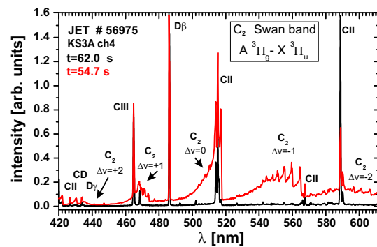
Figure 3: JET: Strong emission of C_2 in the corner region of the inner divertor.
