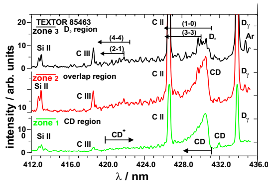
Figure 2: TEXTOR: Strong overlap of D_2 and CD lines during a D_2 gas blow.
