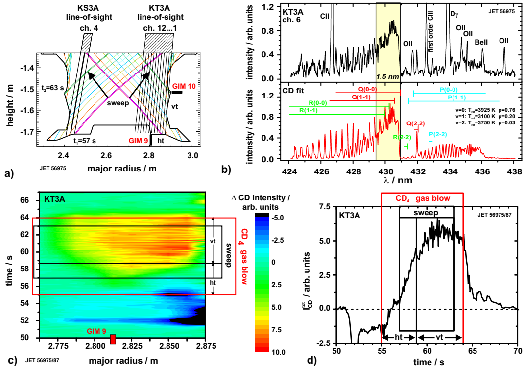
Figure 1: JET: a) Sketch of the JET divertor with the two observation systems marked. b) Spectra of the A-X transition of CD . c) Evolution of the CD intensity as function of the major radius during the CD_4 gas injection. d) Time evolution of the total CD intensity.
